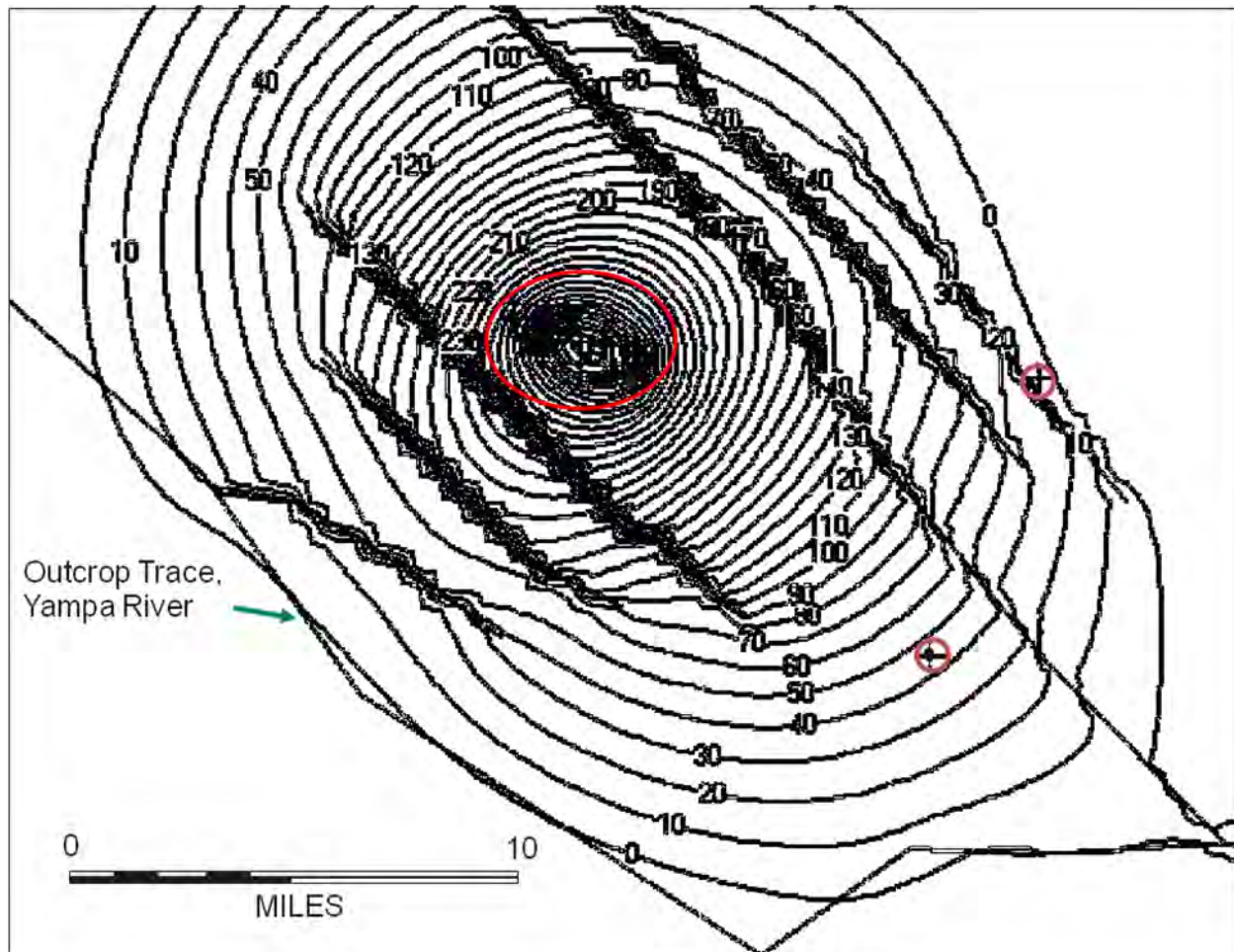
Figure 6.2. Steady-state Drawdown Plot for Encore Field With Mapped Fault Barriers. Drawdown contours drawn at a ten-foot interval center around the Encore wellfield with all wells pumping at rates calculated from monthly water production totals. Traces of mapped surface faults deflect contours and fragment the surface. Drawdown at the closest water well completed in the same stratigraphic interval is now about 45 feet. A well the same distance away, but across three fault barriers shows less than 5 feet of drawdown. Drawdown within the same block is enhanced while drawdown outside is reduced. The TWODAN® model uses general aquifer parameters and assumes a uniform and isotropic aquifer. Results should be considered qualitative.
