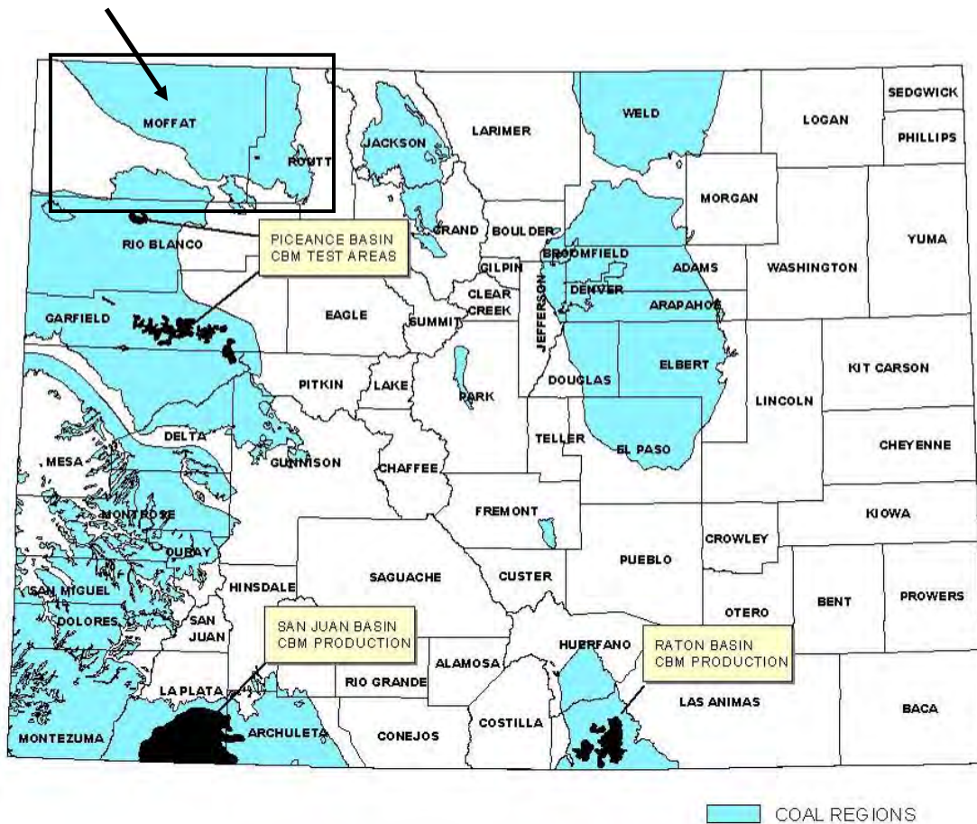
Figure 1.2 CBM Regions of Colorado. Sand Wash Basin, in the northwest corner of the state, is one of several coal regions in the State. Primary CBM production in the state is from the San Juan and Raton Basins along the southern border.
