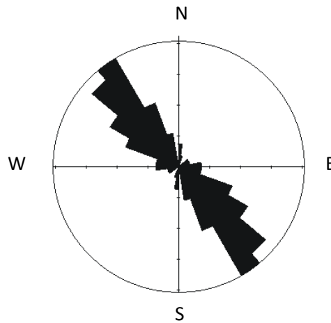
Fractures in brittle sandstone layers (54 measurements).
