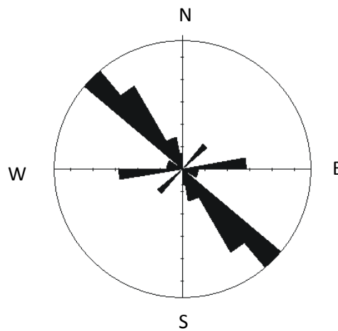
Coal seam face cleats (28 measurements).
