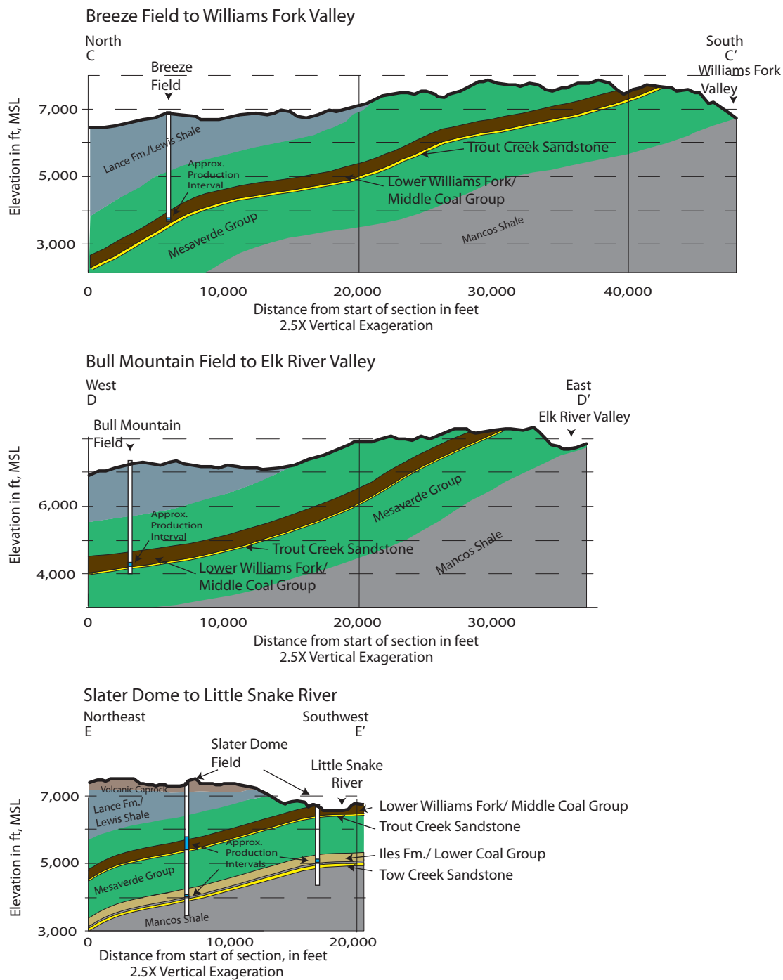
Figure 5.9 Cross-sections of Potential Connection from Slater Dome, Breeze, and Bull Mountain Fields to Surface Water Resources. Diagrammatic cross-sections show stratigraphic relationships and general structure between CBM production intervals at Breeze, Bull Mountain, and Slater Dome Fields and surface water resources. The Tow Creek and Trout Creek Sandstones underlie the coal-bearing intervals and are considered regional aquifers. Depths and stratigraphic thicknesses are approximate. See Figure 5.7 for cross-section alignments. Note that horizontal scale is larger than in Figure 5.8 for Encore Field. Sources: Tweto (1976), and CGS structural maps for BLM study.
