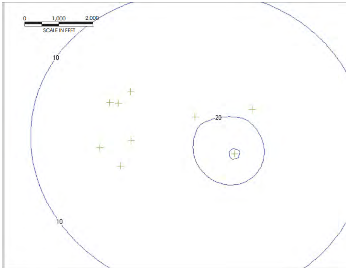
Figure 6.4. Steady-state Drawdown Plot for Section 20 with Wells Pumping at Appropriated Rates. Drawdown contours drawn at a ten-foot interval show combined interference around the close-spaced wells. Domestic well permits have a maximum allowed annual volume and rates calculated for those volumes are lower than reported yields. Contours now center around well with highest annual appropriation and drawdown in the area between wells is on the order of 10 to 25 feet. Note the difference in scale compared with the Encore scenario in Figures 6.1 and 6.2. The TWODAN® Model uses general aquifer parameters and assumes a uniform and isotropic aquifer. Results should be considered qualitative.
