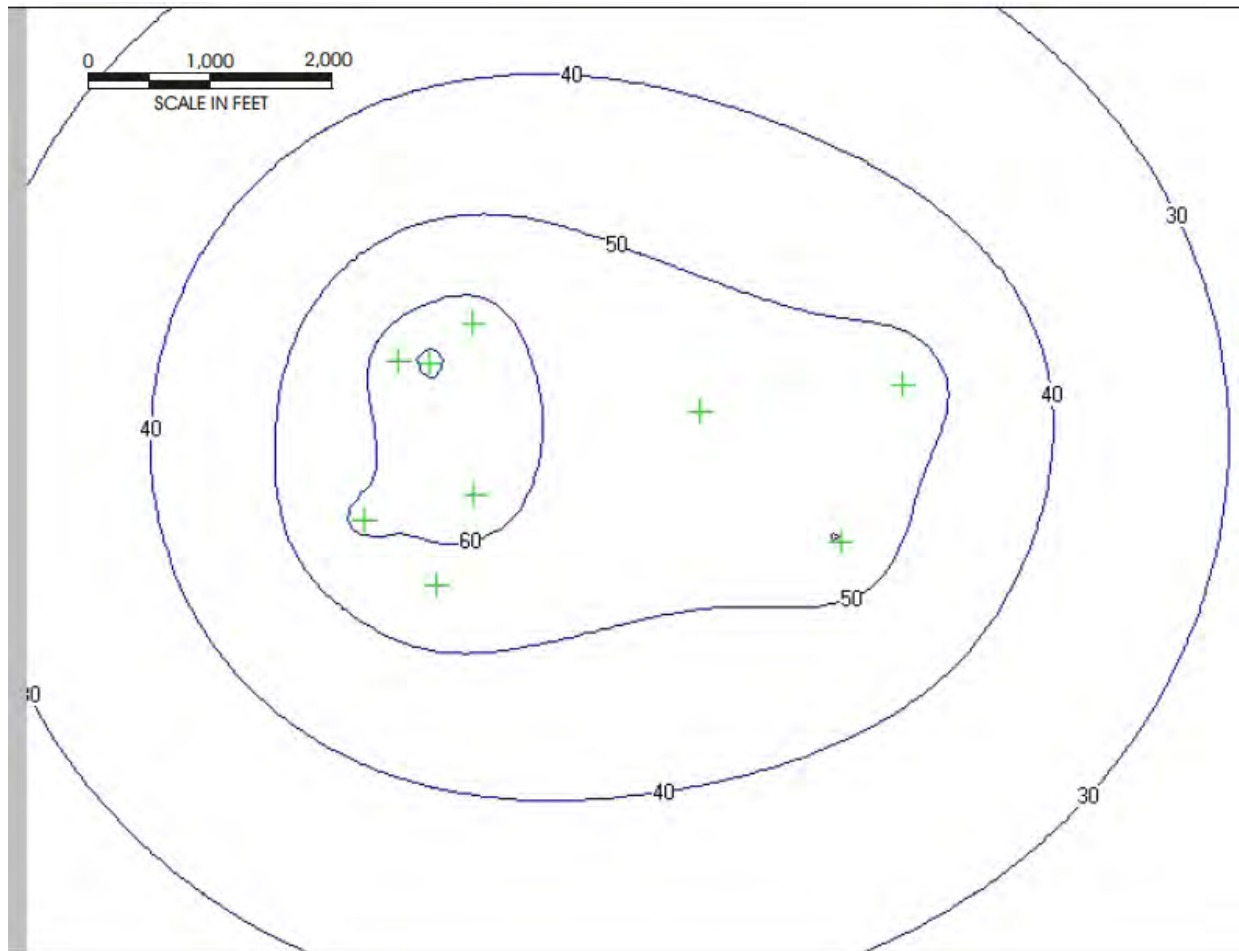
Figure 6.3. Steady-state Drawdown Plot for Section 20 with Wells Pumping at Reported Yields. Drawdown contours drawn at a ten-foot interval show combined interference around close-spaced domestic wells. Domestic well permits list yields based on short-term pump tests or simply listed permitted rate. Rates exceed rates based on annual appropriations and allow peak usage. Note the difference in scale compared with the Encore scenario in Figures 6.1 and 6.2. The TWODAN® model uses general aquifer parameters and assumes a uniform and isotropic aquifer. Results should be considered qualitative.
