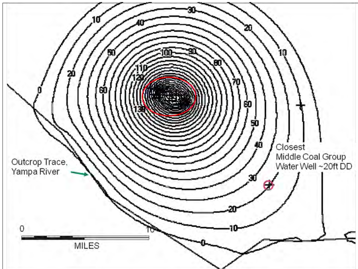
Figure 6.1. Steady-state Drawdown Plot for Encore Field without Fault Barriers. Drawdown contours drawn at a ten-foot interval center around the Encore wellfield with all wells pumping at rates calculated from monthly water production totals. Oval shape is driven by the outcrop trace constant head boundary. Drawdown at the closest water well completed in the same stratigraphic interval is about 20 feet. The TWODAN® model uses general aquifer parameters and assumes a uniform and isotropic aquifer. Results should be considered qualitative.
