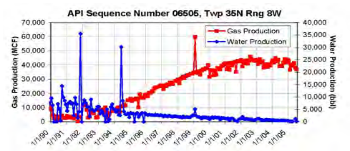
Figure 4.7 Gas-Water Production Plots for Two Sand Wash Basin CBM Wells. First graph shows declining gas production as water production holds steady or rises slightly at Encore Field. Second graph shows very scattered data with rising gas production and possible declining water production. Third graph shows a typical plot from the San Juan Basin. Source COGCC production data.
