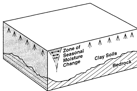
SWELLING SOILS
