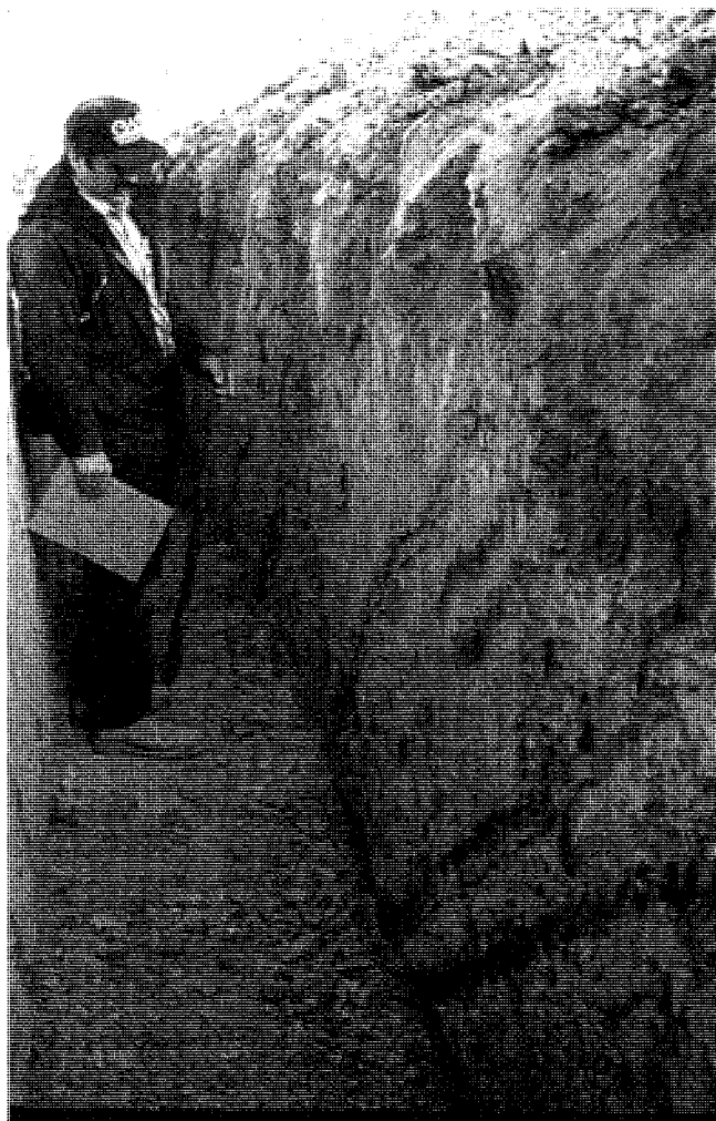
FIGURE 9: This trench has exposed dipping beds of bentonite (dark layers) at a high school site. Earlier drillhole surveys had not encountered the bentonite. The foundation design for the school was subsequently changed from a drilled-pier system to an overexcavation design.
