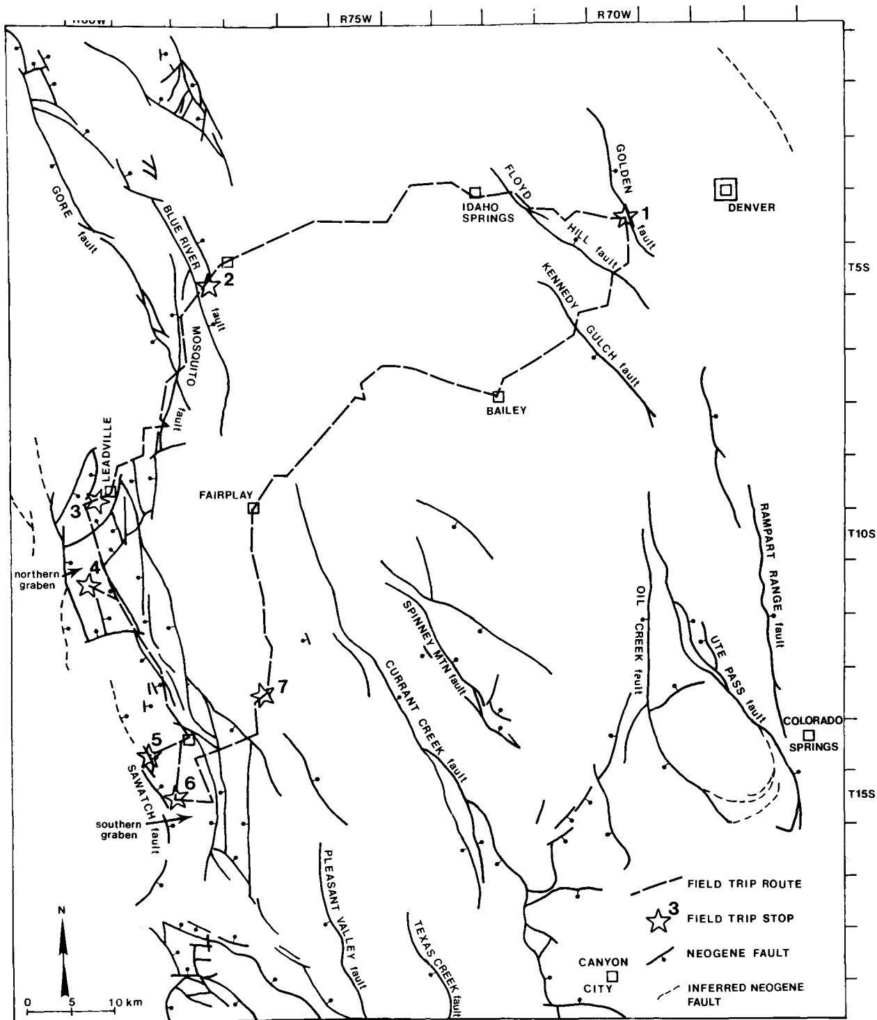
Figure 1. Late Cenozoic faults in central Colorado. (after Kirkham and Rogers, 1981).
