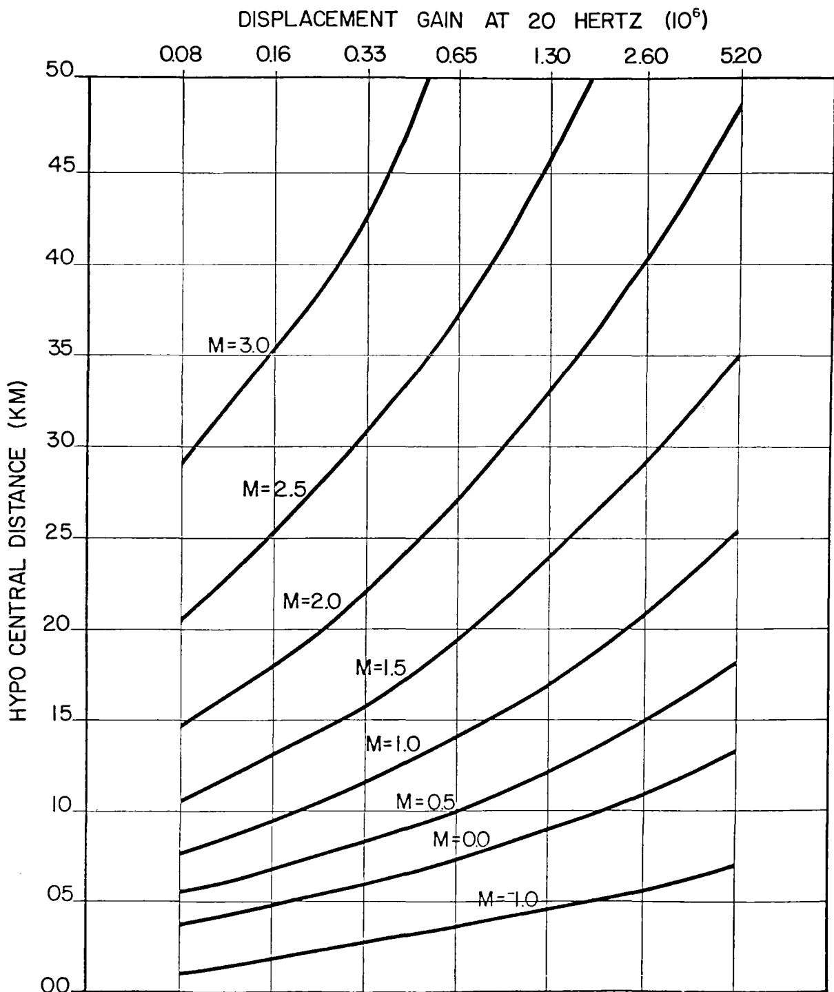
Figure 1: Detection Threshold Curves: Based on Richter with corrections for near field in Southern California by Brune and Allen, these curves denote the conditions of gain, magnitude and distance, for a 2mm pen displacement.
