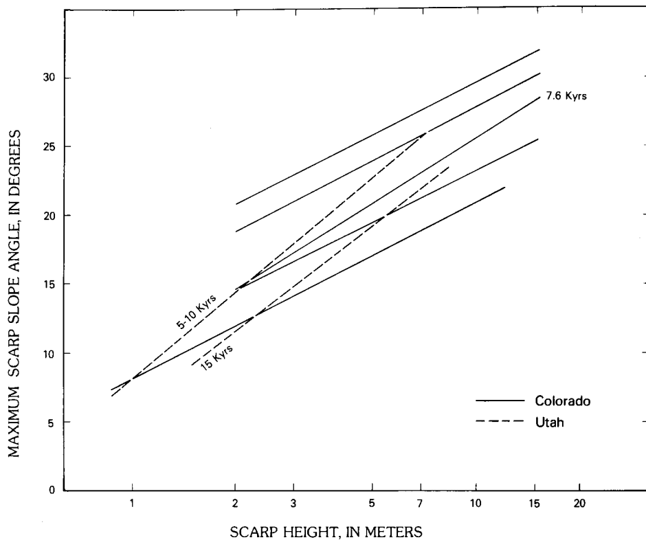
Figure 1.--Plots of maximum scarp angle against scarp height for selected scarps in Utah and in the Rio Grande Rift of Colorado. Utah data is from Bucknam and Anderson (1979). All scarps were formed or were last faulted between 5000 and 15000 years ago. More precise ages are given where known.
