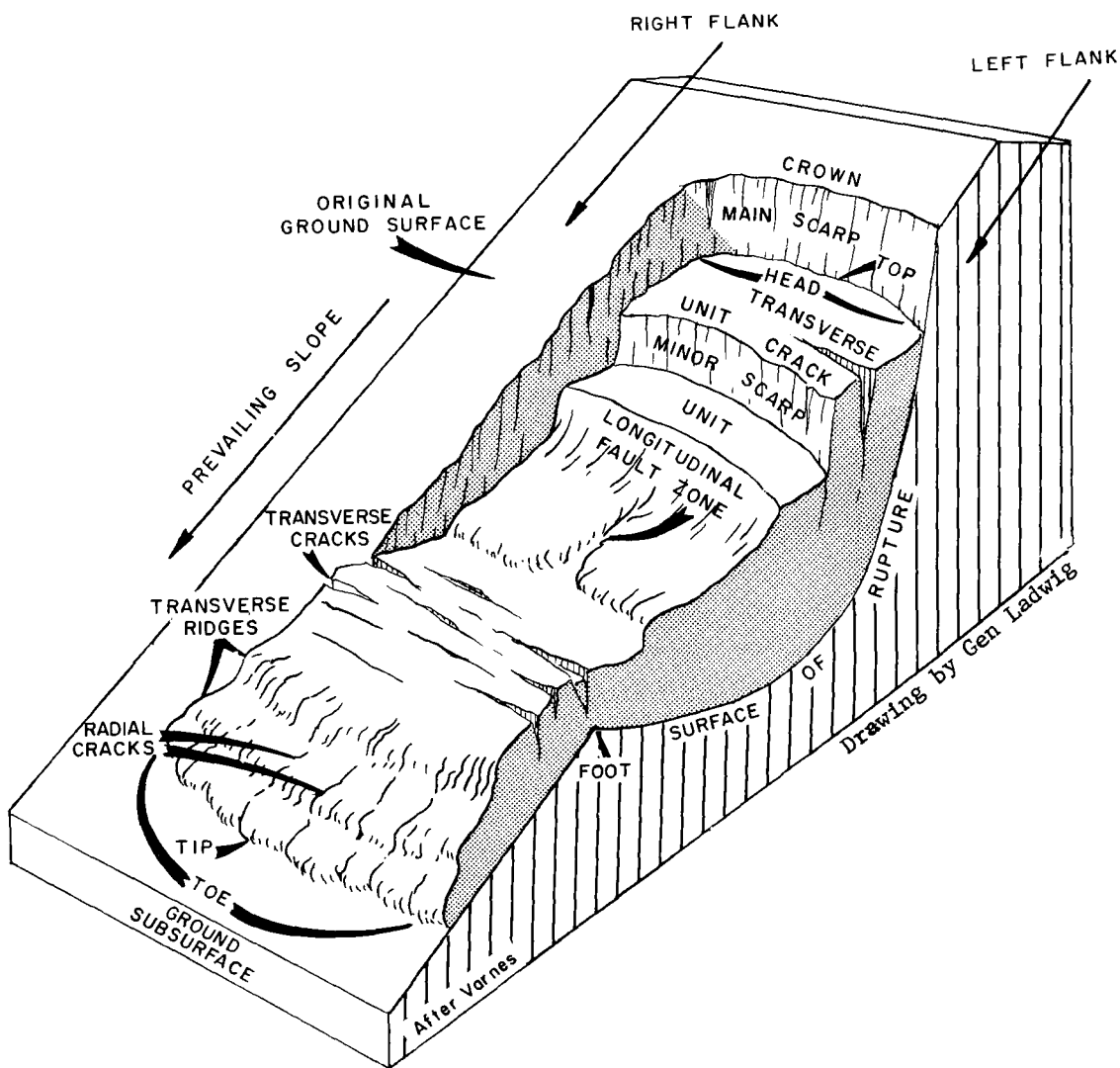
Figure 6. DIAGRAMMATIC DRAWING OF A ROTATIONAL LANDSLIDE
