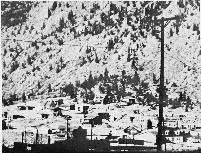
Figure 18. DEVELOPMENT ON A DEBRIS FAN (MOST OF THE DEBRIS FROM THE LATEST EPISODE OF DEPOSITION HAS BEEN REMOVED BY MAN). THE PROCESS OF DEBRIS DEPOSITION IS A RECURRENT EVENT AT MANY LOCATIONS.
