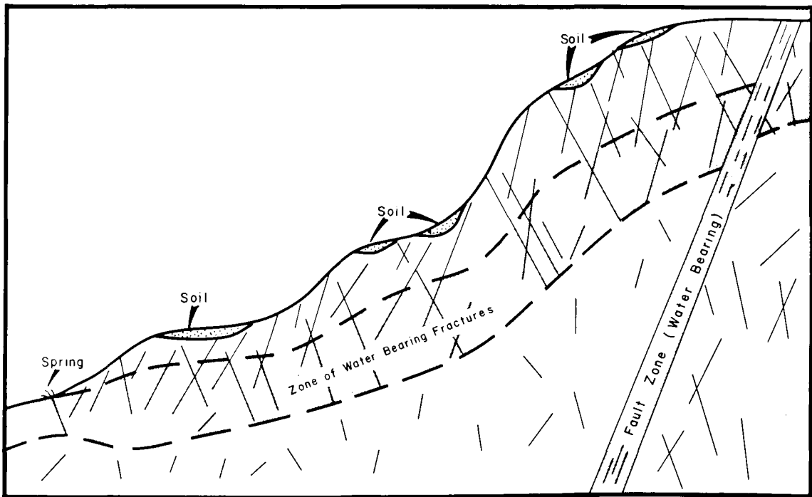
Figure 3. Diagrammatic cross section through a fractured crystalline bed rock aquifer system showing relationship between geologic conditions and occurrence of ground water.
