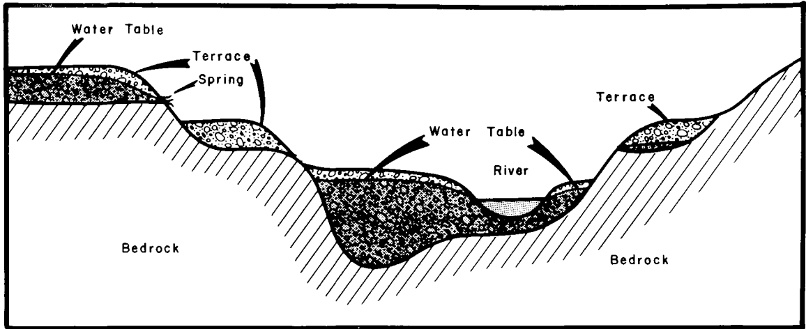
Figure 2. Diagrammatic cross section through an unconsolidated alluvial and terrace aquifer system found along most major rivers.
