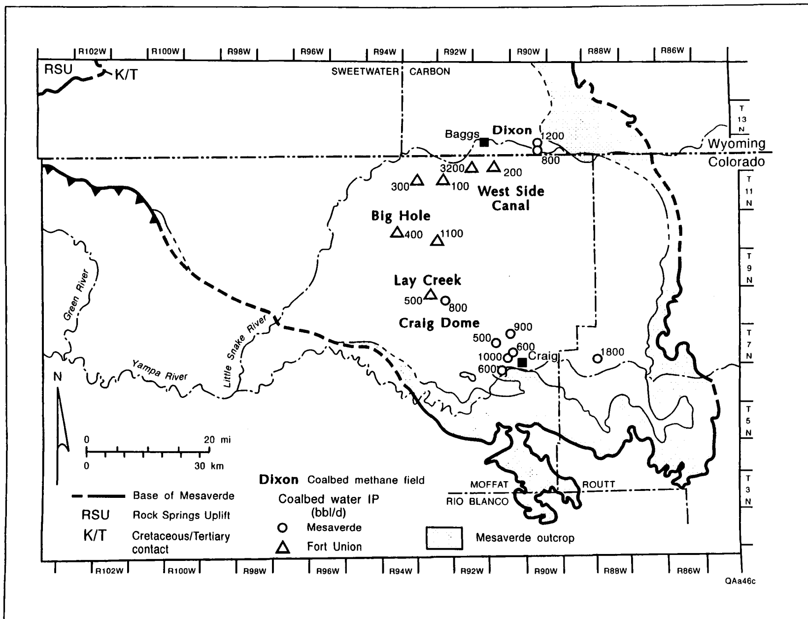
Figure 79. Initial water potentials, Williams Fork and Fort Union coals. Williams Fork IP's are high at the basin margin and reflect proximity to the recharge area and high coalbed permeability. Fort Union IP's are highest along the south-north trend of thick net coal.
