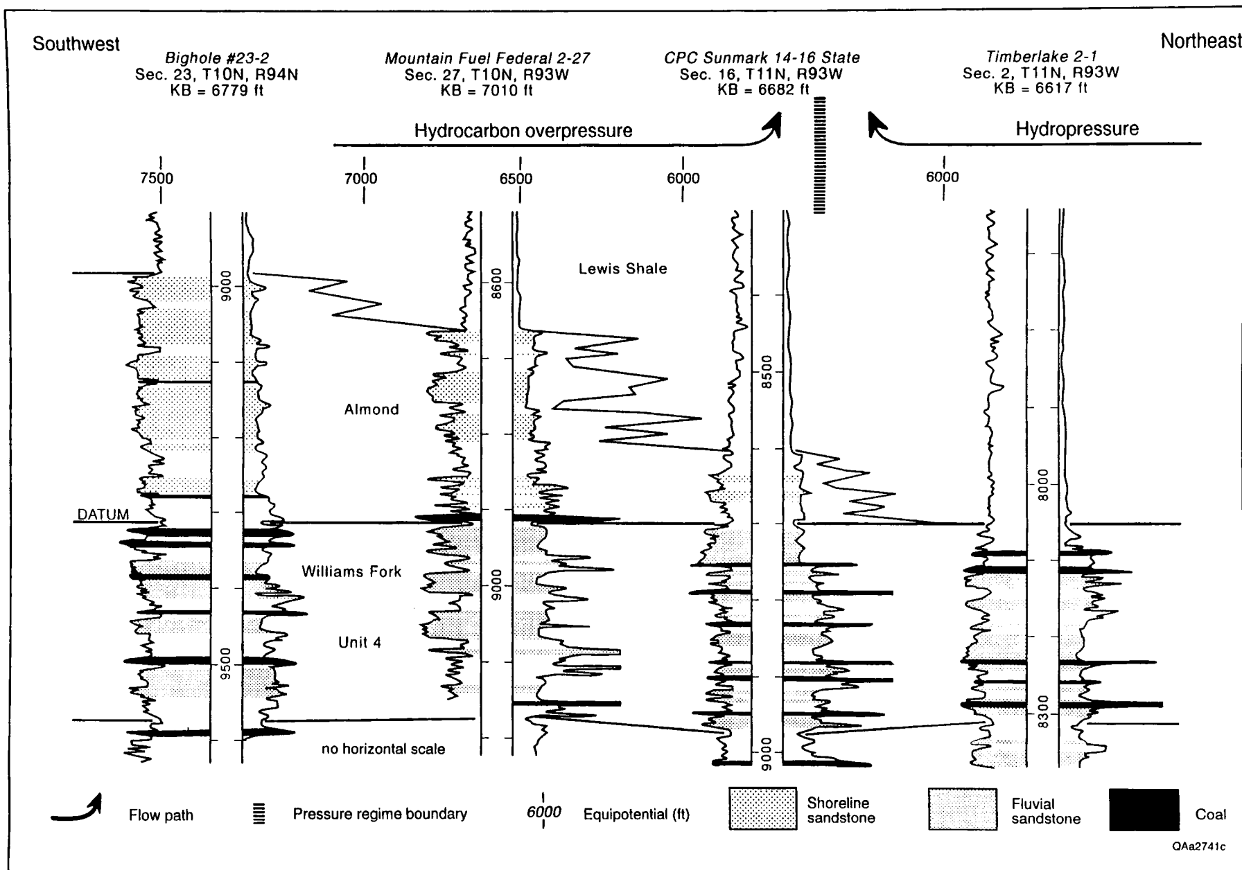
Figure 44. Southwest-northeast cross section across the geopressed-hydropressed transition zone. Pinch-out of Almond shoreline and fluvial sandstones in Unit 4 of the Williams Fork Formation correspond to the transition from geopressure to hydropressure. Location of section is shown in figure 40.
