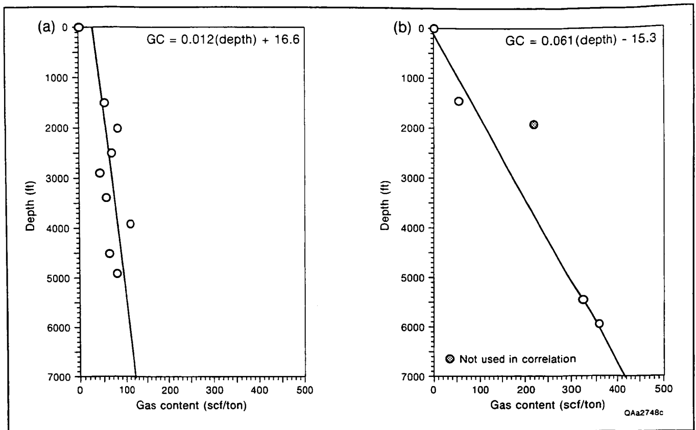
Figure 78. Gas content profiles and equations used for in-place gas and coal resource calculations. A moving average of 1,000 ft (305 m) intervals with 500 ft (153 m) overlap was used to determine a general relation between gas content and depth for the (a) Fort Union and (b) Williams Fork Formations.
