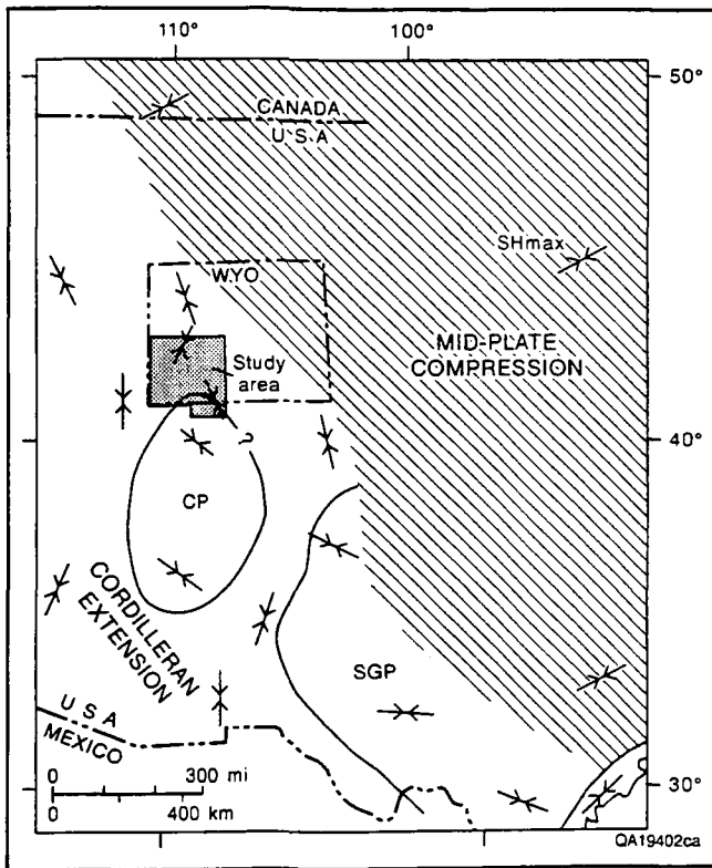
Figure 9. Stress province map showing major stress province boundaries in the vicinity of the Sand Wash Basin. Inward-pointing arrows indicate SHmax direction. CP = Colorado Plateau stress province; SGP = Southern Great Plains stress province. Study area is near the boundary between the Cordilleran extensional province and the midplate compressional province. Modified from Zoback and Zoback (1989).
