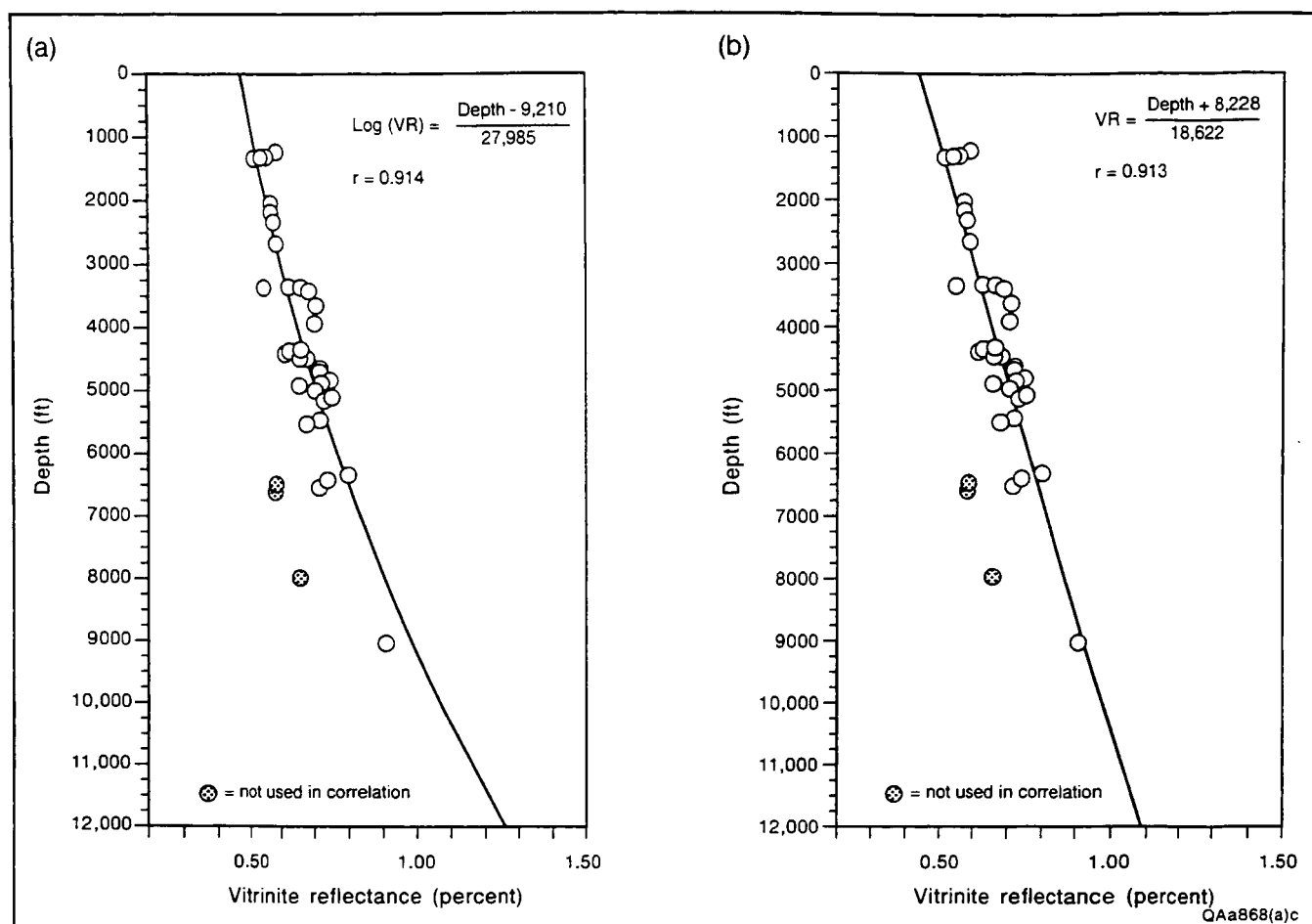
Figure 29. Vitritine reflectance profiles using depth versus vitritine reflectance for Mesaverde coals in the Sand Wash Basin. (a) Logarithmic regression analyses and (b) linear regression analyses. These equations were used to estimate the amount of overburden removal from the basin.
