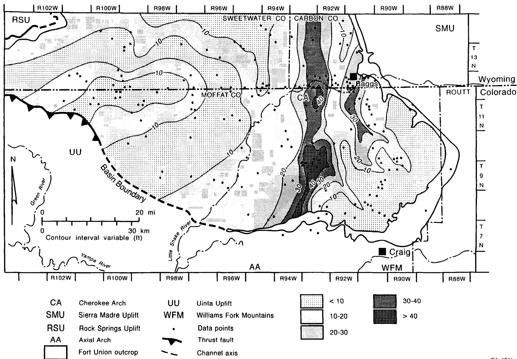
Figure 59. Maximum-coal-thickness map of the lower coal-bearing unit, Fort Union Formation, Sand Wash Basin. Thickest individual coal development (>40 ft [12.2 m]) occurs above and alongside a south-north-oriented fluvial system between R92W and R94W.
