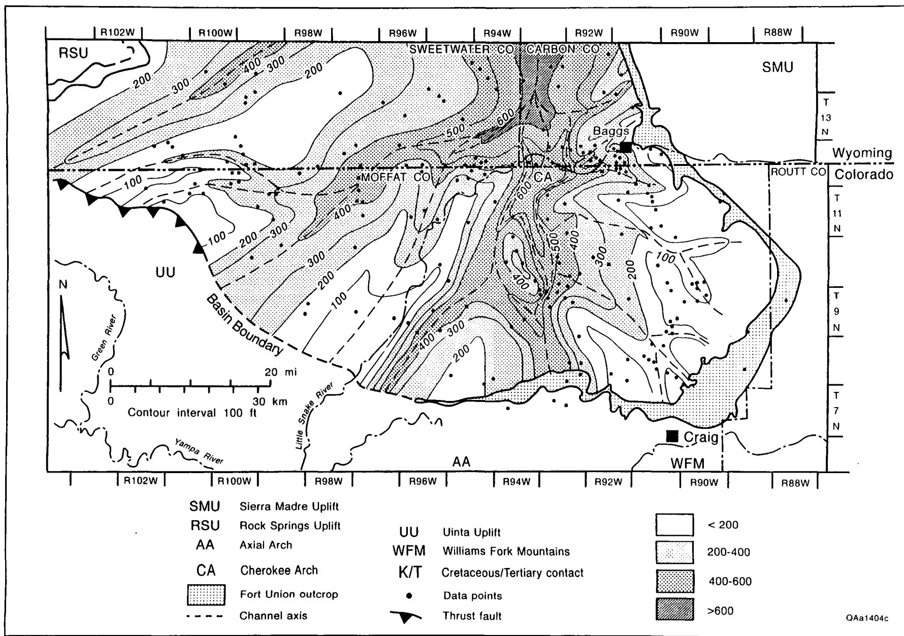
Figure 54. Net-sandstone-thickness map of the lower coal-bearing unit, Fort Union Formation, Sand Wash Basin. Thickest sandstone development (>600 ft [>182.8 m]) occurs along a south-north-oriented fluvial system between R92W and R94W. Smaller tributaries flow both east and west toward the depositional axis centered on R93W.
