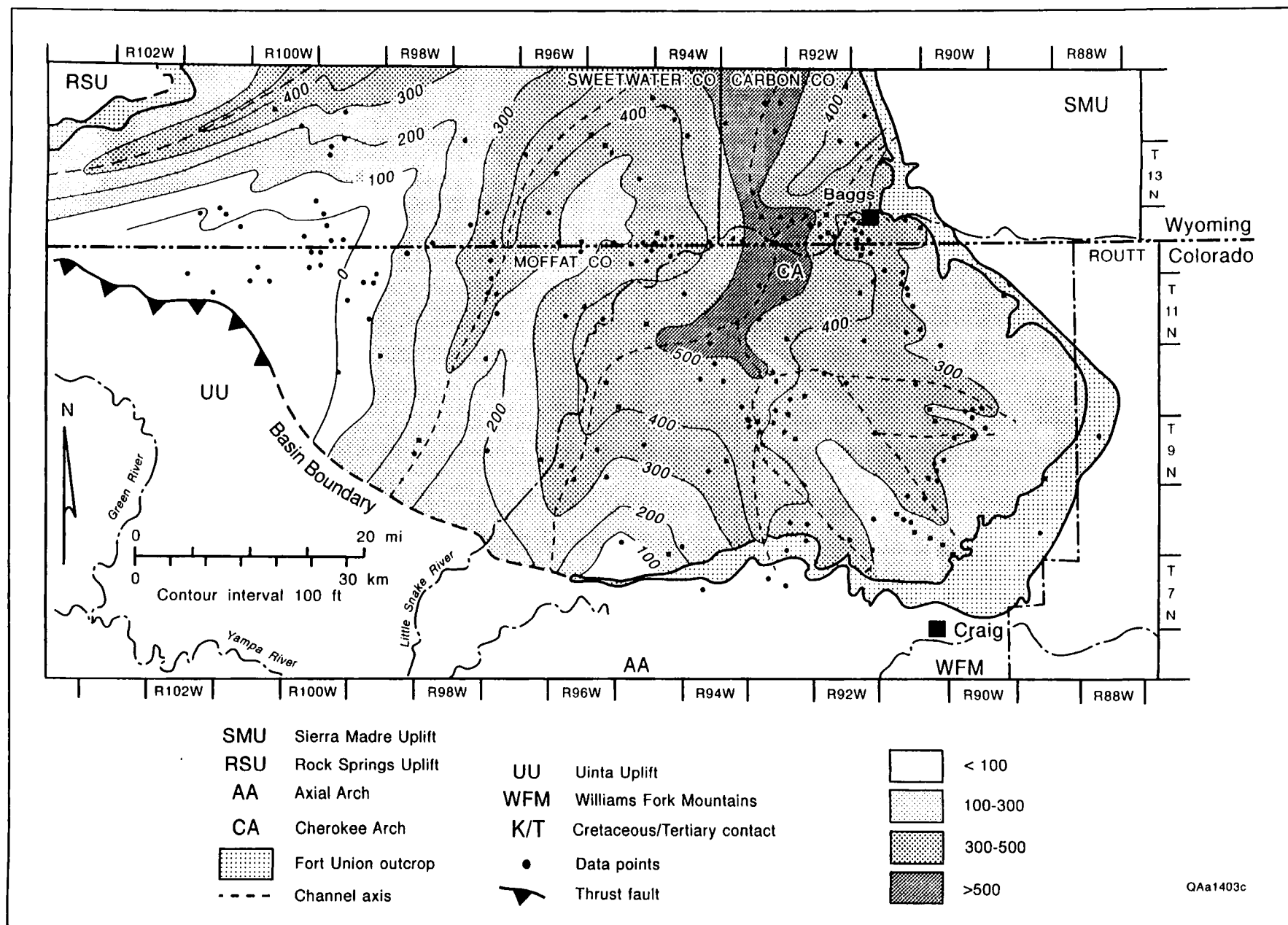
Figure 53. Net-sandstone-thickness map of the massive Cretaceous/Tertiary (K/T) sandstone unit, Sand Wash Basin. Thickest sandstone development (>500 ft [>152 m]) occurs along a south-north-oriented fluvial system between R92W and R94W.
