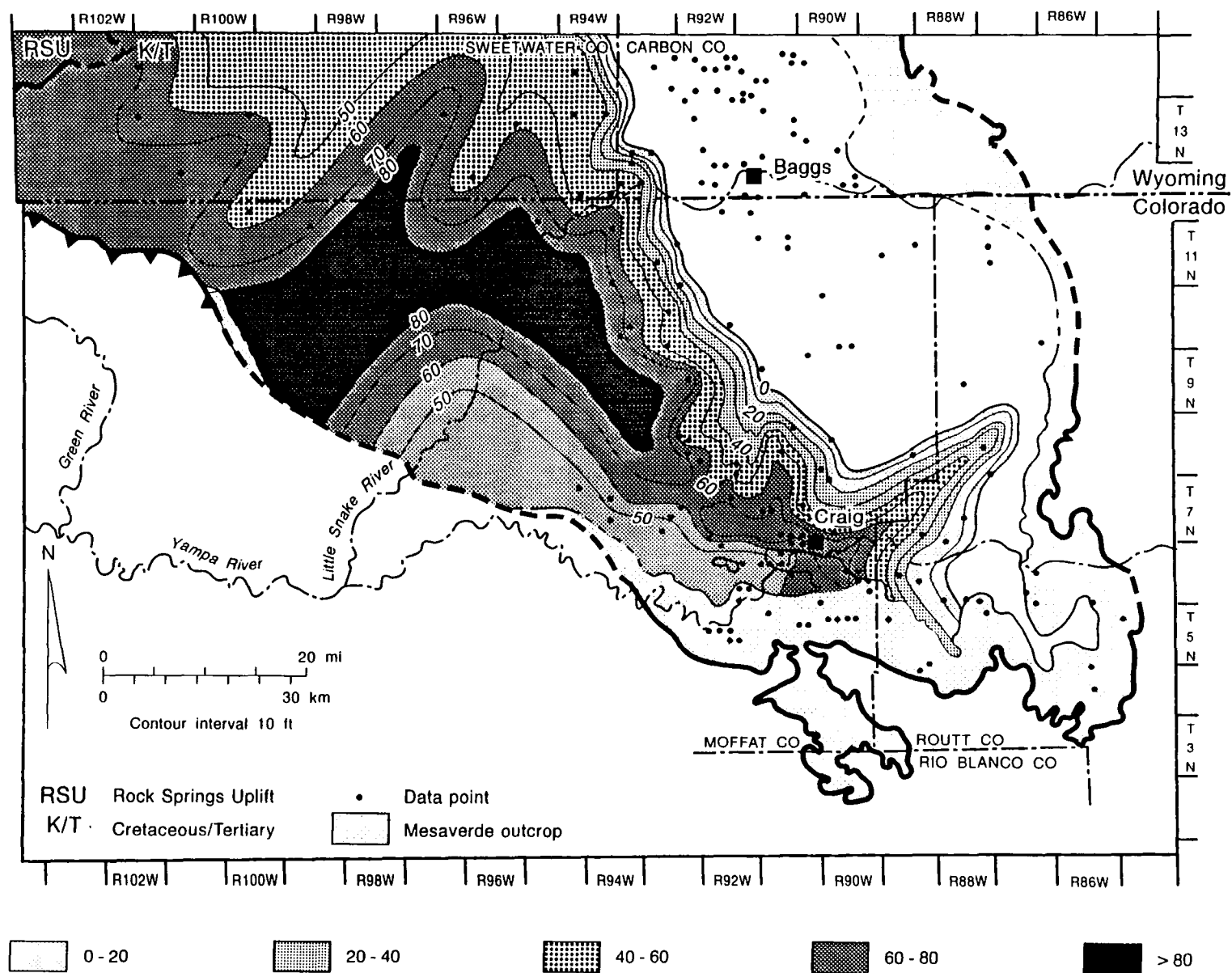
Figure 25. Percent-sandstone map of the Almond Formation. The map defines a strike-oriented strandplain system that extends between deltaic distributaries.
