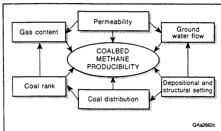
Figure 82. Interplay of geologic and hydrologic controls governs the producibility of coalbed methane.
