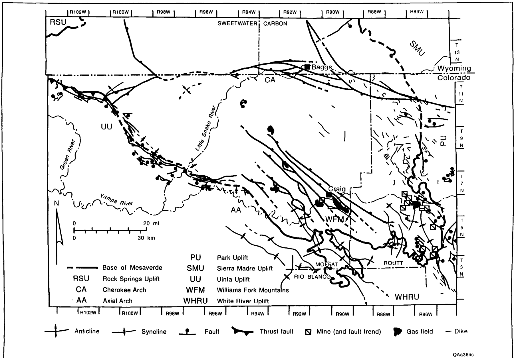
Figure 7. Map of tectonic elements in the Sand Wash Basin (modified from Hancock, 1925; Tweto, 1976a, 1979; Rowley and others, 1985). Locations of faults associated with coal mines and gas fields are shown. Note predominantly northwest trend of faults, folds, and dikes.
