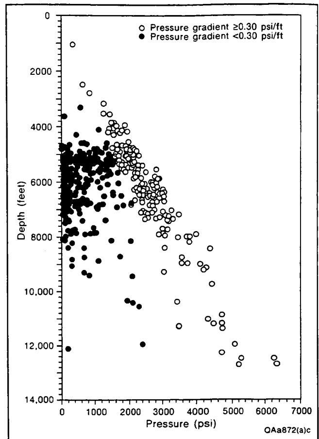
Figure 38. Depth versus pressure plot for Mesaverde DST data from the Sand Wash Basin. DST data with simple pressure gradients less than 0.30 psi/ft ( <6.8 kPa/m) were eliminated from the data base because of their uncertain validity.
