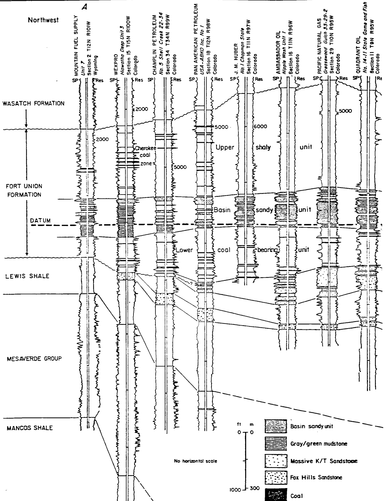
Figure 49. Northwest-southeast stratigraphic cross section A-A' of the Paleocene Fort Union Formation, Sand Wash Basin, illustrating operationally defined stratigraphic units and coal occurrence. Thick coal beds occur in the eastern Sand Wash Basin in the lower coal-
