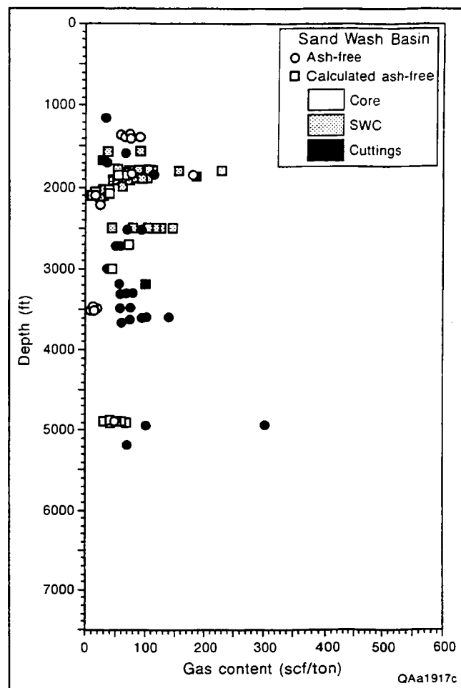
Figure 68. Gas content profile, Fort Union coals. The slightly higher gas content values at ~1,800 ft (~549 m) are from wells in T12N, R91W that correspond to an area of artesian overpressure.
