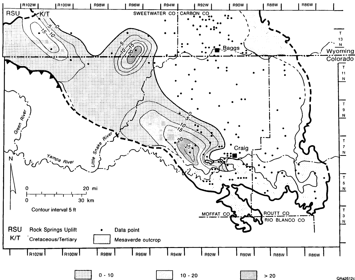
Figure 26. Net-coal-thickness map of the Almond Formation. Coals are distributed in three areas: (1) west of Craig, (2) southeast of the Rock Springs Uplift, and (3) west of the Sweetwater/Carbon county line.
