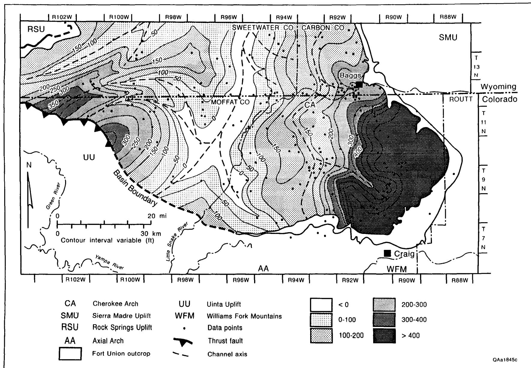
Figure 62. Net-mudstone-thickness map of the gray-green mudstone unit, Fort Union Formation, Sand Wash Basin. Thickest mudstone development (>400 ft [>121.9 m]) occurs east of the south-north-oriented fluvial system between R92W and R94W, adjacent to the Sierra Madre-Park Uplift. Structural and depositional axes have migrated to the west (R96).
