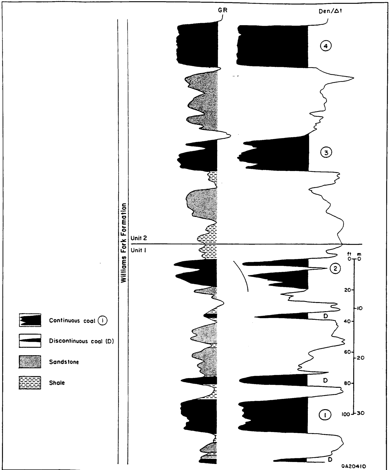
Figure 14. Density profile of typical Williams Fork coals. Coal seams can have a unique profile, or signature, owing to variations in their lithotypes. The lithotypes are a function of the original peat-forming plants and the physical and chemical conditions of the peatswamp. Gamma-ray and density logs are sensitive to minor fluctuations in coal seam lithotypes and thus provide a tool for correlation.
