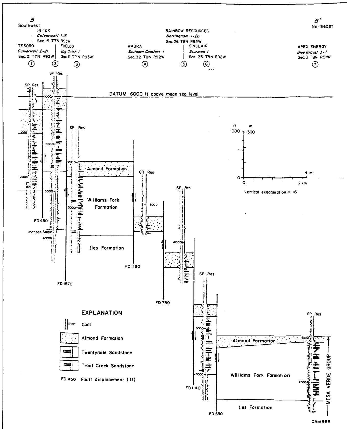
Figure 8. Structural cross section through the Cedar Mountain fault system, drawn on the Mesaverde Group, Sand Wash Basin. Fault blocks downthrown to northeast. Throws range from 500 to 1,500 ft (152 to 457 m). Total displacement across the system is about 5,000 ft (~1,524 m).
