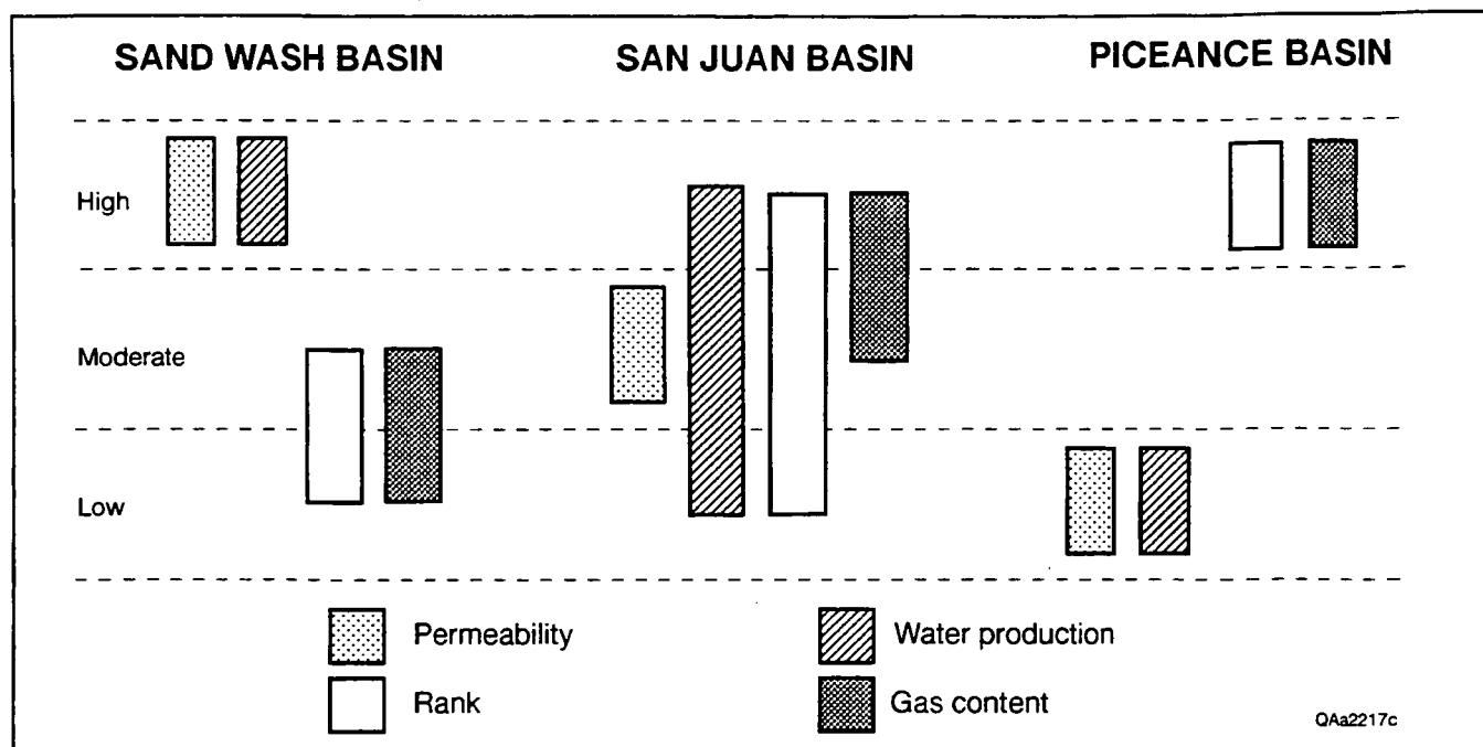
Figure 83. Characteristics of key geologic and hydrologic controls overlap in western coal basins.
