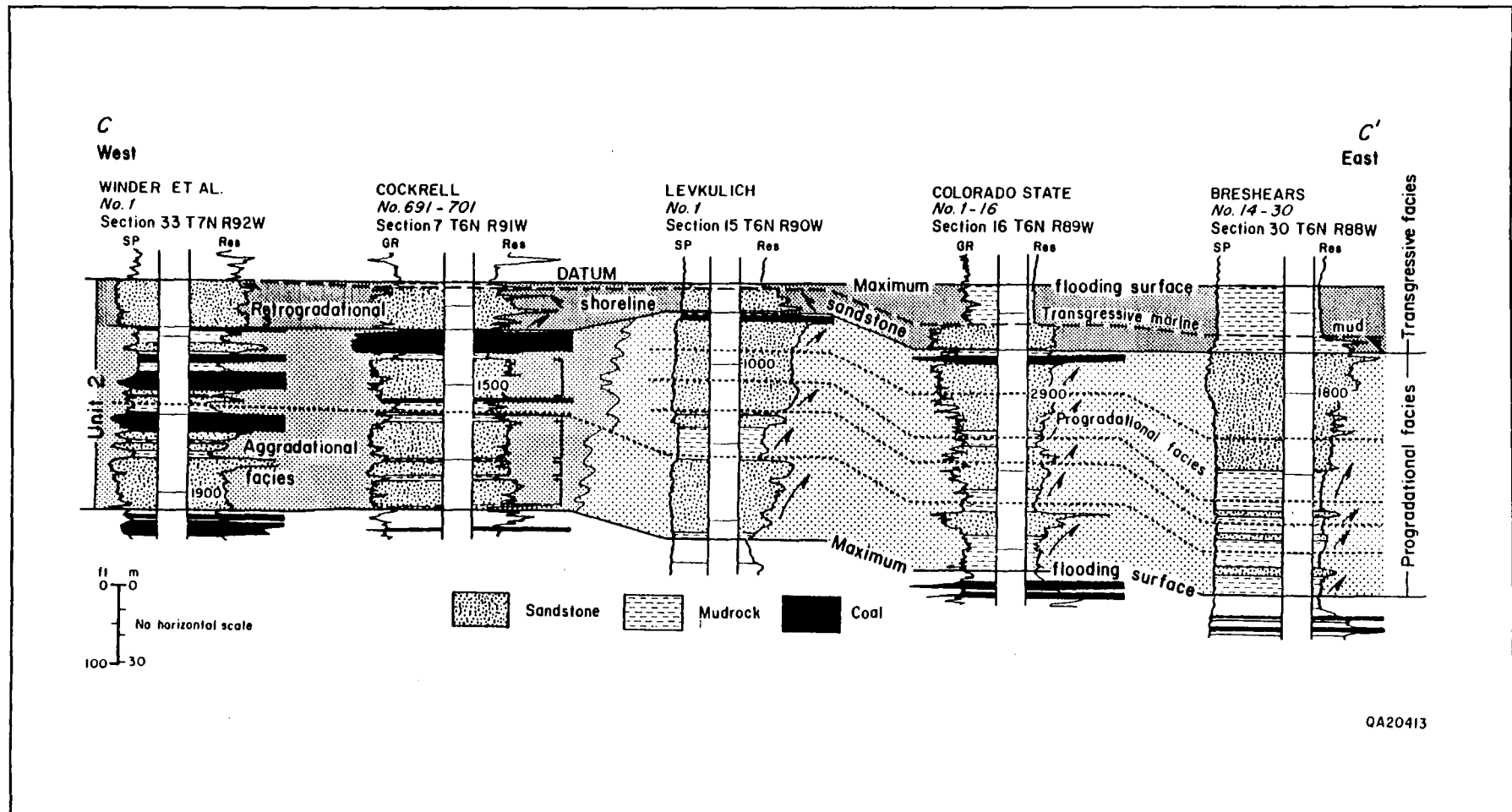
Figure 20. Cross section of the Unit 2 coal. Peat accumulated on an aggrading coastal plain behind the progradational shoreline facies. Coals override the shoreline sandstones to achieve great lateral extent.
