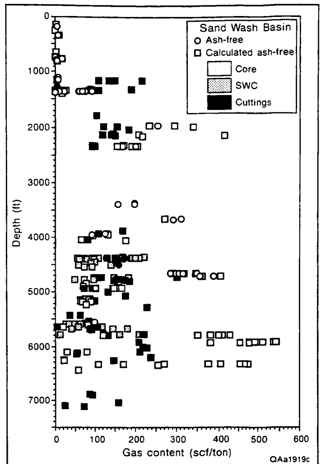
Figure 32. Gas content profile for the Sand Wash Basin Mesaverde coals. Gas content increases with depth, as in other western coal basins. At any particular depth, there is a wide range of gas content values. Sidewall cores and cuttings generally have lower gas contents than whole cores, indicating that sampling and handling procedures influence gas content measurements. Data are ash-free values calculated from average ash contents of adjacent seams.
