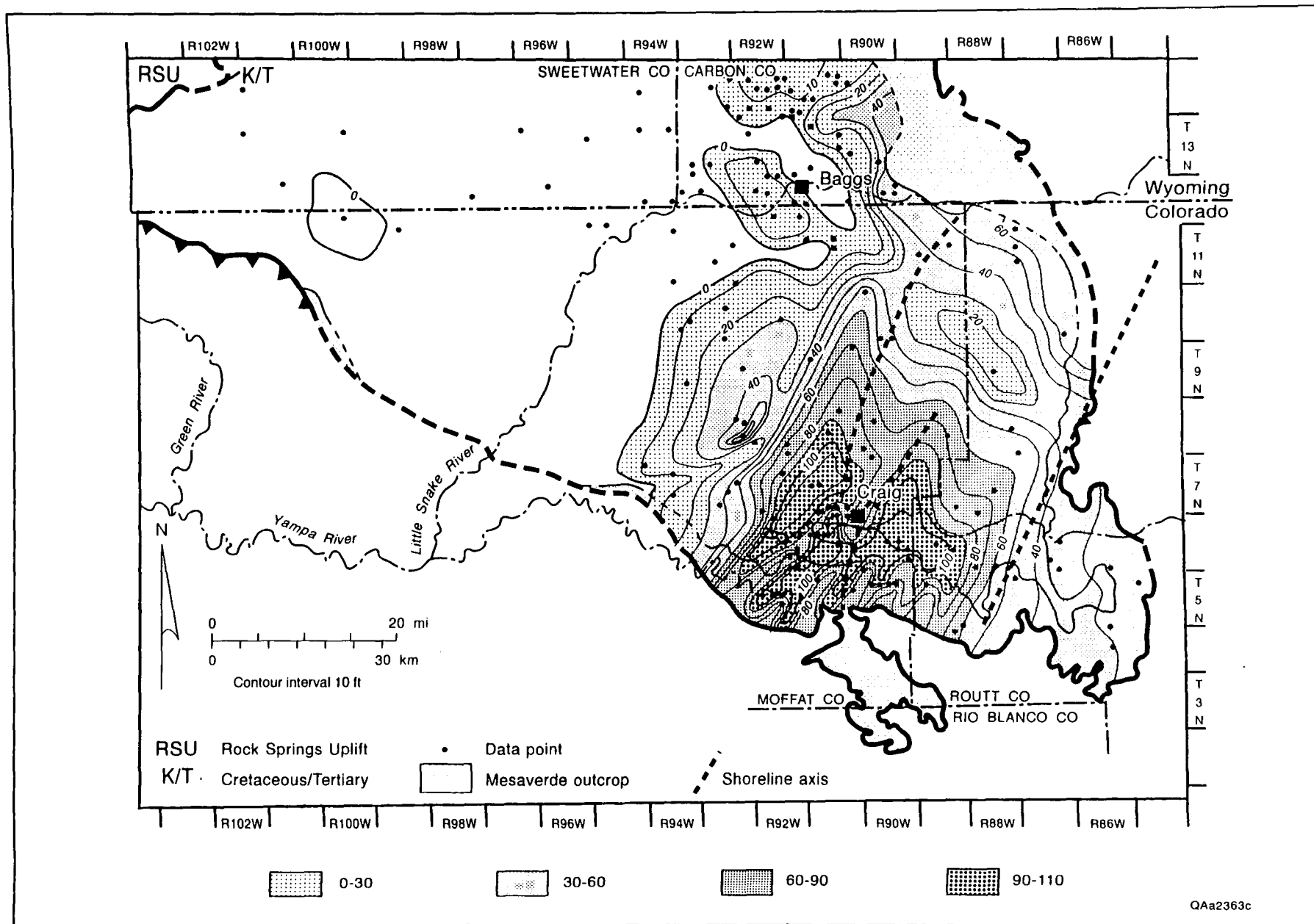
Figure 16. Net-coal-thickness map of Unit 1, Williams Fork Formation. Thickest net coal occurs in the Craig area, where peat accumulated on the coastal plain behind the linear shoreline systems. Coals thin to the west at the coastal-alluvial plain transition. Coal is also thin along a dip-oriented (northwest-southeast) distributary system extending southeastward from Baggs.
