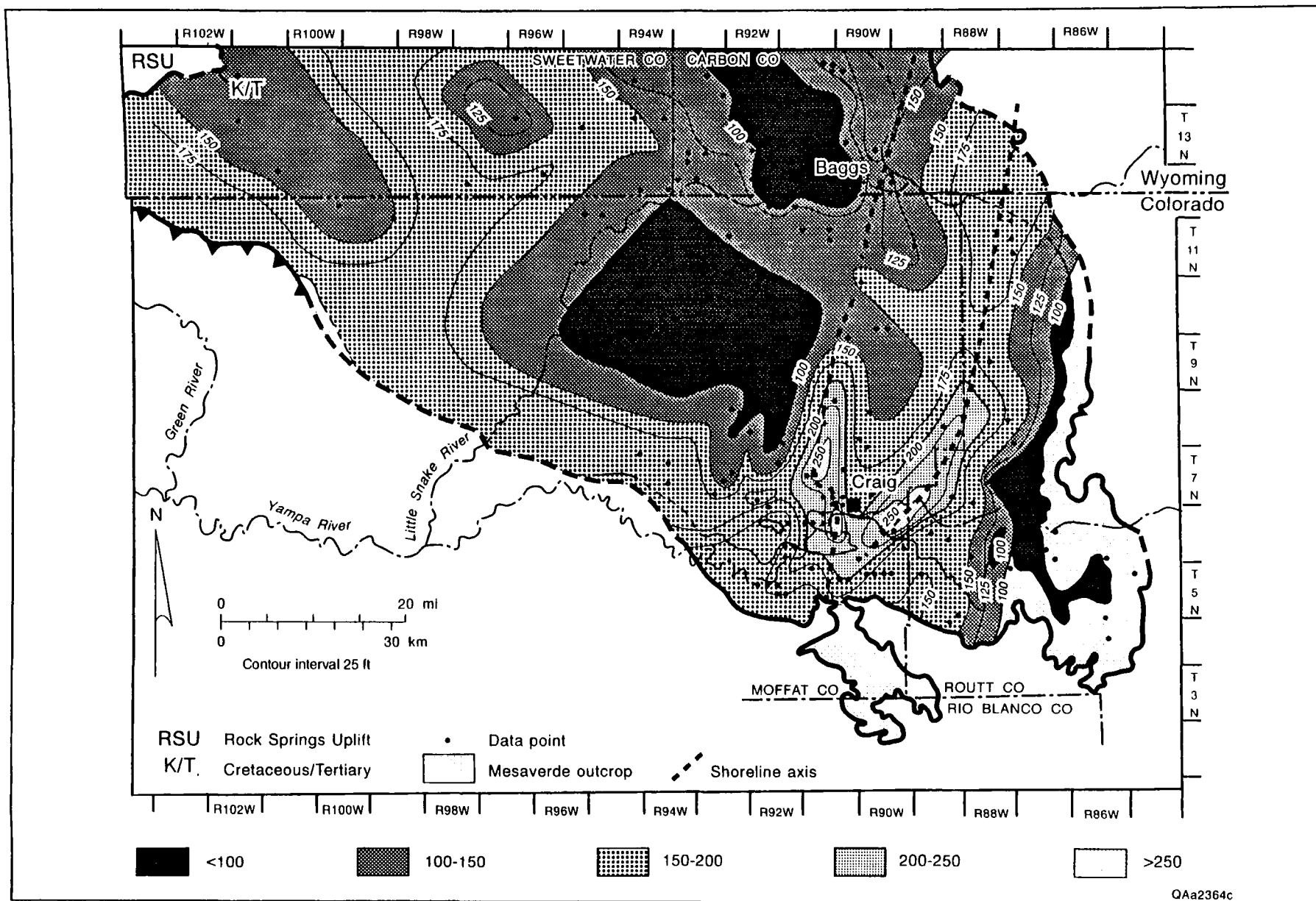
Figure 17. Net-sandstone map of Unit 2, Williams Fork Formation. Two subparallel, strike-oriented sandstone-rich trends define the shoreline system that is backed landward by a coastal plain system (net sandstone less than 150 ft [ <46 m]), which grades westward into the alluvial plain. The sand-poor trend crosscutting the seawardmost shoreline is interpreted as a tidal-inlet complex. The sandstone-rich trend crosscutting the coastal plain represents a distributary channel complex.
