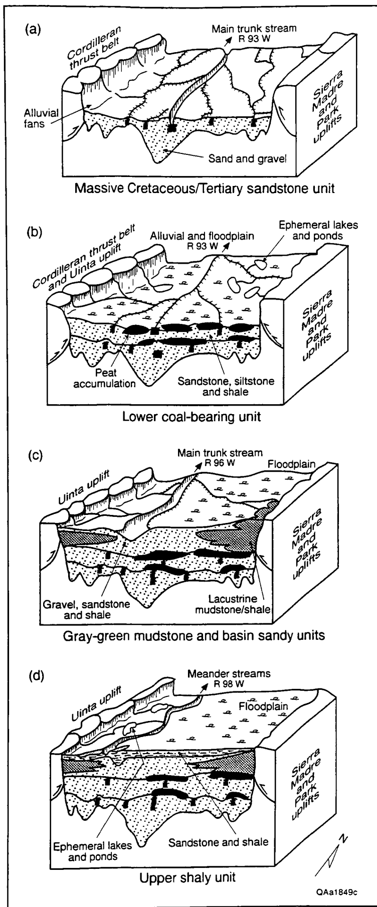
Figure 64. Block diagrams showing the stratigraphic development of the Fort Union Formation, Sand Wash Basin. (a-d) Valley aggradation stages 1-4: (a) Maximum massive K/T sandstone development occurs along a south-north-oriented fluvial system centered on R93W. (b) Lower coal-bearing unit: maximum sandstone development occurs along a south-north-oriented fluvial system; maximum coal development occurs above and alongside the fluvial system as floodplain deposits. (c) Gray-green mudstone and basin sandy units: maximum mudstone/shale development occurs in the eastern and western Sand Wash Basin as floodplain and lacustrine deposits; maximum sandstone development occurs along a south-north-oriented fluvial system centered on R96W. (d) Upper shaly unit: maximum sandstone development occurs in the western Sand Wash Basin; the eastern Sand Wash Basin is predominantly made up of shaly floodplain and lacustrine deposits. Modified from Beaumont (1979).
