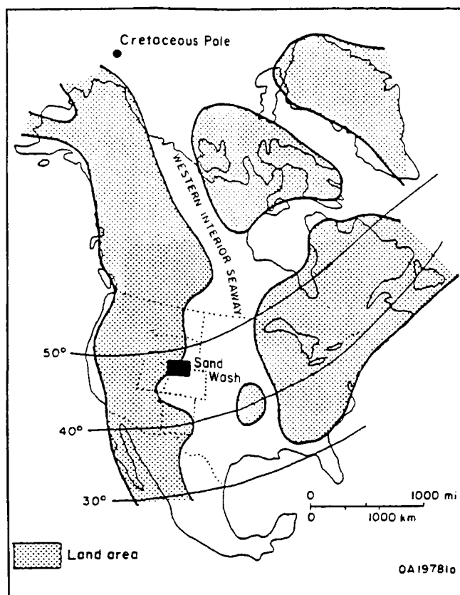
Figure 3. Location of the Sand Wash Basin relative to the Western Interior Seaway. Modified from Kauffman (1977).
