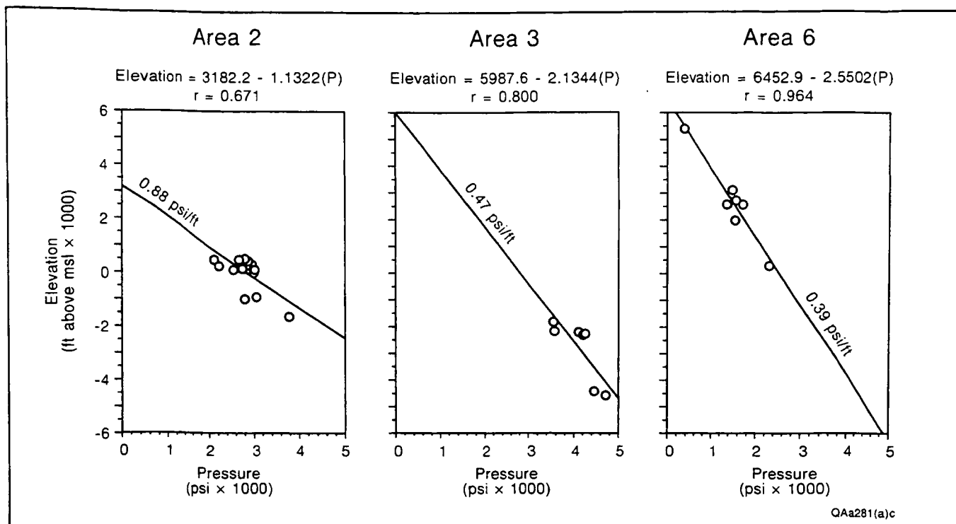
Figure 42. Mesaverde pressure-elevation plots for pressure-analysis, Areas 2, 3, and 6. The large vertical-pressure gradient in Area 2 (~0.88 psi/ft [~19.9 kPa/m]) indicates a strong potential for upward flow and poor vertical connectivity (good confinement), whereas Areas 3 and 6 indicate weak upward and moderate downward-flow potentials, respectively. Downward flow in Area 6 may reflect flow down steep structural dip (Tyler and Tremain, this vol., fig. 5).
