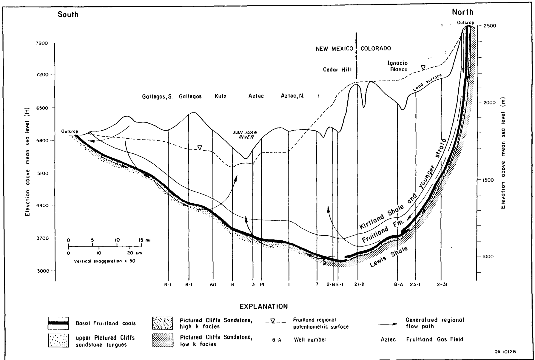
Figure 85. Schematic cross-sectional ground-water flow, San Juan Basin (modified from Kaiser and others, 1991b). Flow is down the steep northern limb from high to lower rank coal. Flow turns steeply upward in the vicinity of Cedar Hill field, upon pinch-out of thick coal beds and/or their offset by faults, along a structural hingeline. Free gas and solution gas, conventionally trapped and concentrated at a no-flow boundary, and high permeability combine for prolific production at this point in the basin.
