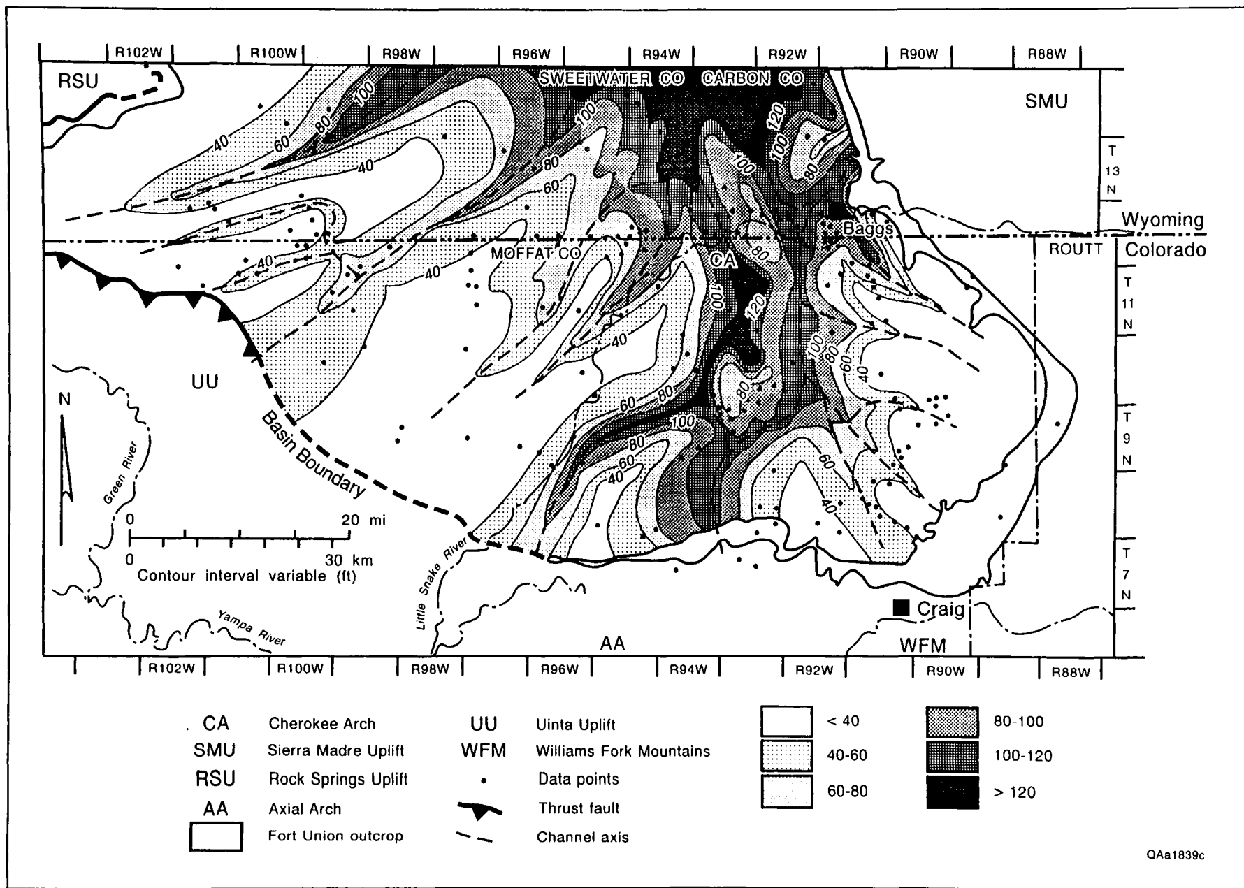
Figure 56. Maximum-sandstone-thickness map of the lower coal-bearing unit, Fort Union Formation, Sand Wash Basin. Thickest individual sandstone development (>120 ft [>36.6 m]) occurs along a south-north-oriented fluvial system between R92W and R94W.
