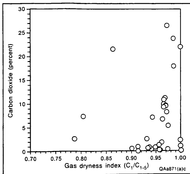
Figure 37. Variation of carbon dioxide content with the gas dryness index ( C_1/C_{1.5} values). Coals with the higher carbon dioxide content generally have very dry gases, although coals in the Morgan Federal 12-12 and Colorado State 1-31 wells have wet gases.
