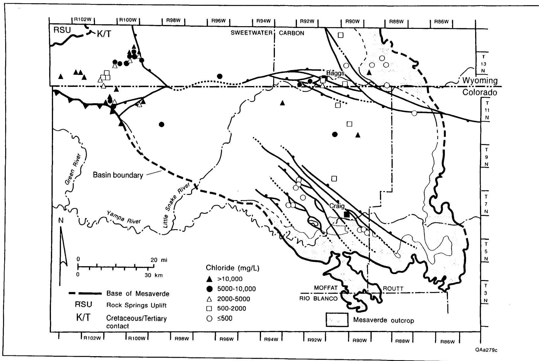
Figure 46. Mesaverde chlorinity map. Chlorinity of formation waters ranges from less than 100 mg/L east of Baggs to generally more than 10,000 mg/L in the western part of the basin. The chlorinity gradient shows that ground water flows westward and northwestward from the eastern and southern margins of the basin, respectively.
