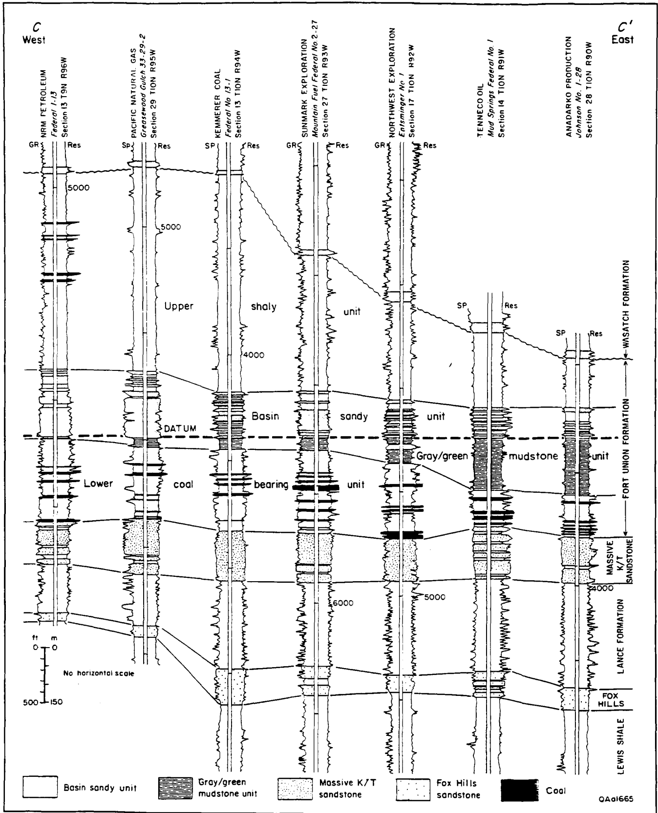
Figure 51. West-east stratigraphic cross section C-C' through T10N of the Paleocene Fort Union Formation, Sand Wash Basin, illustrating operationally defined stratigraphic units and coal occurrence of the lower coal-bearing unit. Thickest and more continuous coal beds occur in the eastern Sand Wash Basin above thickest sandstone development.
