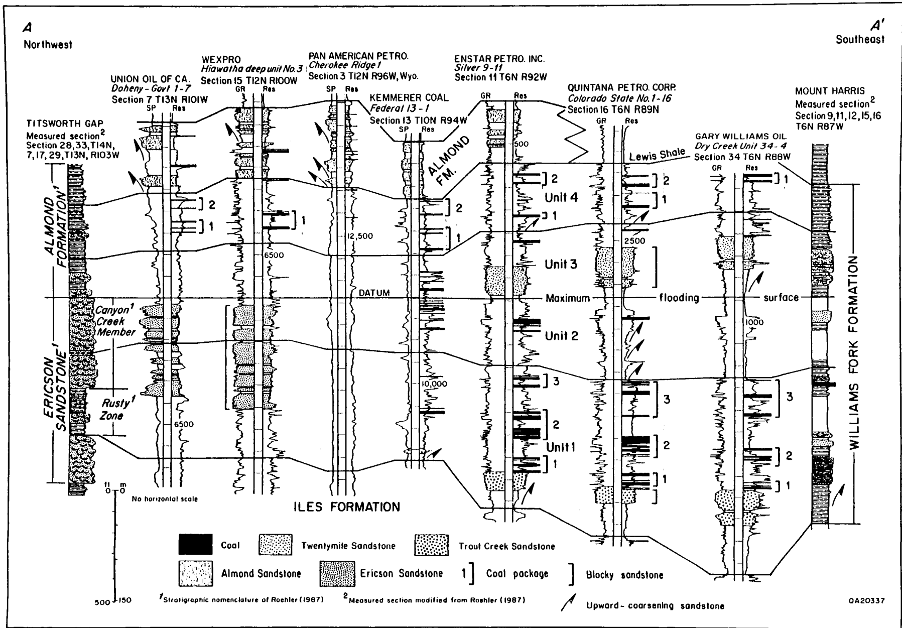
Figure 12. Northwest-southeast cross section of the upper Mesaverde Group, Sand Wash Basin, illustrating genetic stratigraphy of the Williams Fork Formation and coal occurrence. Unit 1 and 2 coals are lost westward of the transition to alluvial Ericson Sandstone at the basin's structural center.
