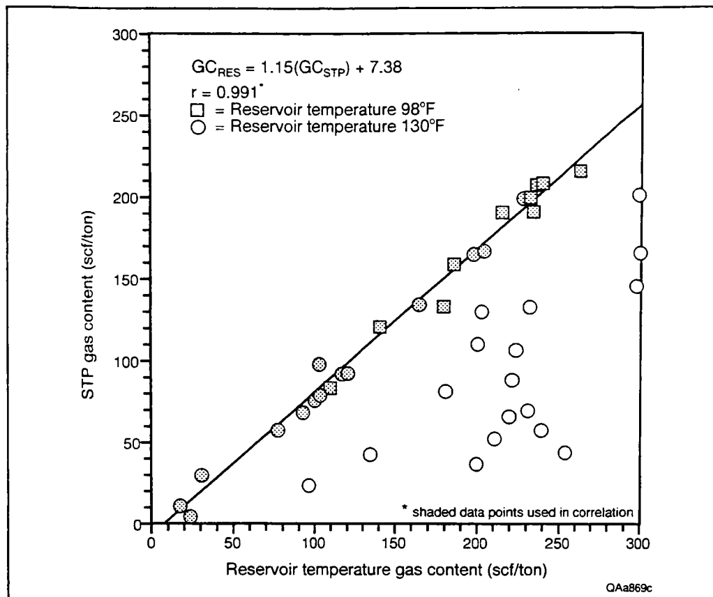
Figure 33. Relation between gas contents determined at room (STP conditions) and reservoir temperatures.
