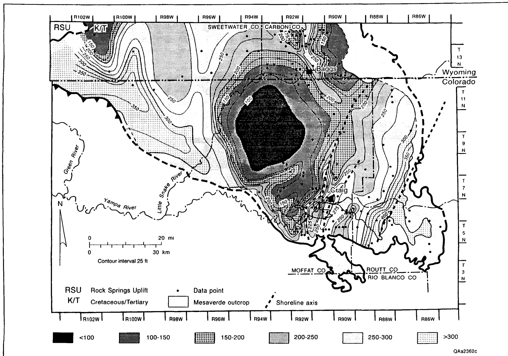
Figure 15. Net-sandstone map of Unit 1, Williams Fork Formation. A number of strike-oriented (northeast-southwest) linear clastic shorelines are evident, backed landward by a coastal plain system (net sandstone less than 125 ft [ <38 m]), which grades westward into a large fluvial system (Ericson Sandstone). A dip-oriented distributary channel system extends southeastward from Baggs.
