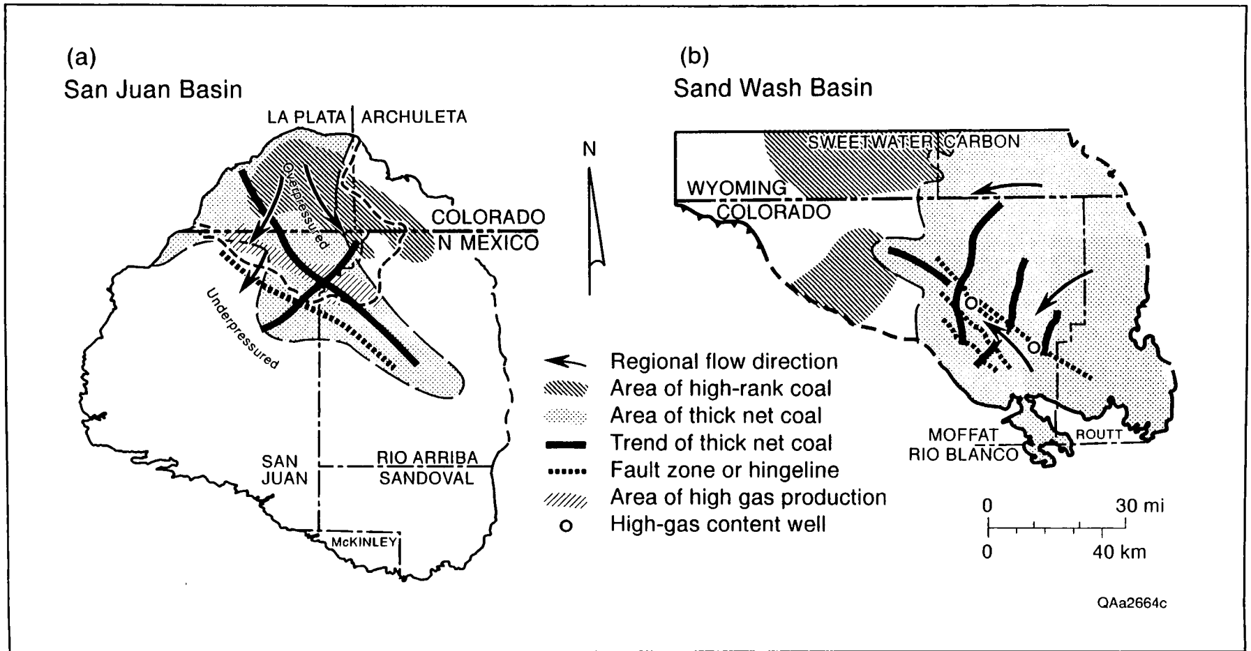
Figure 84. Geologic and hydrologic comparison of the San Juan and Sand Wash Basins. In the San Juan Basin, ground water flows through thick coals of high rank toward a structural hingeline (no flow boundary) along which prolific production occurs. In the Sand Wash Basin, flow is through coals of low thermal maturity toward a leaky, regional fault system along which high- and low-gas-content coals occur.
