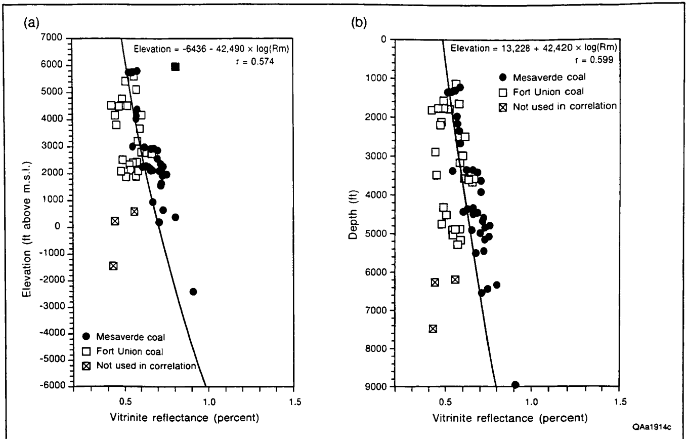
Figure 65. Fort Union vitrinite reflectance profiles relative to (a) elevation and (b) depth. Vitrinite reflectance values remain constant or slightly decrease with increasing depth. This unusual vitrinite reflectance profile may be due to vitrinite reflectance suppression from bitumen generated in the coals during coalification. Equations determined using both Fort Union and Mesaverde vitrinite reflectance data were used to construct a coal rank map of the base of the Fort Union.
