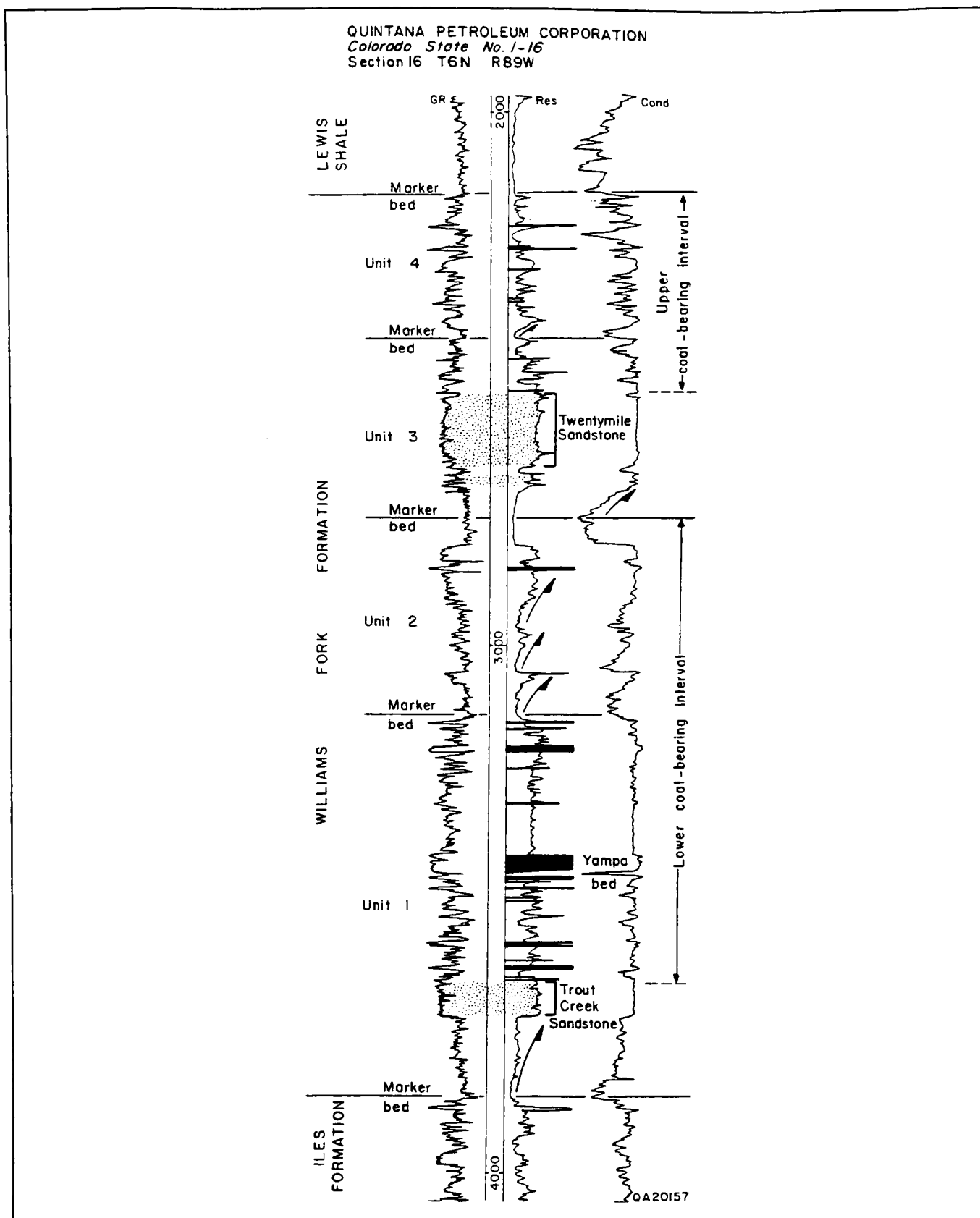
Figure 11. Genetic stratigraphy of the upper Mesaverde Group in the eastern Sand Wash Basin. Coal beds are identified on an accompanying density log. Surfaces bounding genetic units are defined by regionally extensive, low-resistivity shale marker beds.
