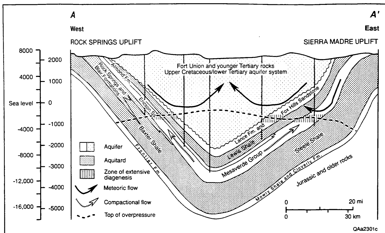
Figure 45. West-east cross section through Washakie Basin (modified from Law and others, [1989]). Recharge is over Sierra Madre and Rock Springs Uplifts. Ground water flows basinward, turning upward upon convergence from the basin margins, aquifer pinch-out, encountering the top of geopressure, or a combination of these. The top of regional overpressure is a no-flow boundary. Line of section is shown in figure 1 of Tyler and Tremain (this vol.).
