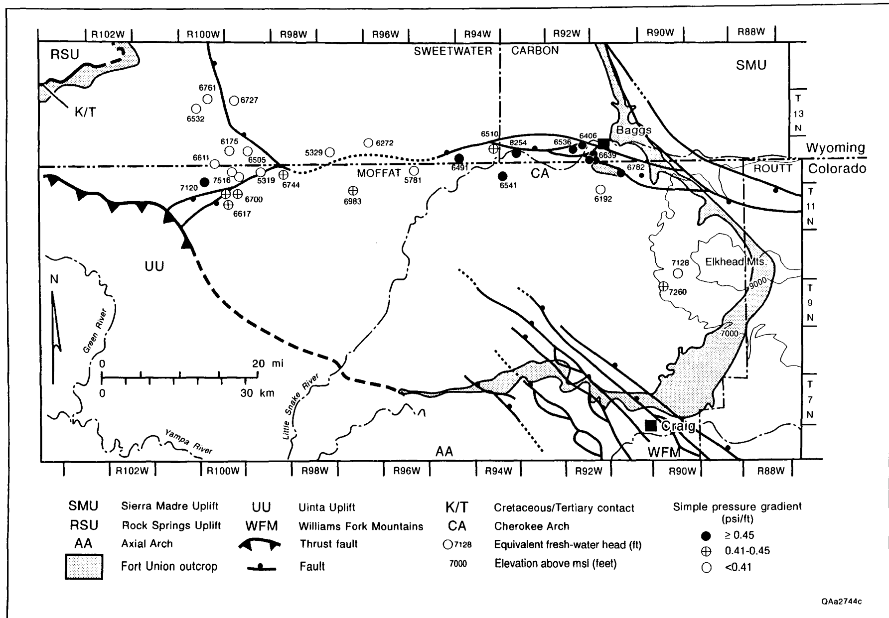
Figure 73. Equivalent fresh-water heads and pressure gradients in the lower coal-bearing unit, Fort Union Formation. The northwestward flow of water from the Elkhead Mountains and artesian overpressure are controlled by complex faulting along the Cherokee Arch and the distribution of coals and sandstones in the lower coal-bearing unit. Heads do not change significantly across the basin, suggesting sluggish lateral flow.
