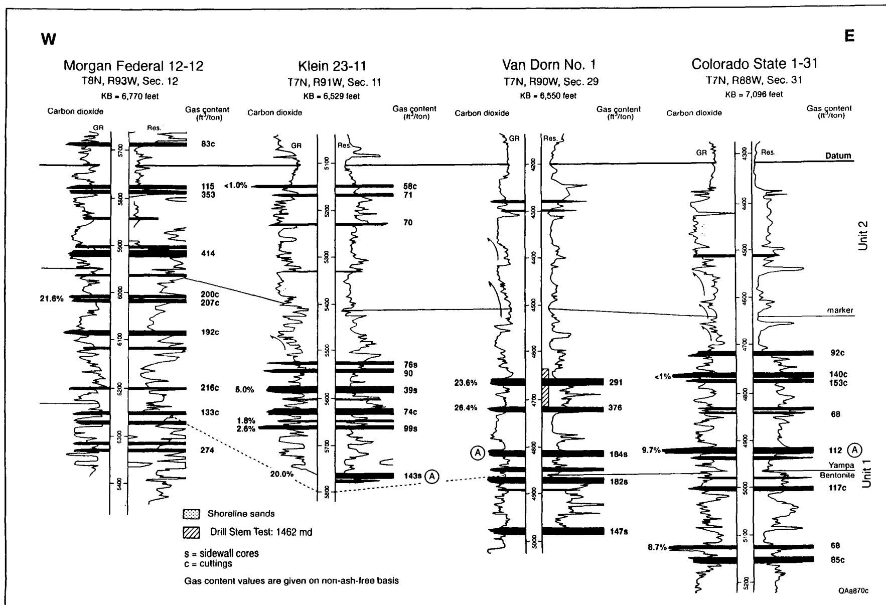
Figure 34. West-east cross section showing the changes in gas content and gas composition between different Mesaverde coal beds. The high gas contents in coal beds at 5,900 ft (1,799 m) in the Morgan Federal 12-12 well may be due to stratigraphic and structural trapping of migrating coalbed gases.
