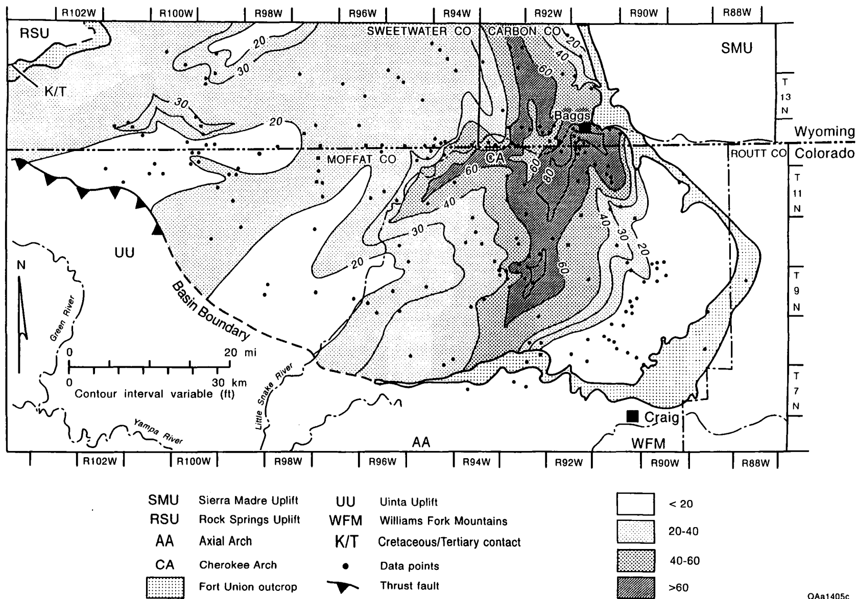
Figure 60. Net-coal-thickness map of the lower coal-bearing unit, Fort Union Formation, Sand Wash Basin. Thickest coal bed development (>60 ft [18.3 m]) occurs above and alongside a south-north oriented fluvial system between R92W and R94W.
