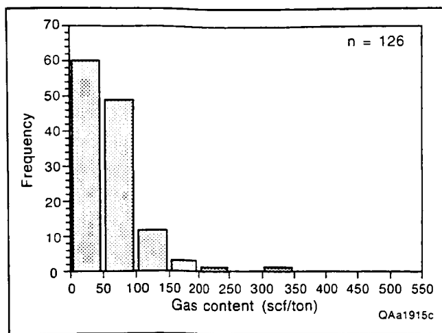
Figure 67. Histogram of gas content values, Fort Union coal samples.
