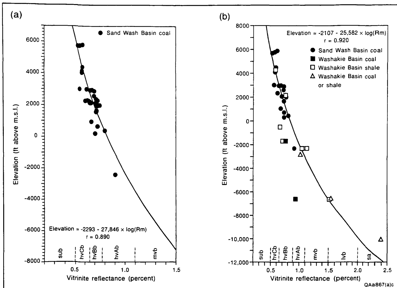
Figure 28. Vitritine reflectance profiles, Sand Wash Basin. (a) Elevation versus vitritine reflectance values of Mesaverde coals in the Sand Wash Basin. (b) Elevation versus vitritine reflectance values of Mesaverde coals and shales from the Sand Wash and Washakie Basins. The equations in (a) and (b) were used to estimate vitritine reflectance values based on depth in the two basins.
