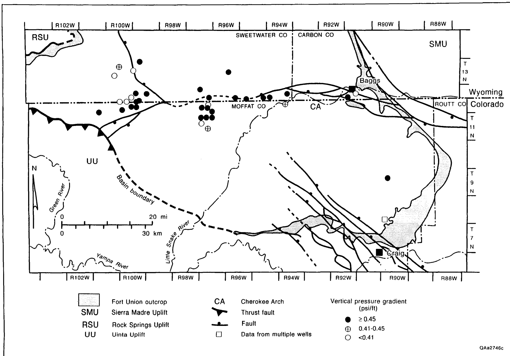
Figure 75. Distribution of vertical pressure gradients by well, Fort Union Formation. Most of wells located along the Cherokee Arch have vertical pressure gradients greater than 0.45 psi/ft ( >10.2 kPa/m), suggesting a strong potential for upward flow. Compactional fluids and gases generated from the deeper parts of the basin may be converging on the arch.
