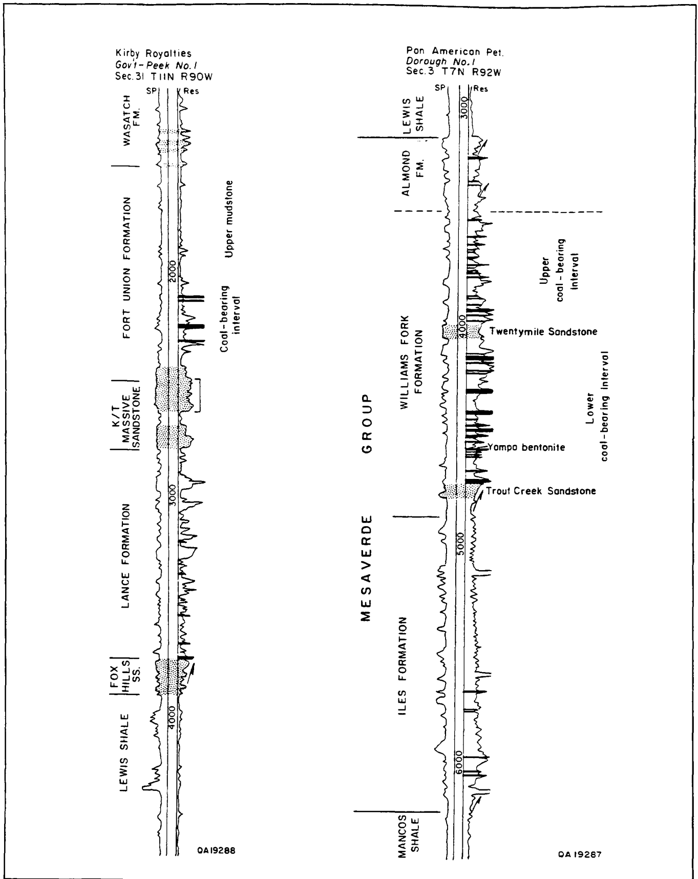
Figure 10. Stratigraphy of the Sand Wash Basin. The most important coal-bearing interval is the lower Williams Fork Formation. Fort Union coals are also important.
