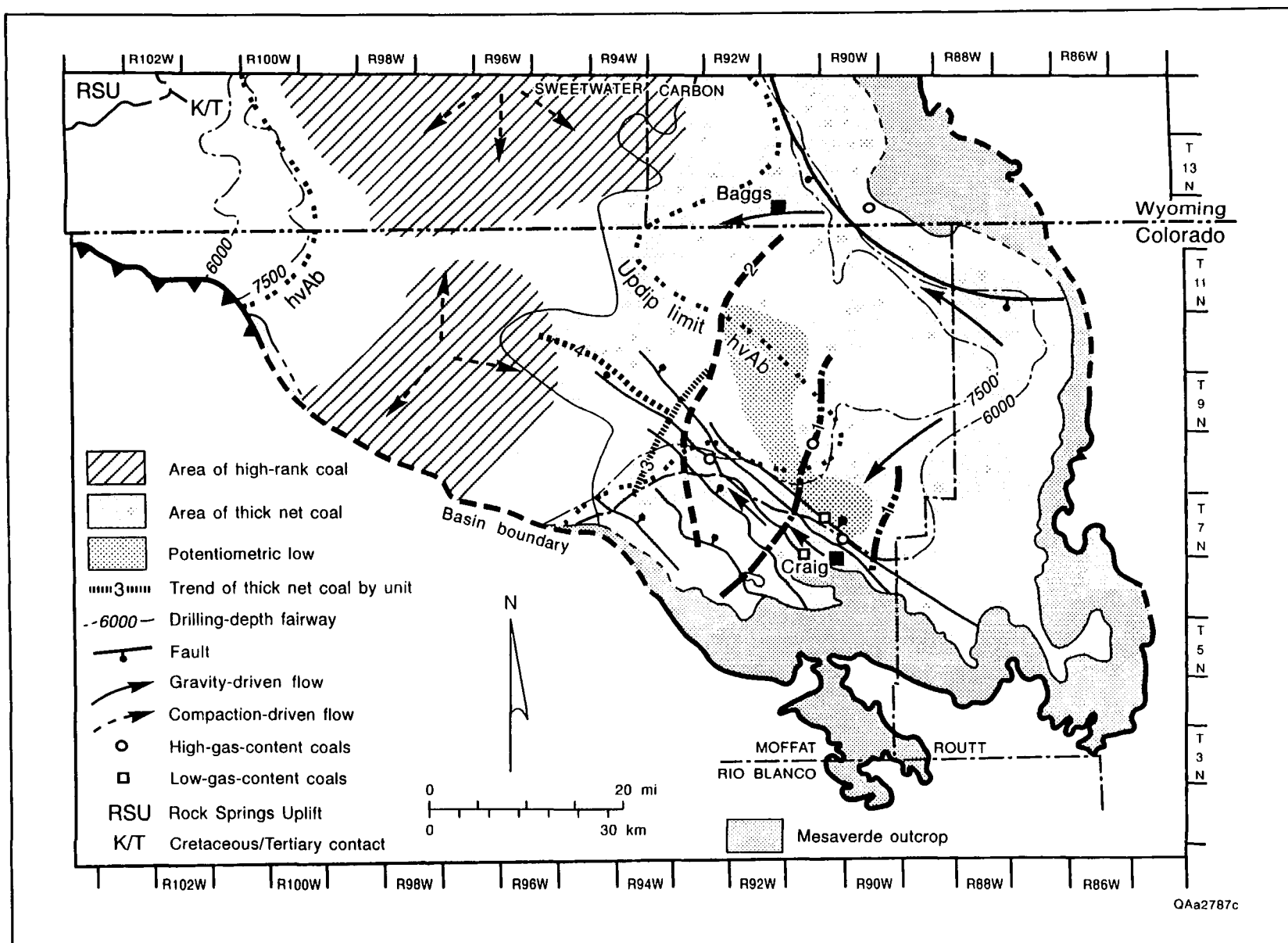
Figure 80. Geologic and hydrologic characterization of the Williams Fork Formation, Sand Wash Basin. Drilling-depth fairways hug eastern margin of the basin, reflecting steep structural dip. Ground water flows westward toward and along the Cedar Mountain fault system (CMFS) up the coal-rank gradient. Compactional flow is in the opposite direction, up and out of the basin center. Prospective coals lie basinward in association with the CMFS.
