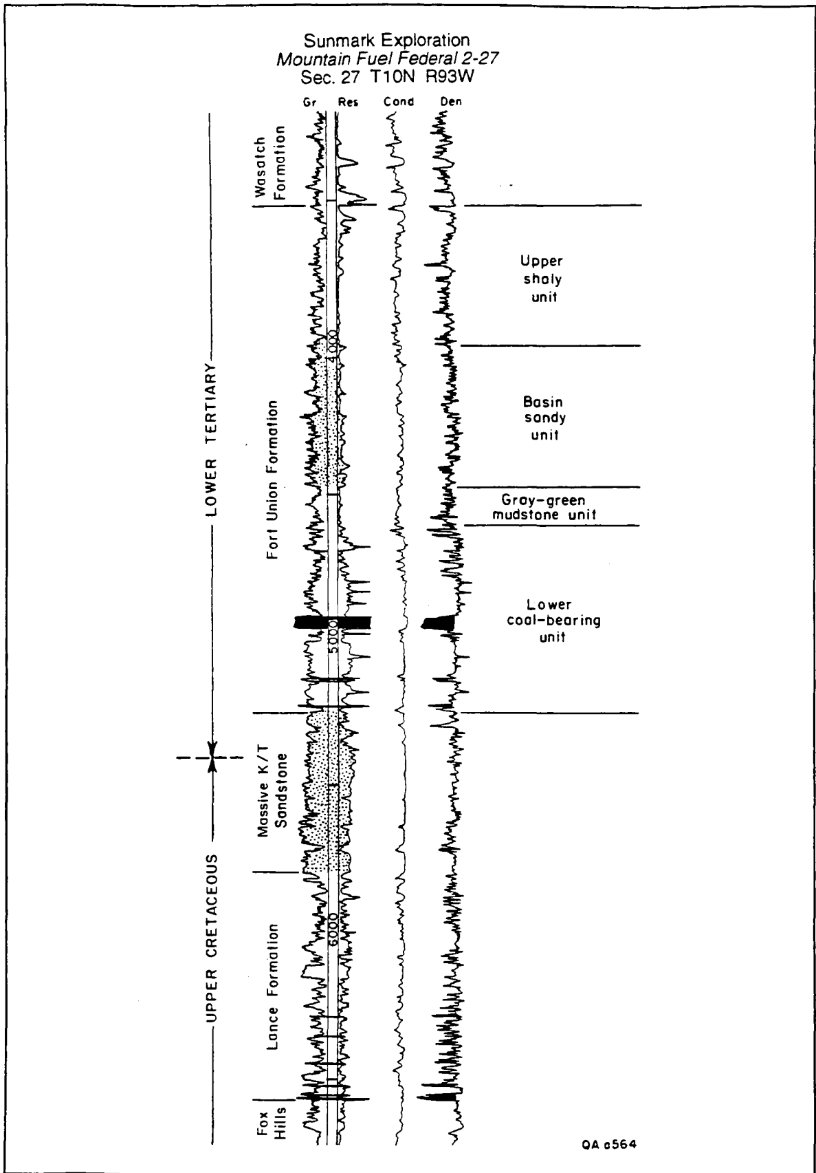
Figure 48. Type log and stratigraphic nomenclature of the Paleocene Fort Union Formation, Sand Wash Basin, and the occurrence of coal. Coal beds identified from density and sonic logs. See figure 52 for location.
