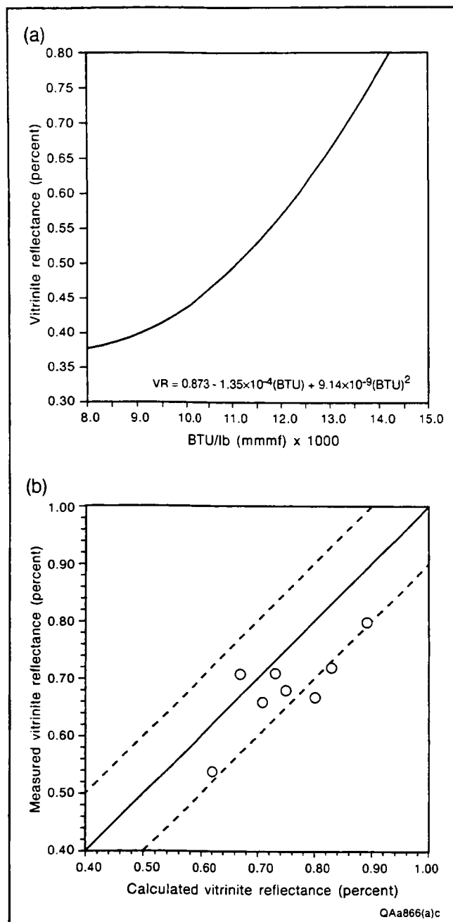
Figure 27. Correlation between vitrinite reflectance and coal Btu (mmmf). (a) Equation and graph used to convert Btu data into equivalent vitrinite reflectance values. (b) Comparison between calculated and measured vitrinite reflectance values. Vitrinite reflectance, proximate, and ultimate data were provided by operators and by Tremain and Toomey (1981).
