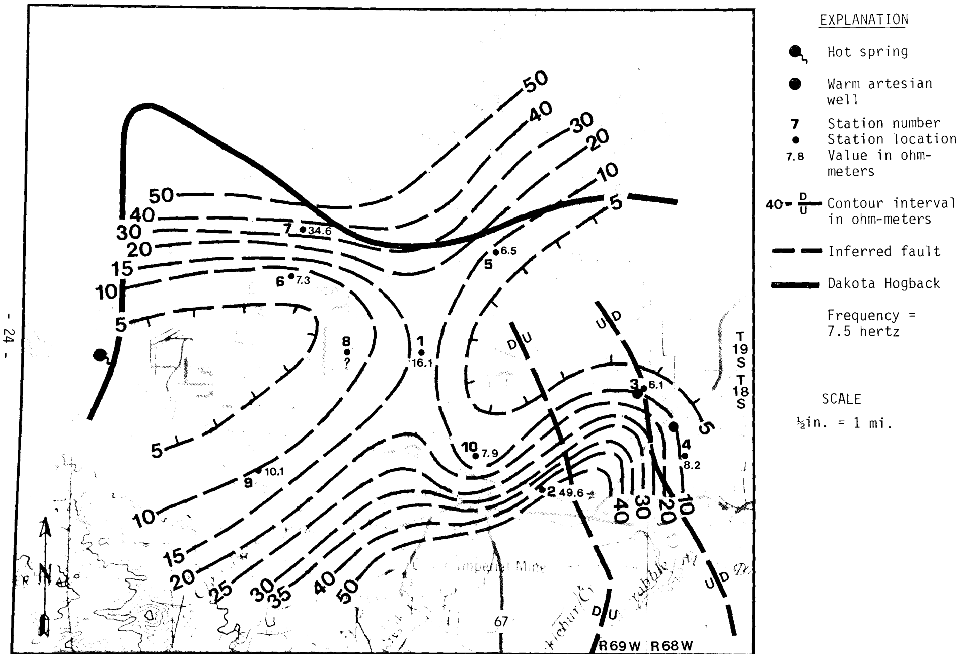
Figure 16. Audio-magnetotelluric survey
