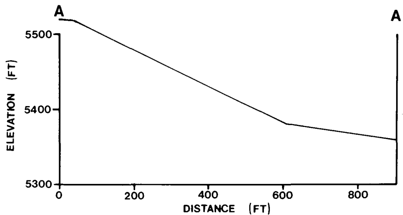
Figure 21. Soil mercury traverse A-A' and surface topography profile, State Penitentiary.
