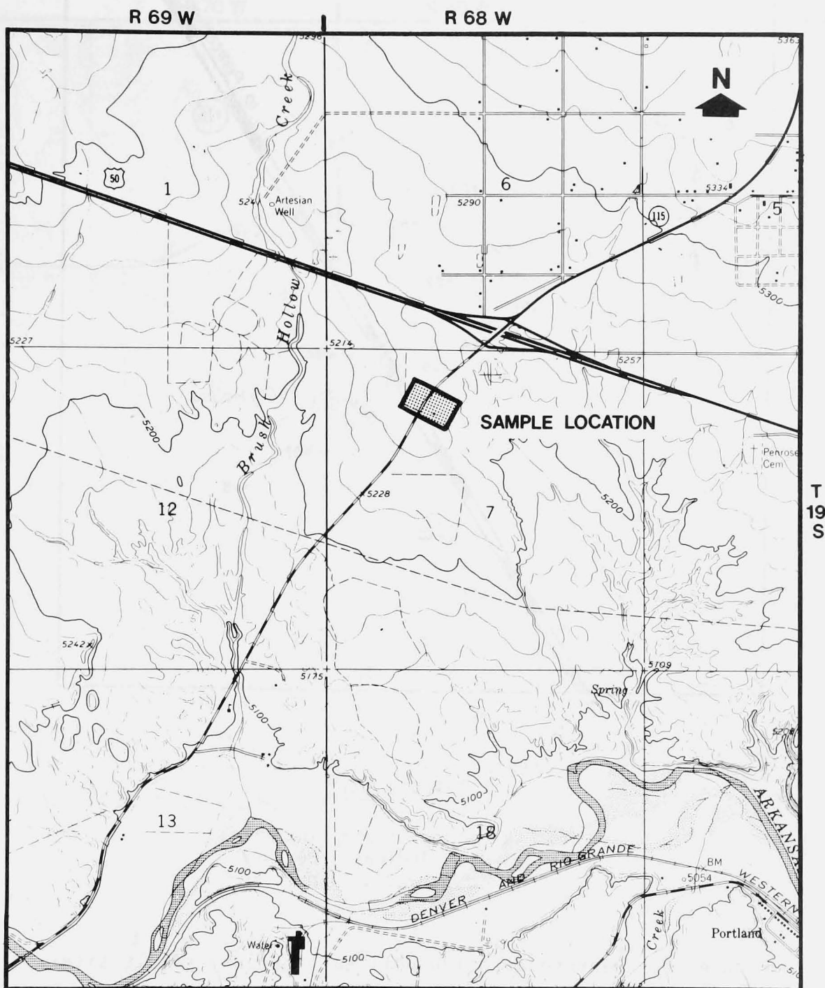
Figure 18. Penrose soil mercury sample area.
