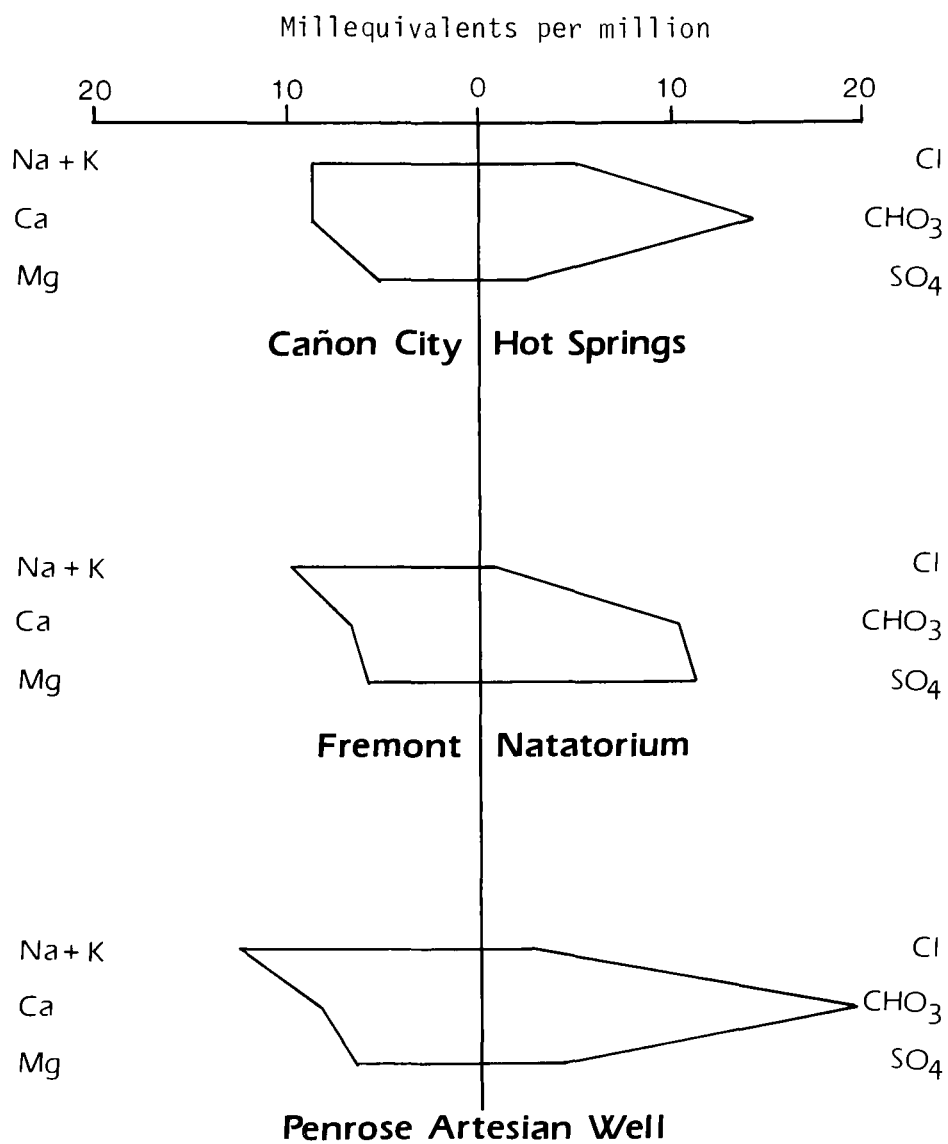
Figure 9. Water quality diagram.
