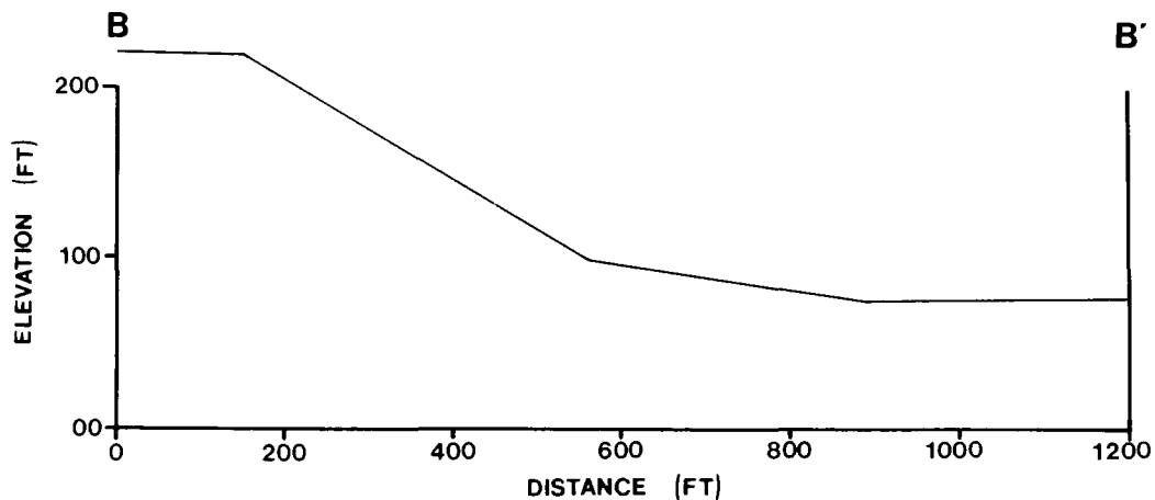
Figure 22. Soil mercury traverse B-B' and surface topography profile, State Penitentiary.
