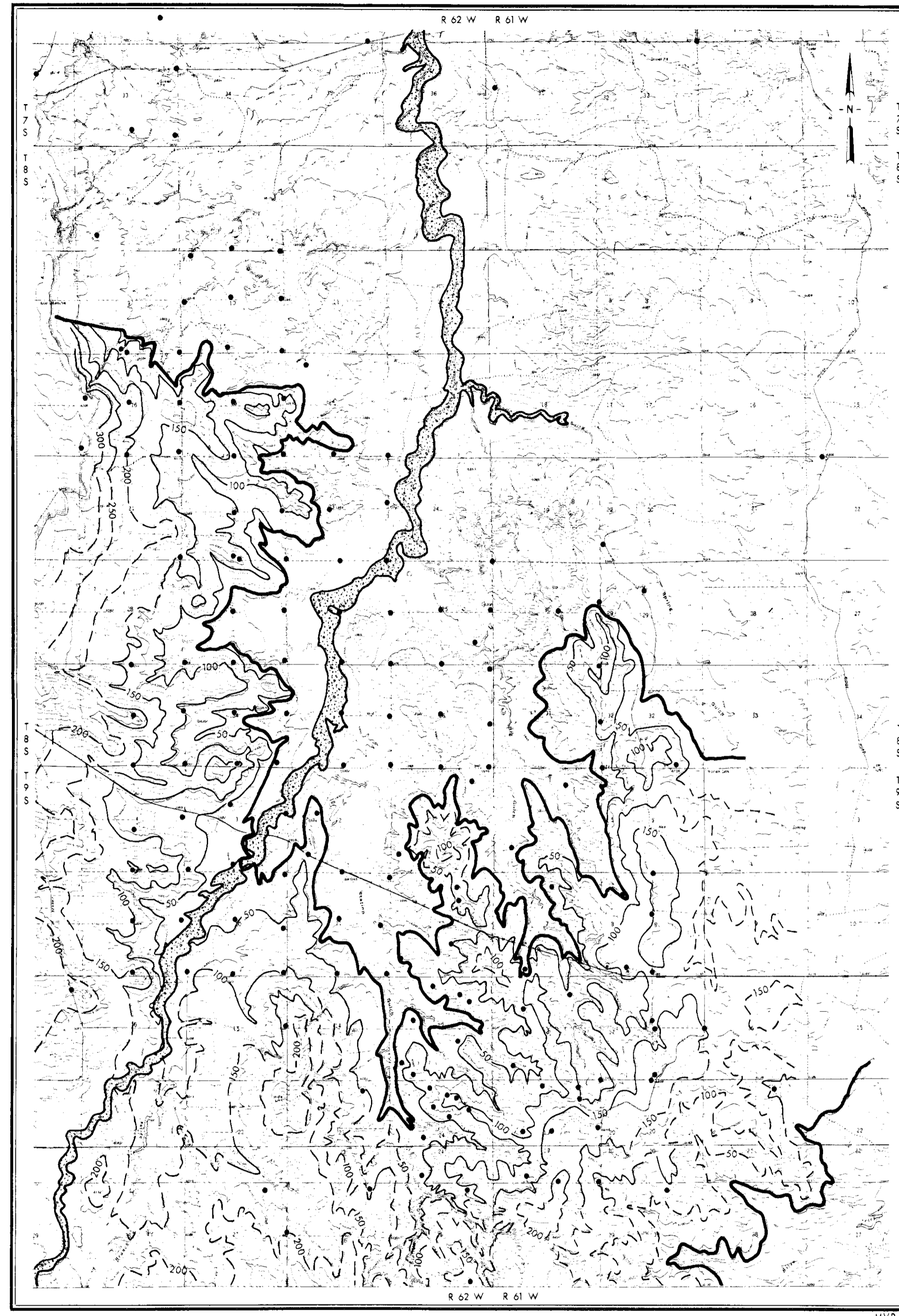
FIGURE 2 EXTENT OF THE ALLUVIAL VALLEY FLOOR AND OVERBURDEN THICKNESS ABOVE THE COMANCHE BED, STATION CREEK AREA
