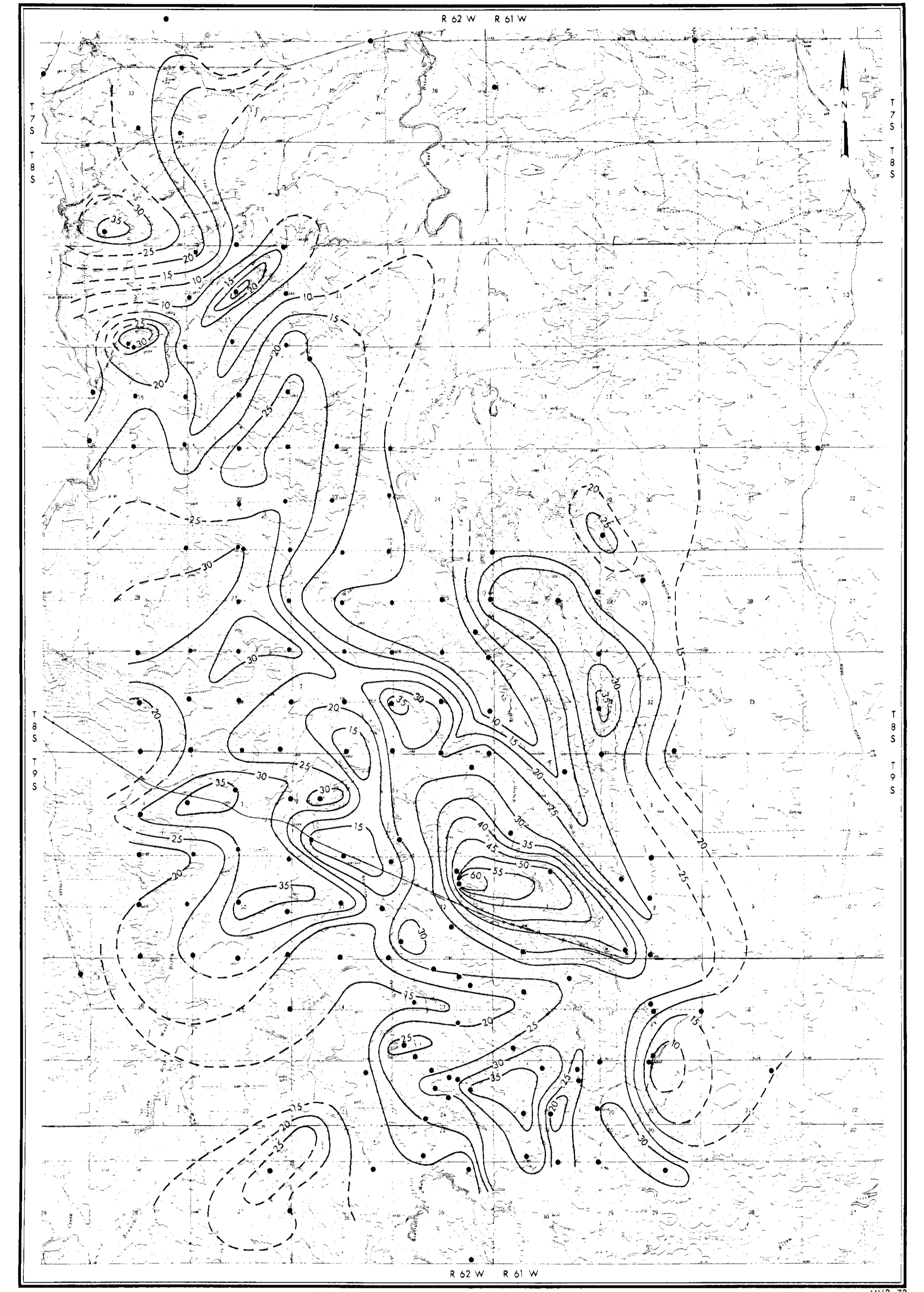
FIGURE 3 TOTAL THICKNESS OF LIGNITE BEDS IN THE DENVER FORMATION, STATION CREEK AREA
