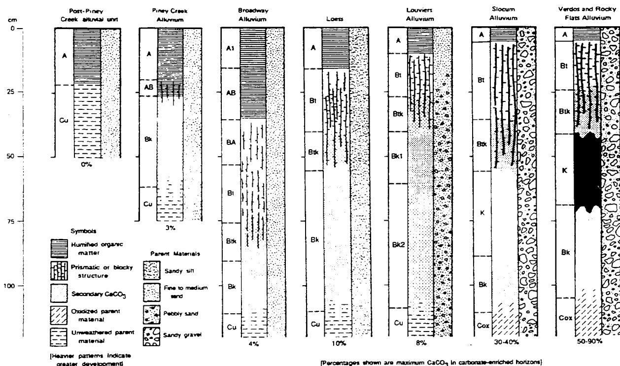
Figure 2. Diagrammatic cross-section showing the Quaternary alluvial units in the Denver area (diagram of Scott, 1963, modified by Madole, 1991)
