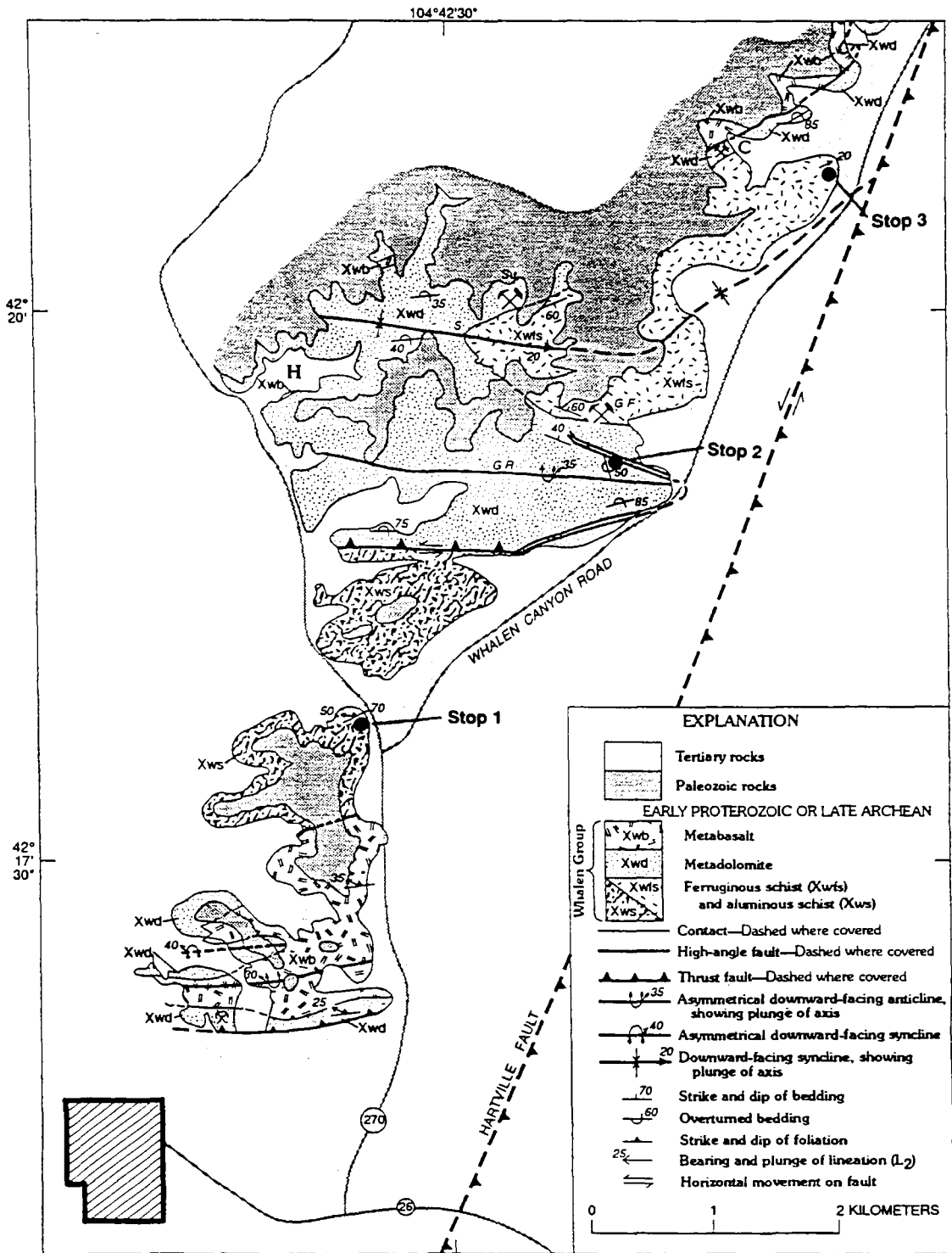
Figure 2. Geologic map of Precambrian rocks in a part of the Guernsey 7 ½-minute quadrangle, Hartville uplift, southeastern Wyoming. C, Chicago mine; H, Hartville; S, Sunrise syncline; GR, Graves Ranch anticline; GF, Good Fortune mine; Su, Sunrise mine. Town of Guernsey is shown by the diagonally-ruled polygon in the lower left corner.
