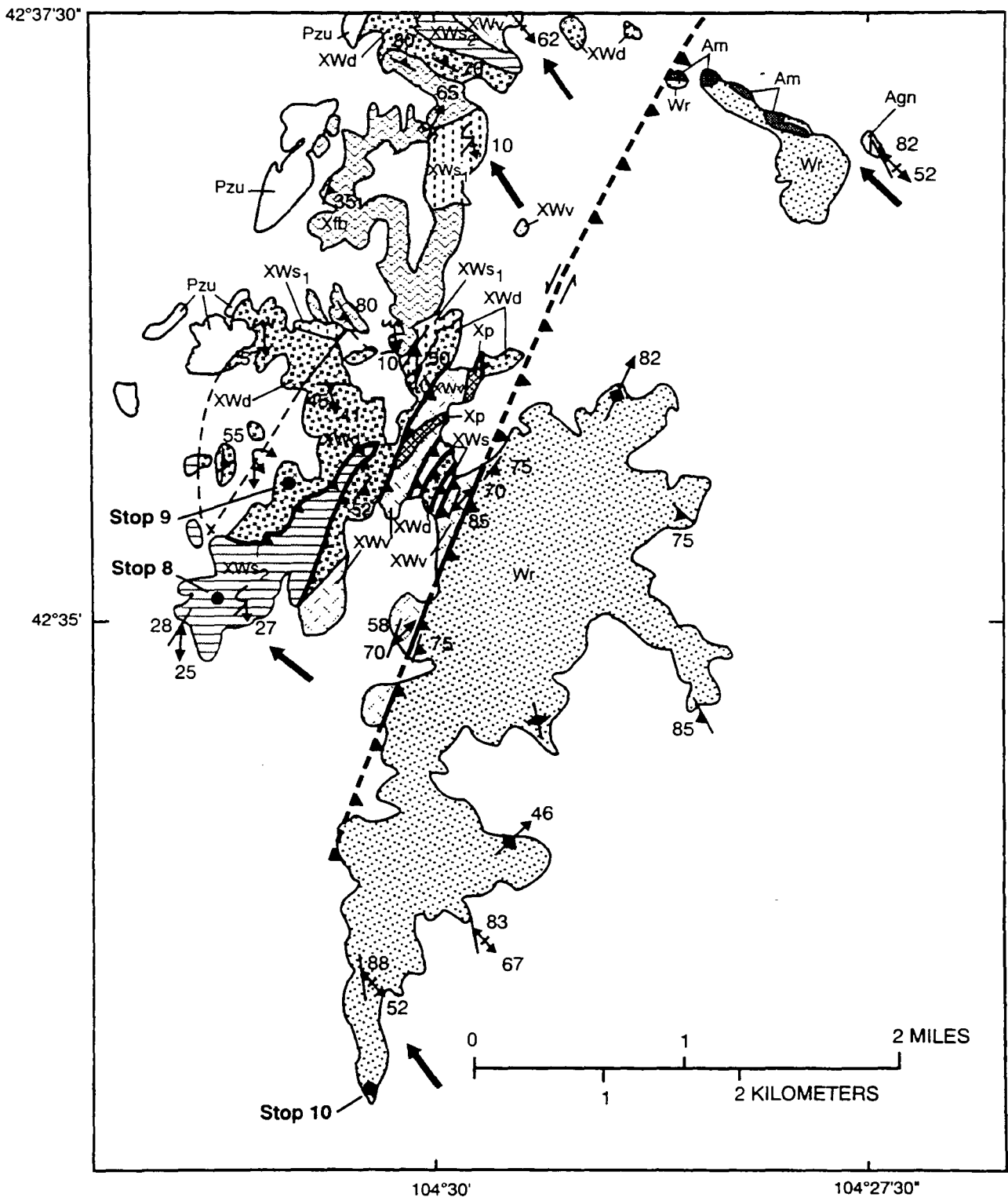
Figure 6. Geologic map of Precambrian rocks in parts of the Rawhide Buttes West and Rawhide Buttes East 7 1/2-minute quadrangles, Hartville uplift, southeastern Wyoming. (legend)
