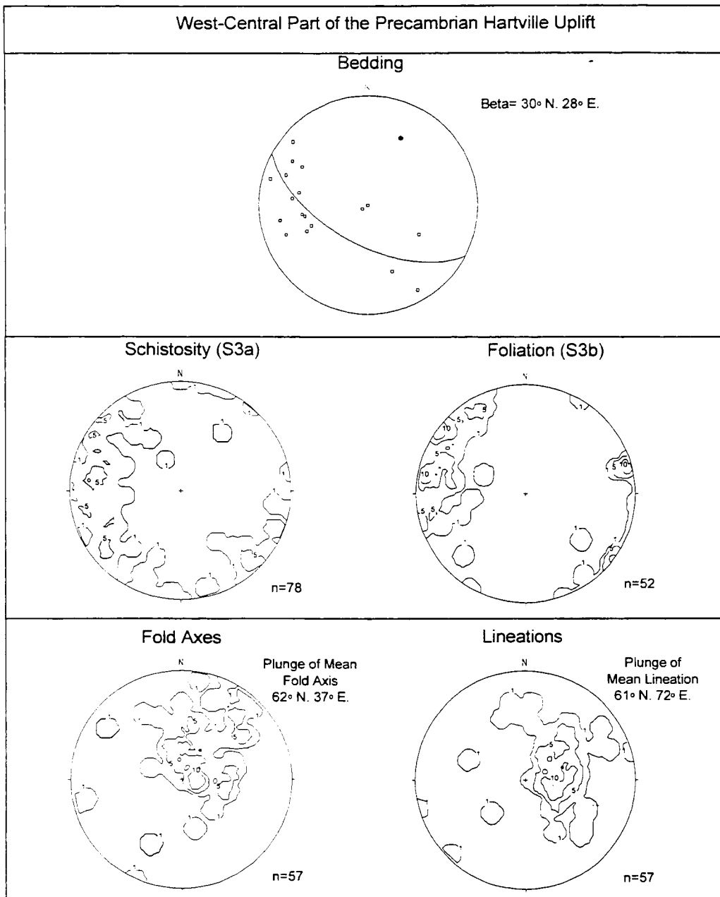
Figure 4. Equal-area projections of D 3 structures and bedding in west-central part of Hartville uplift. Schistosity (S 3a ) and foliation (S 3b ) are discussed in text. Fold axes and lineations are D 3 structures. Structures were measured in Frederick Ranch domain and areas to the north, including area of figure 5.
