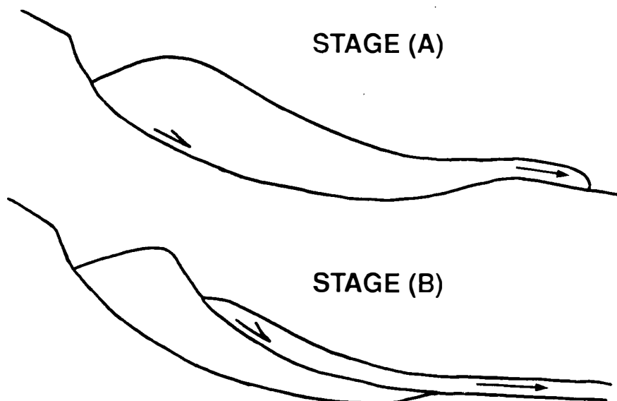
Figure 37. Diagrammatic representation of proposed failure sequence along cross-section B-B'. (Not to scale.)
