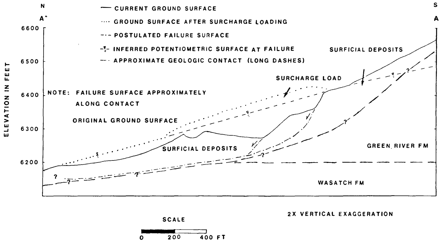
Figure 38. Cross-section along A-A' after surcharge loading.
