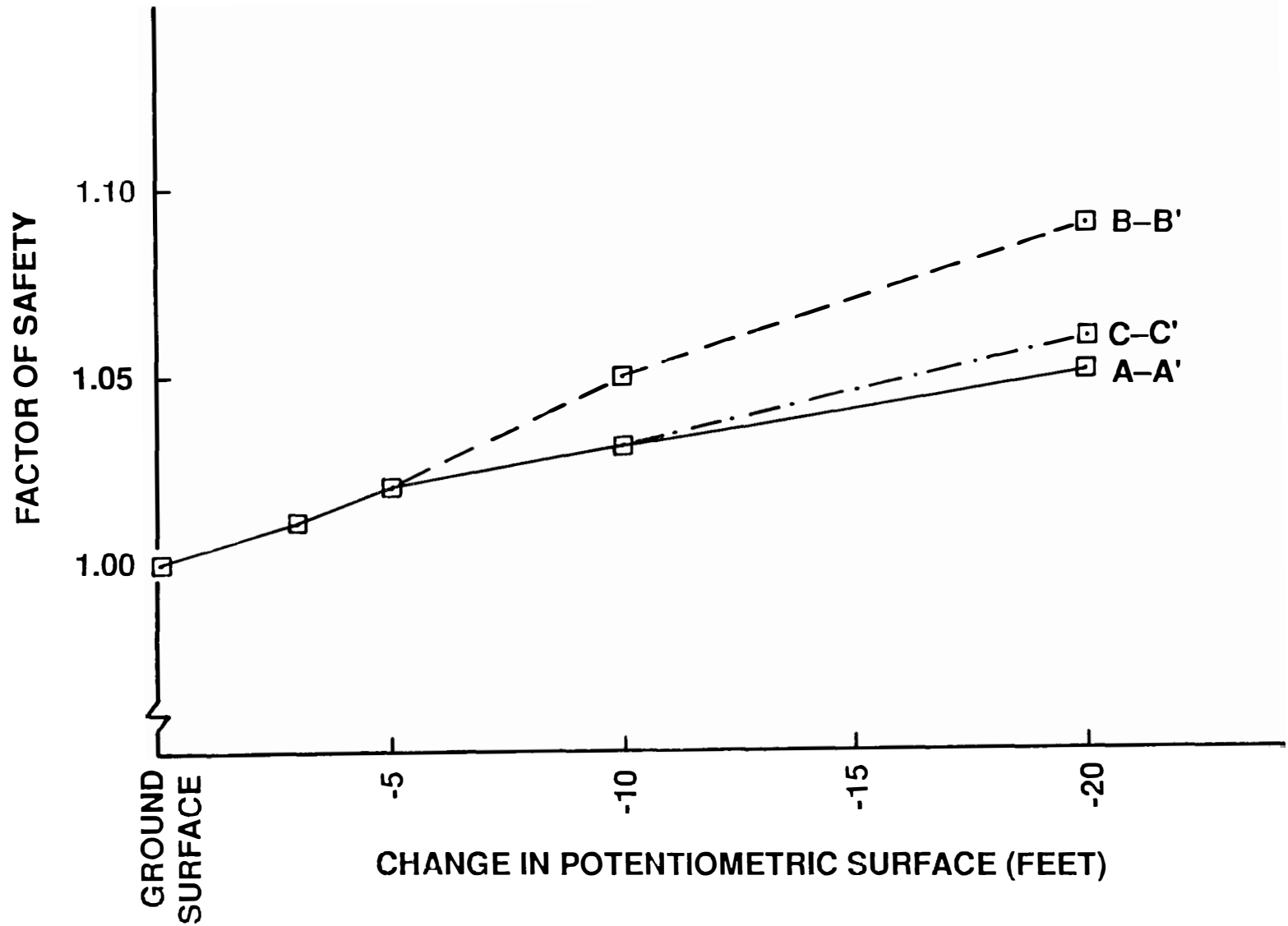
Figure 45. Effect of lowering potentiometric surface on factor of safety.
