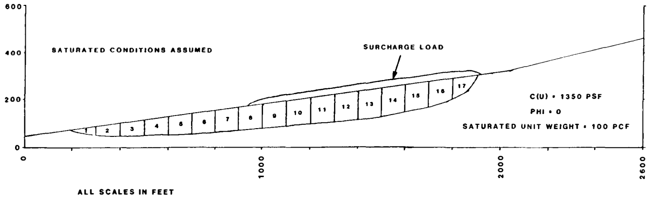
DIAGRAM USED IN TOTAL STRESS ANALYSES PRIOR TO AND AFTER SURCHARGE LOADING FOR HAND COMPUTATIONS OF FACTORS OF SAFETY ALONG PROFILE A-A*.
