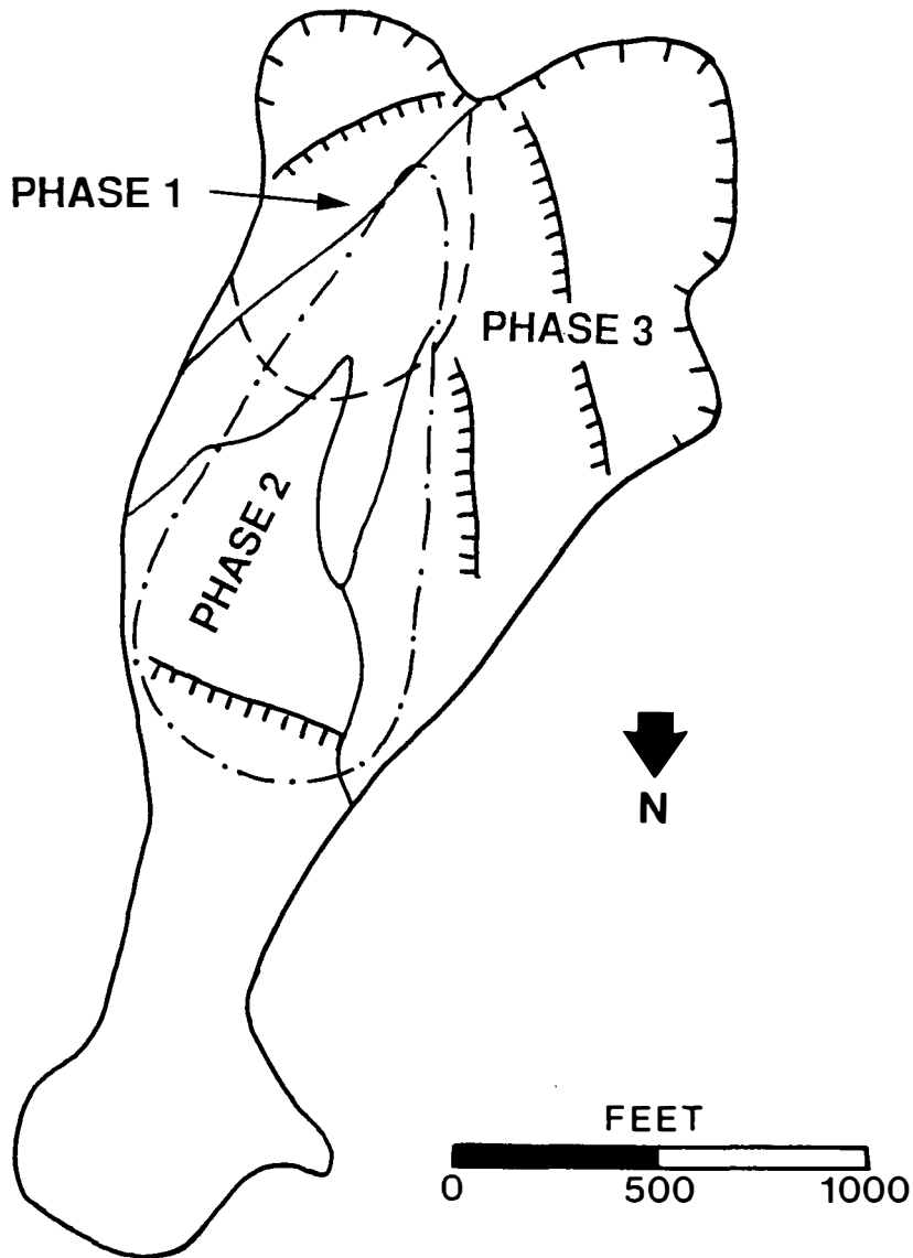
Figure 40. Phase 3 movement of the Roan Creek landslide.
