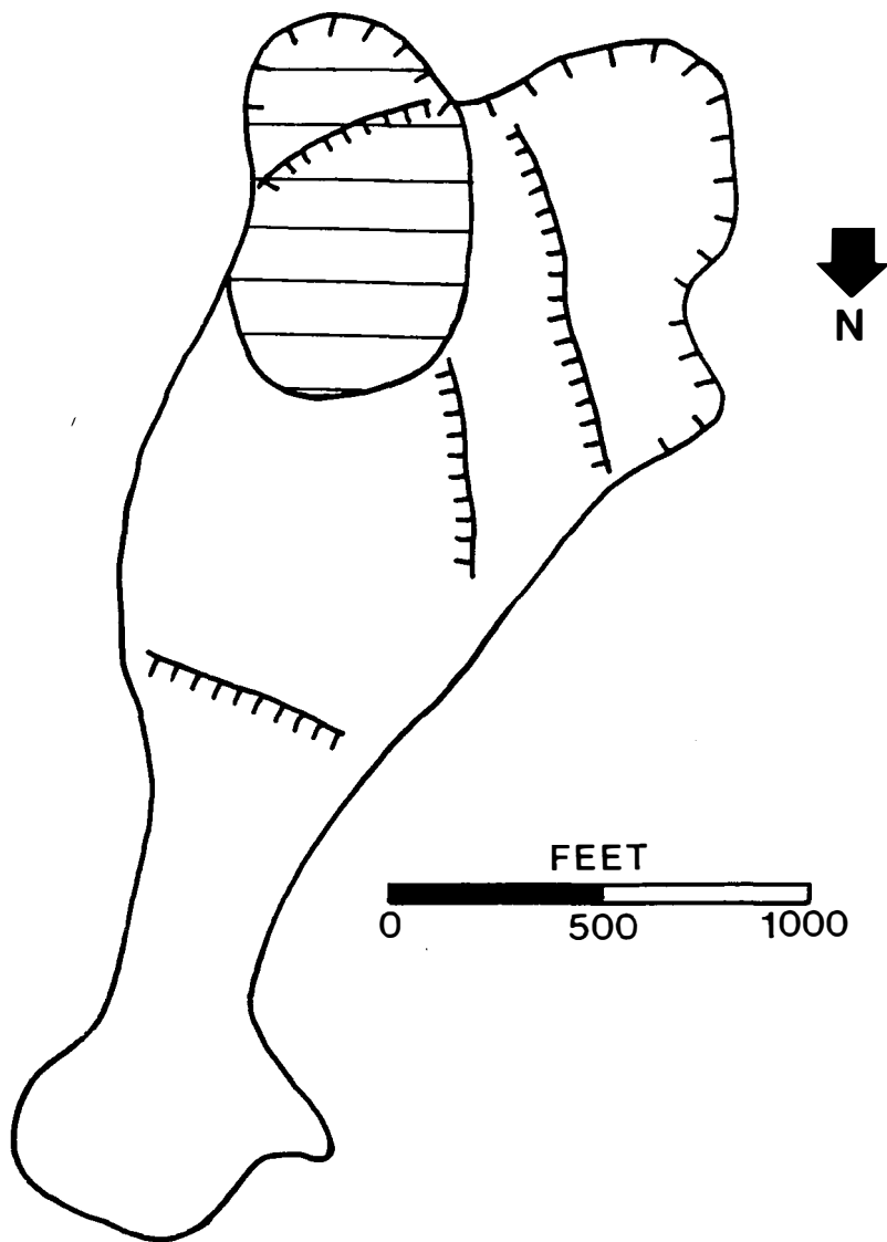
Figure 35. Phase 1 Movement of the Roan Creek landslide.
