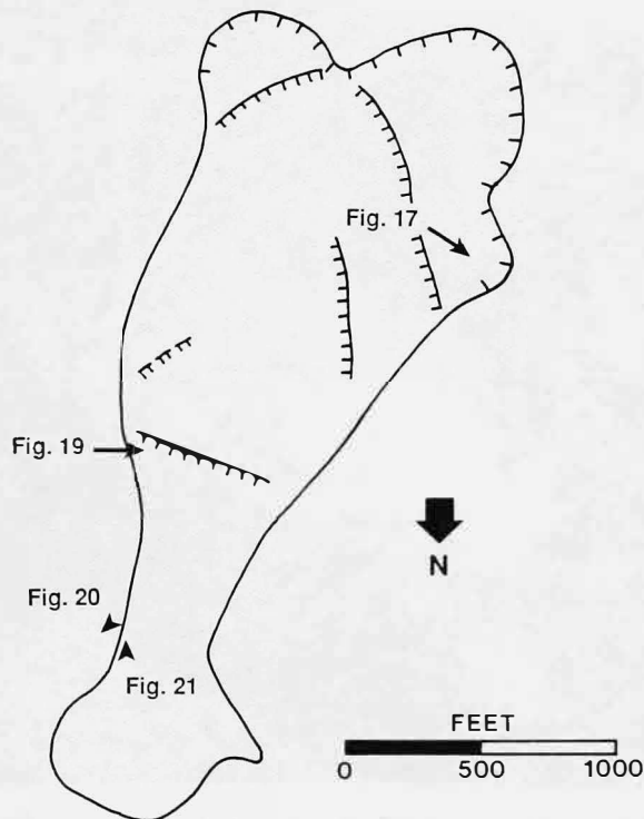
Figure 18. Scarp map of the Roan Creek Landslide.
