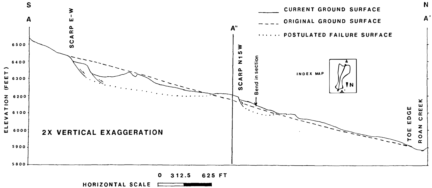
Figure 33. Cross-section along A-A'.
