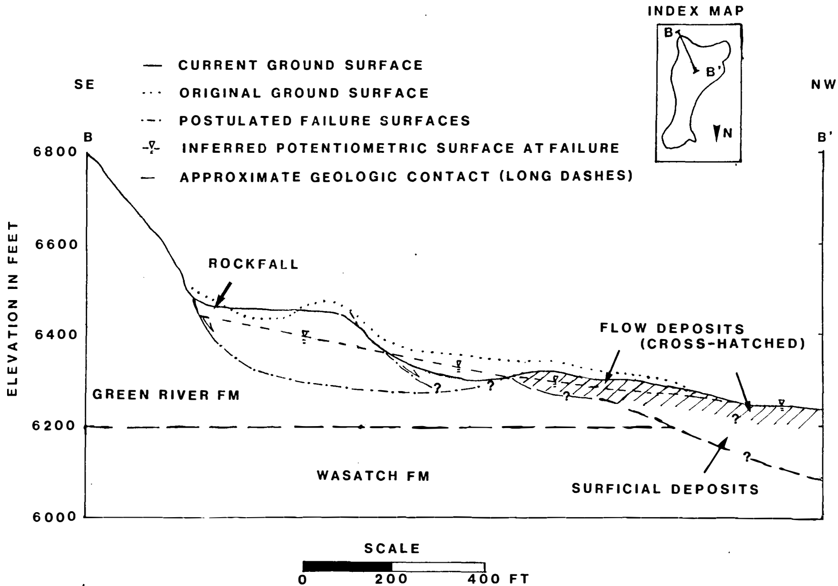
Figure 36. Cross-section along B-B'.
