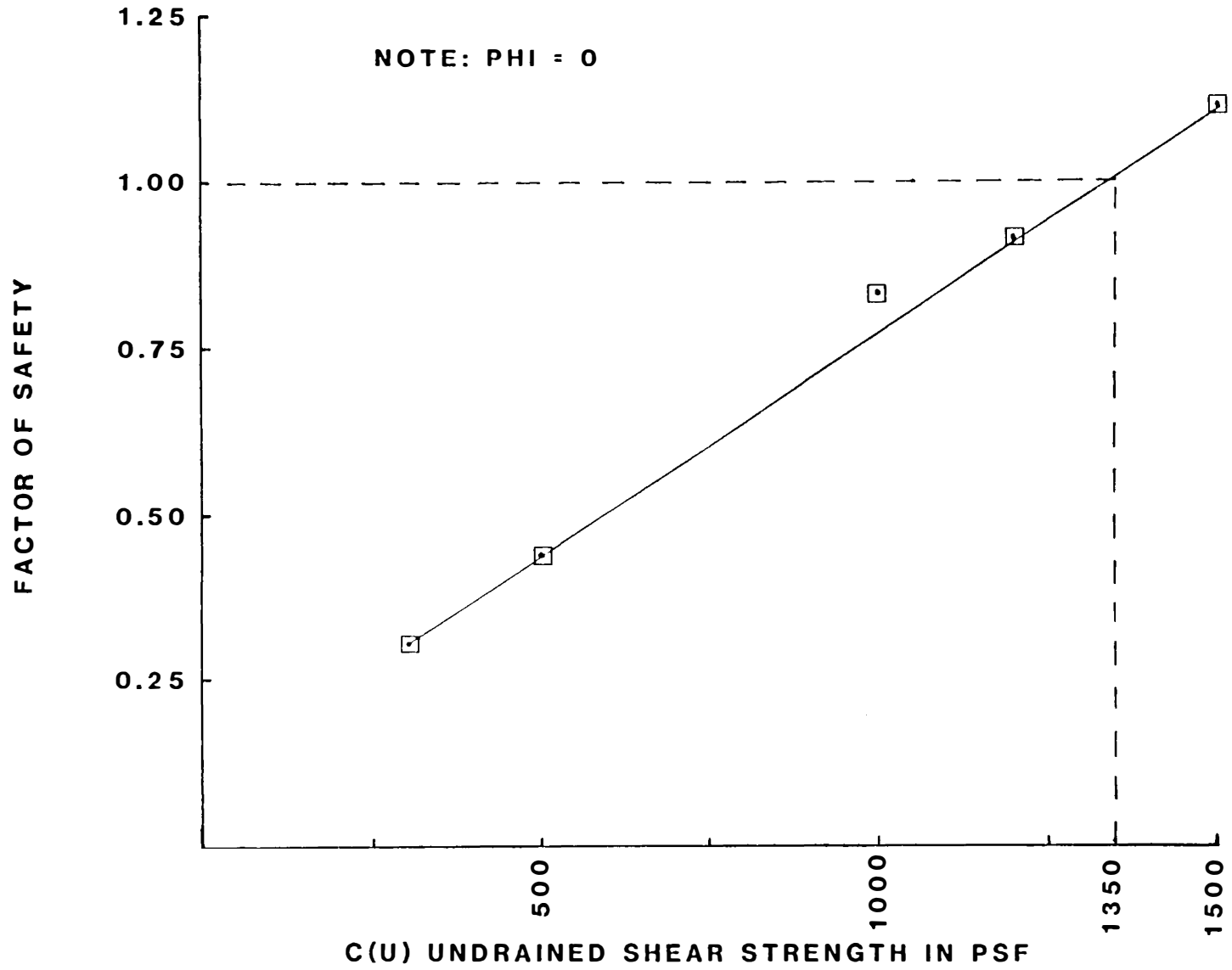
Figure 44. Determination of undrained shear strength.
