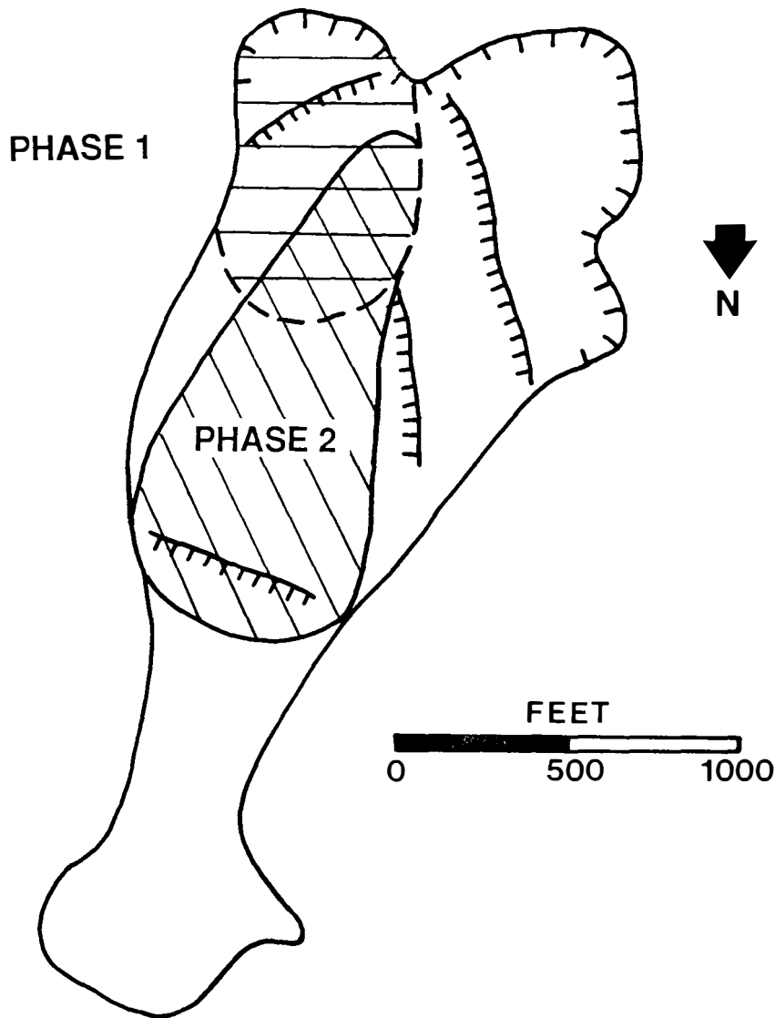
Figure 39. Phase 2 movement of the Roan Creek landslide.
