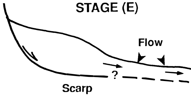
Figure 43. Diagrammatic representation of proposed failure sequence along cross-section C-C'.
