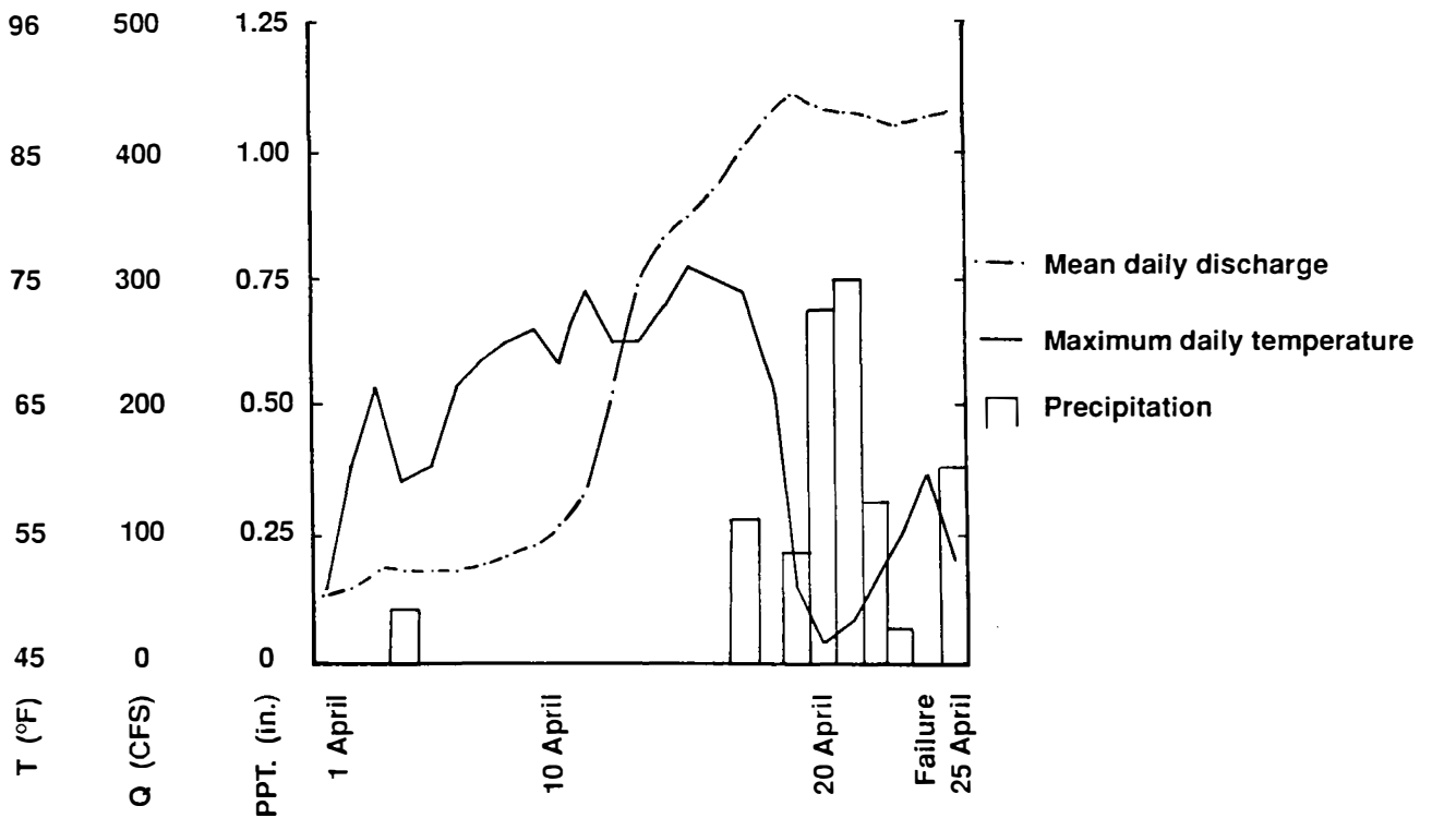
Figure 11. Maximum daily temperature, daily precipitation and mean daily discharge of Roan Creek in the first 25 days of April 1985.
