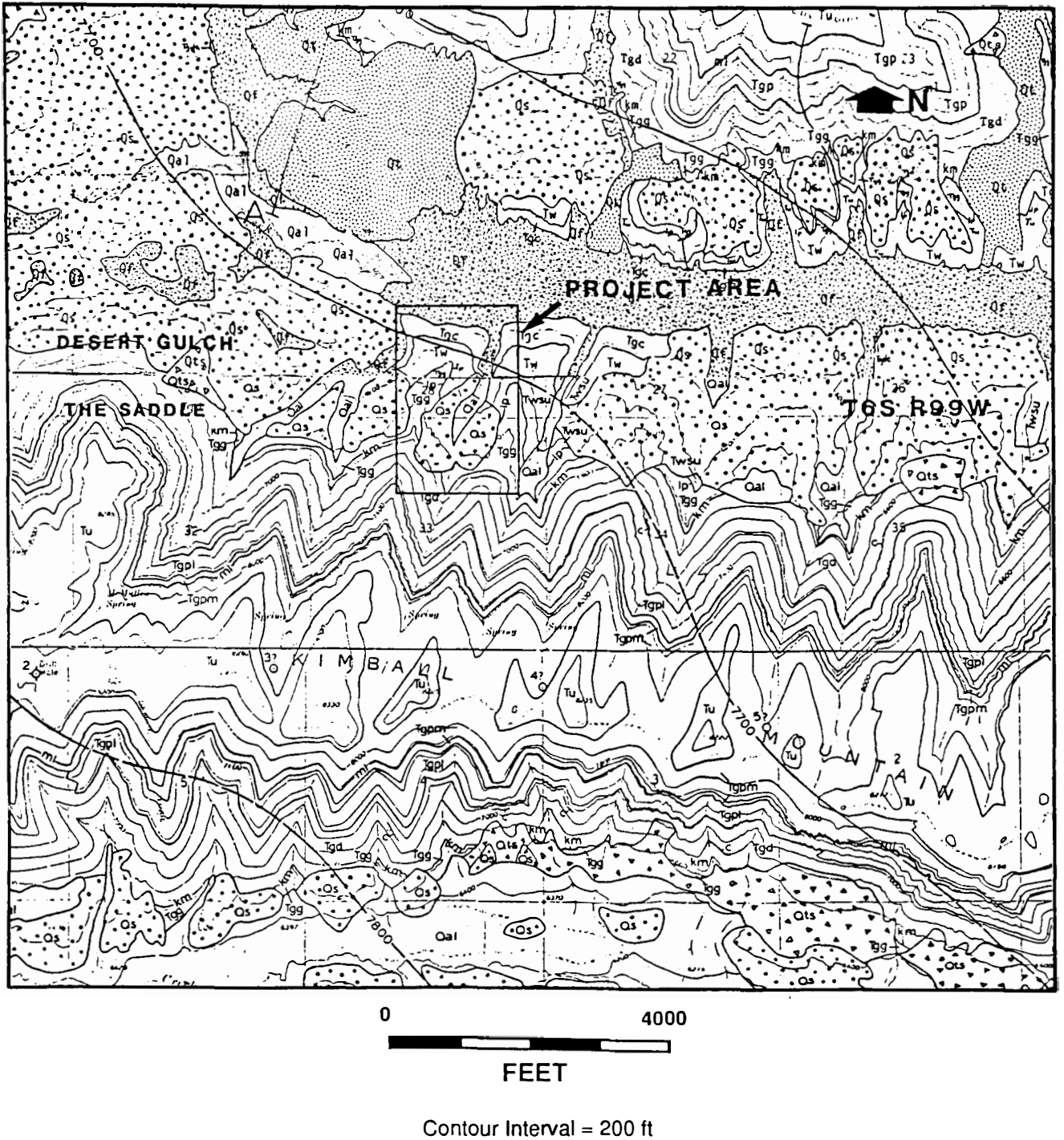
Figure 5. Geologic map of the study area, from Johnson 1977, 1981.
