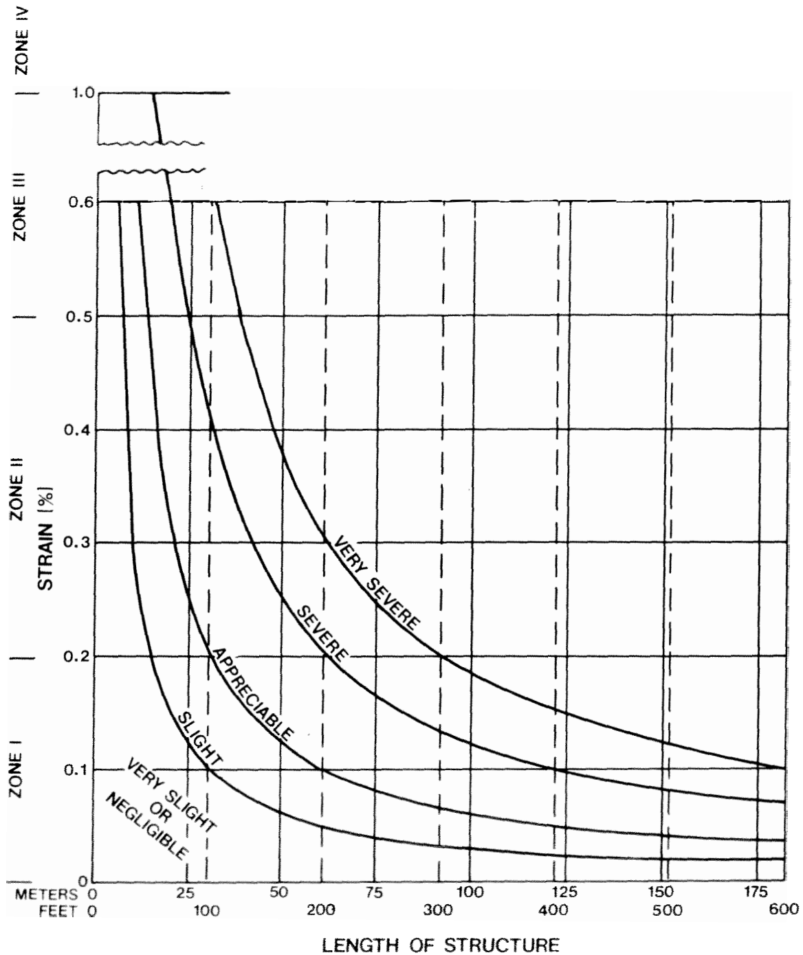
Figure 10. Relationship of damage to length of structure and horizontal ground strain and strain zones in Category 4 (See Table I.) (Modified from National Coal Board, Great Britain, and Baker, 1974).
