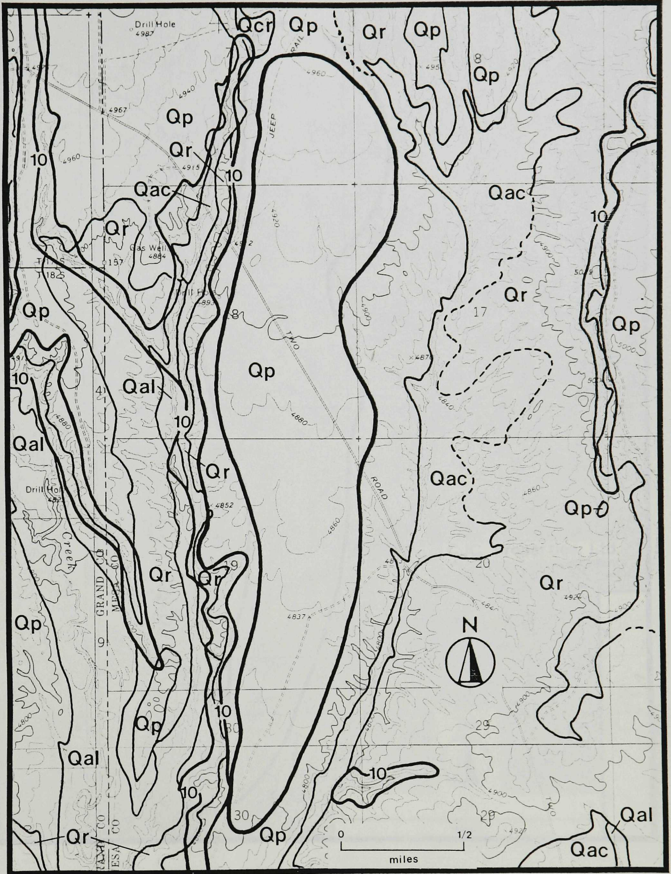
Figure 18. Surficial Geology and Slope Map of the Two Road Site, scale 1:24,000.
