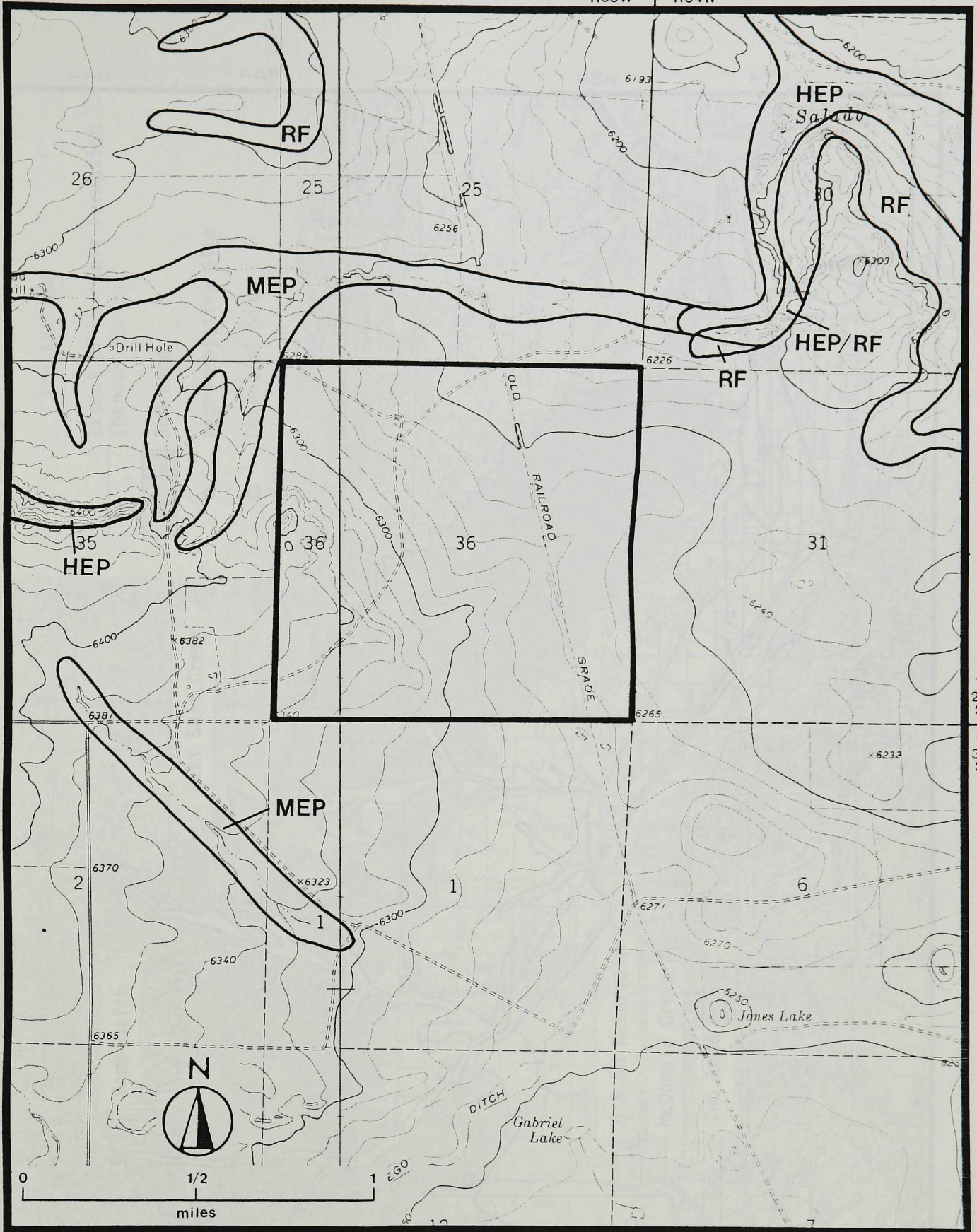
Figure 16. Geologic Hazards and Constraints Map of the Rugby Site, scale 1:24,000.
