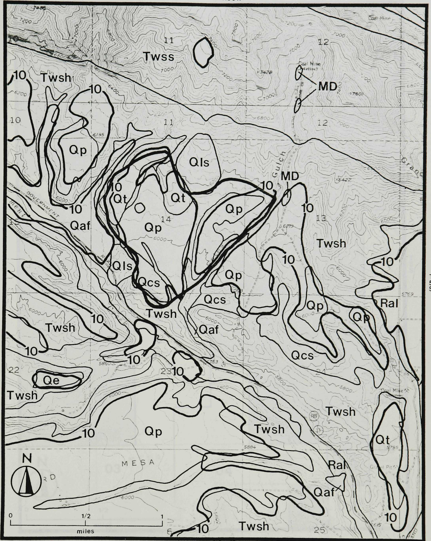
Figure 27. Surficial Geology and Slope Map of the Estes Gulch Site, scale 1:24,000.
