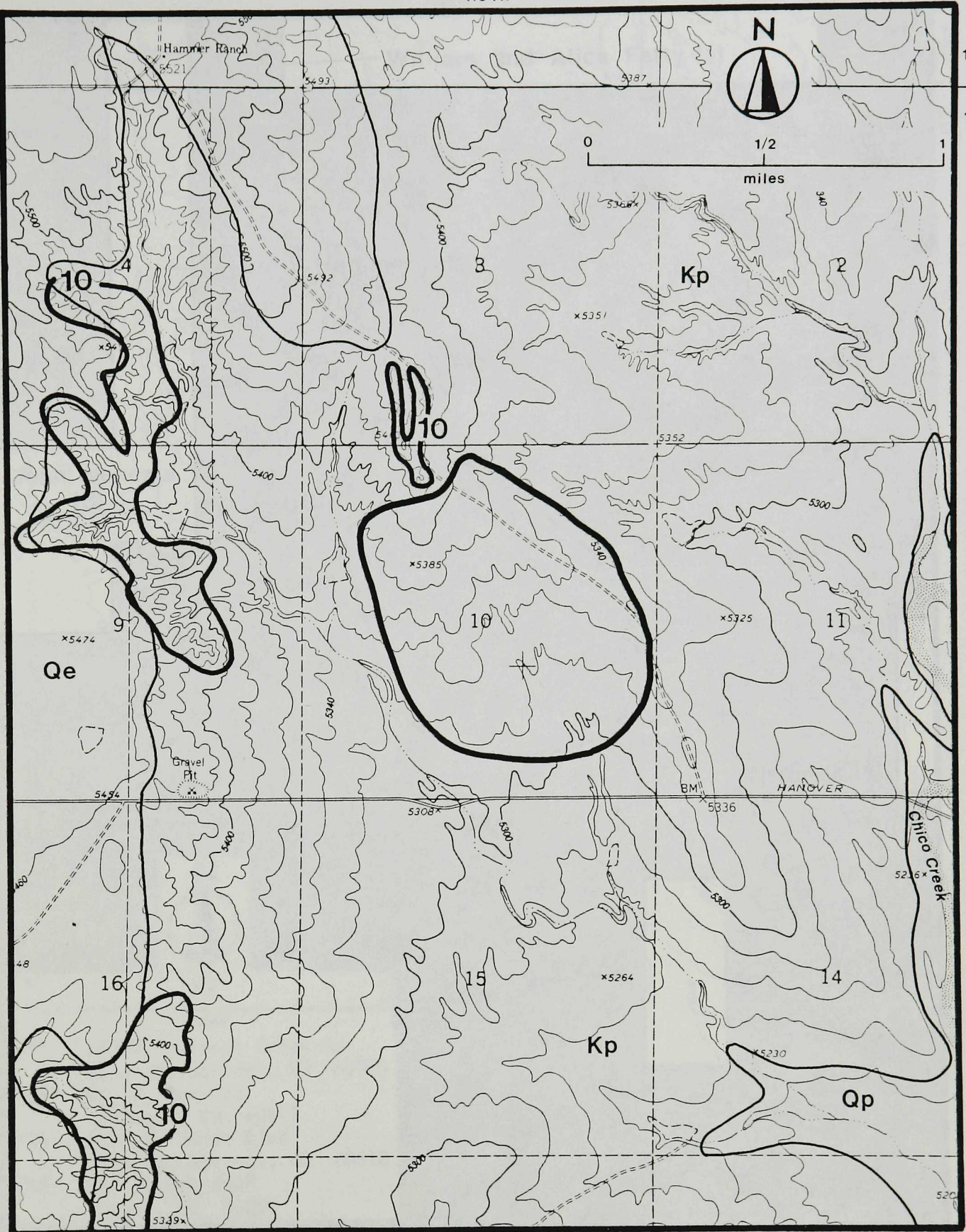
Figure 10. Surficial Geology and Slope Map of the Wigwam Site, scale 1:24,000.
