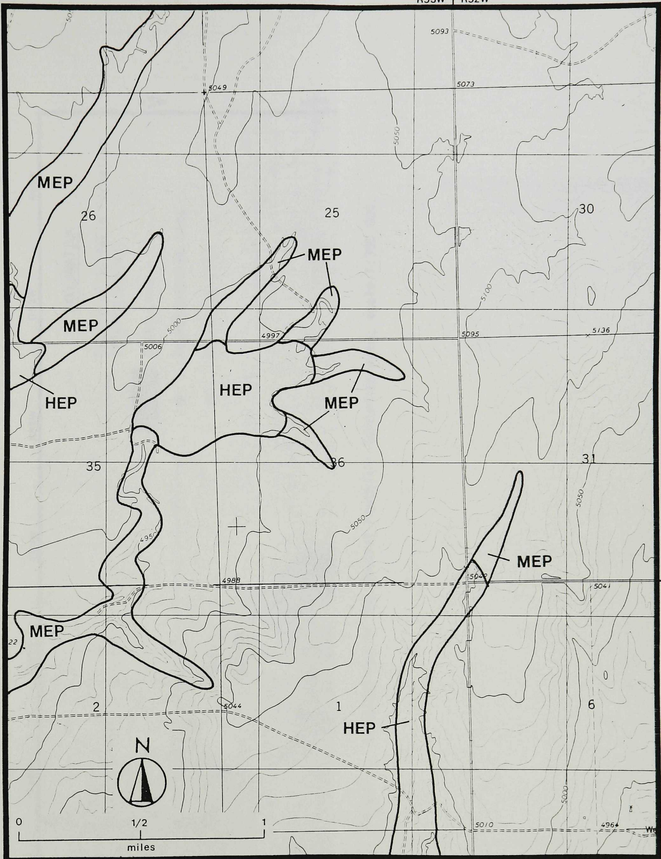
Figure 8. Geologic Hazards and Constraints Map of the Clifford Site, scale 1:24,000.
