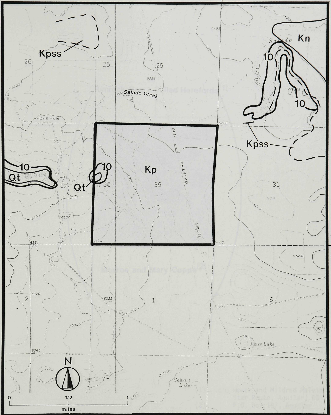
Figure 14. Surficial Geology and Slope Map of the Rugby Site, scale 1:24,000.
