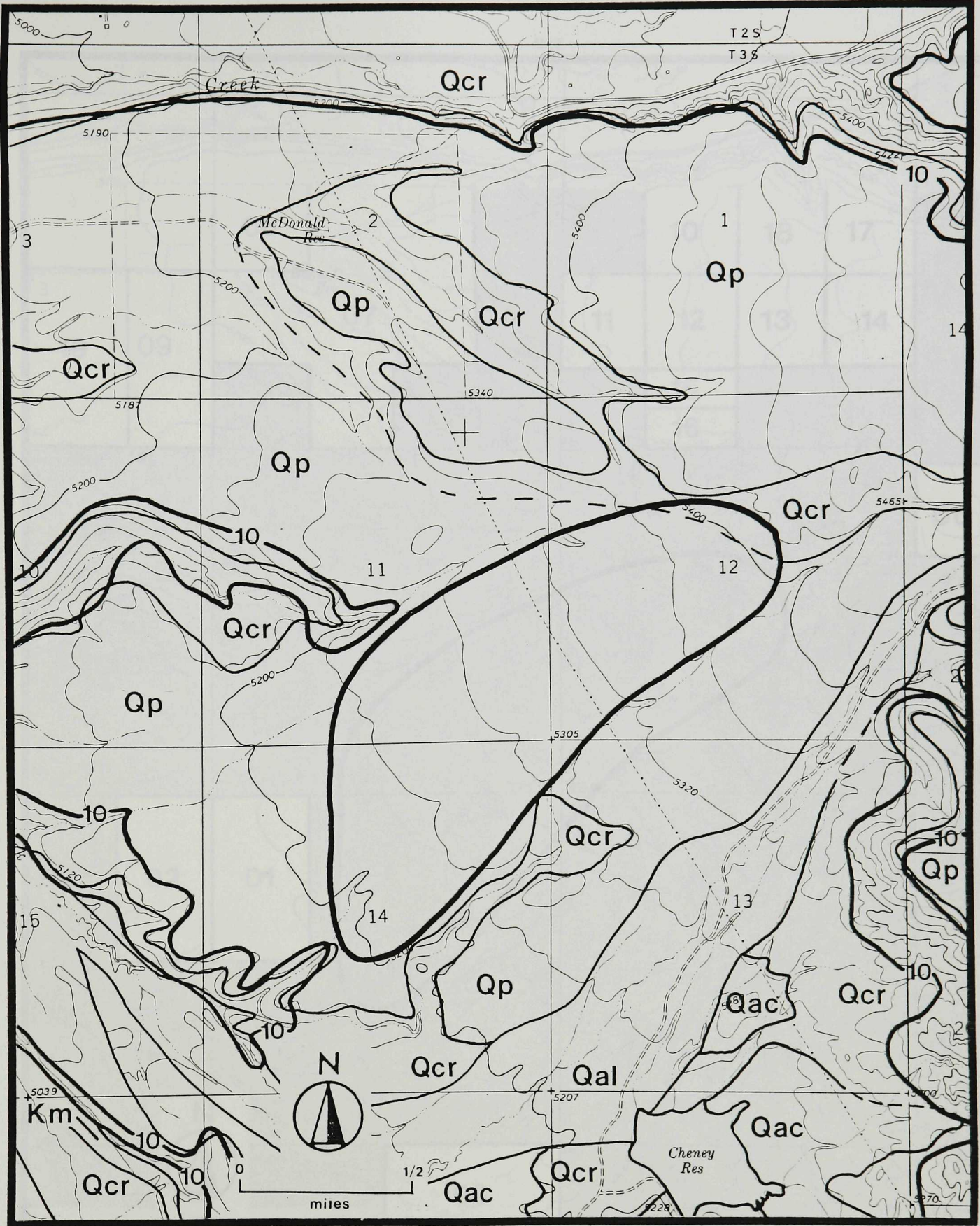
Figure 22. Surficial Geology and Slope Map of the Cheney Reservoir Site, scale 1:24,000.
