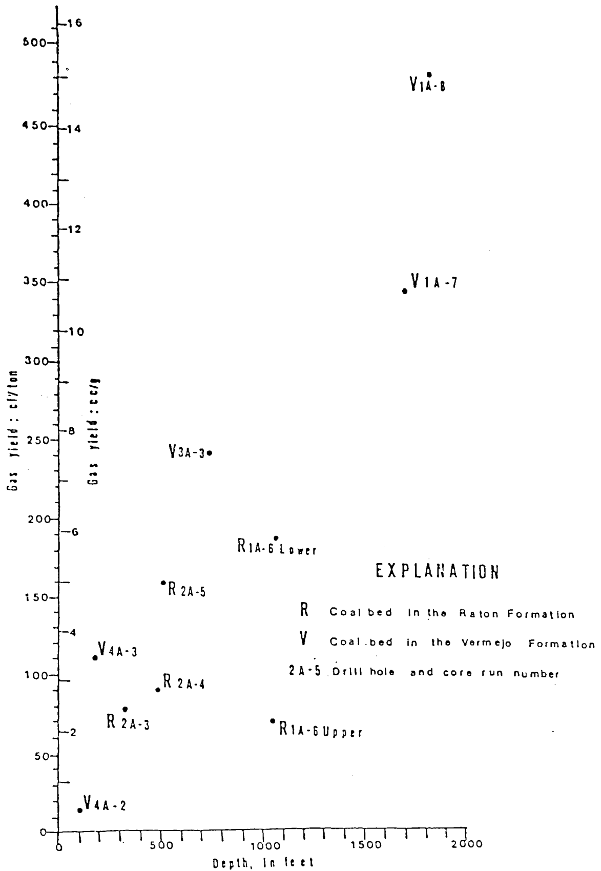
Figure 2.--Depth vs. gas-yield relationships of selected coal core samples from the Raton and Vermejo Formations, Las Animas County, Colorado.
