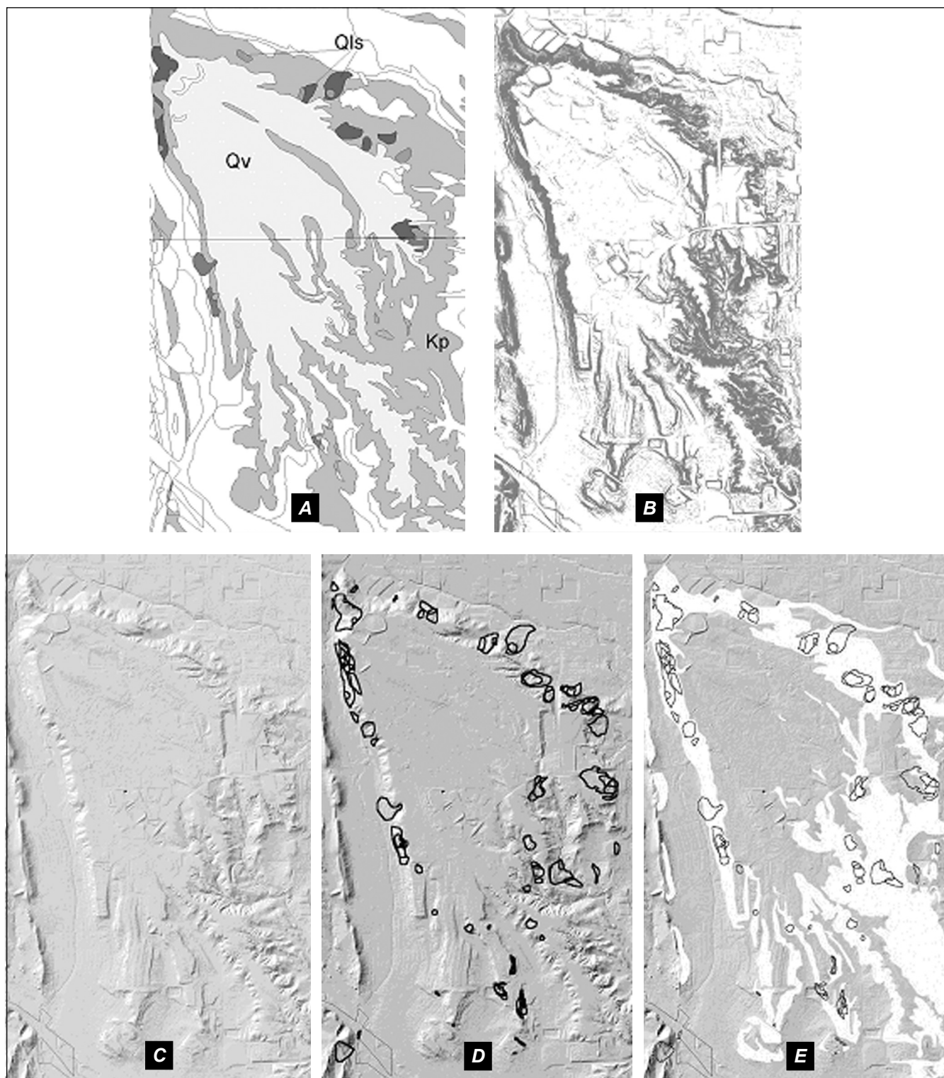
Figure 14. GIS imagery of “The Mesa” area to illustrate map development. Images shown are: (A) geology and published landslides; (B) slope grade; (C) shaded relief DEM; (D) DEM with landslide inventory; and then (E) DEM with landslide boundaries and landslide susceptibility coverage.
