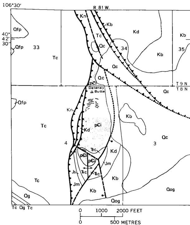
FIGURE 3.—Generalized geologic map showing the distribution of fluor spar in the vicinity of Delaney Butte, Jackson County, Modified from Hail (1965).
