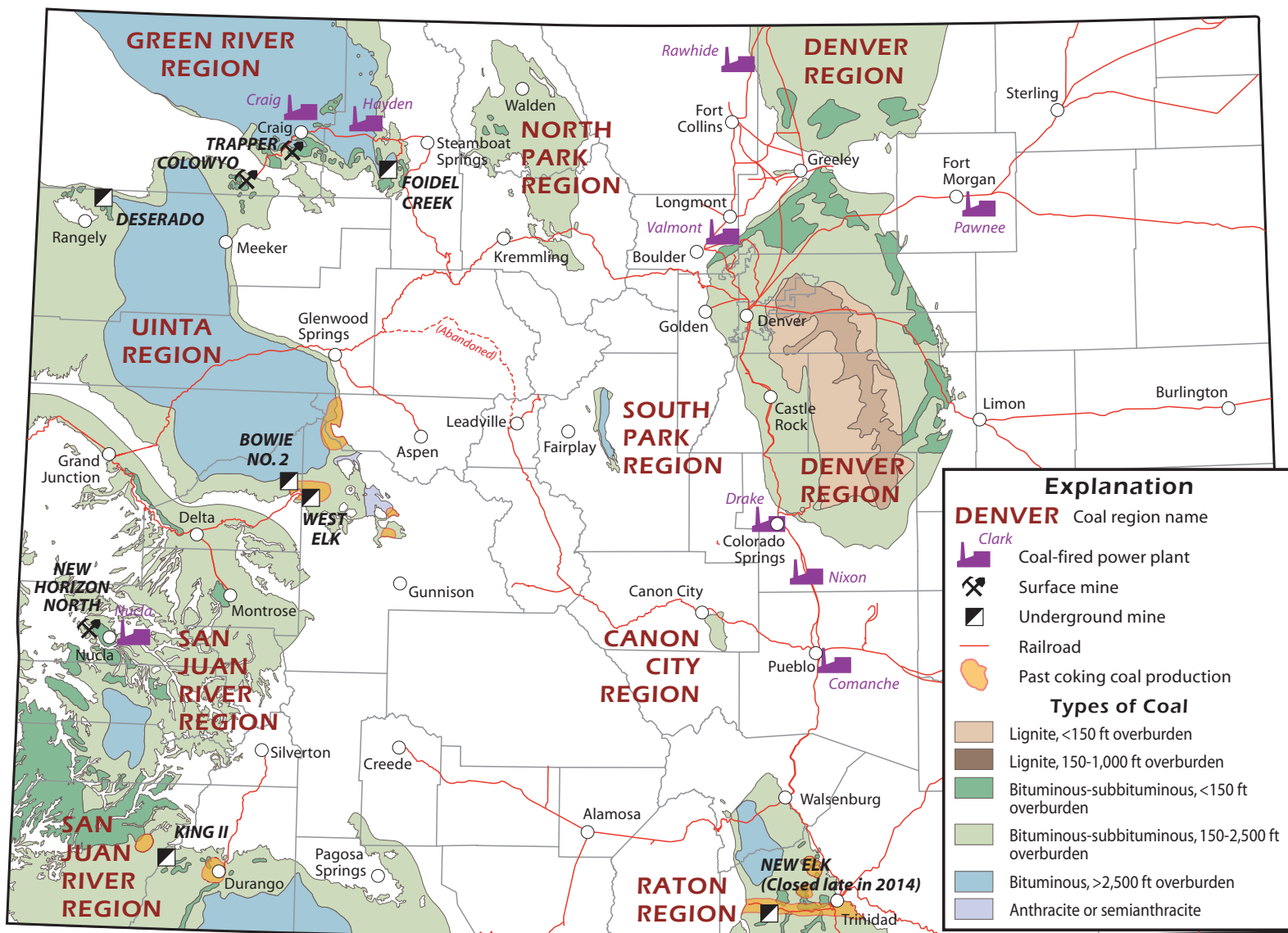
Figure 2-16. Locations of active coal mines, power plants, railroads, and coal-bearing regions in Colorado, 2014.
