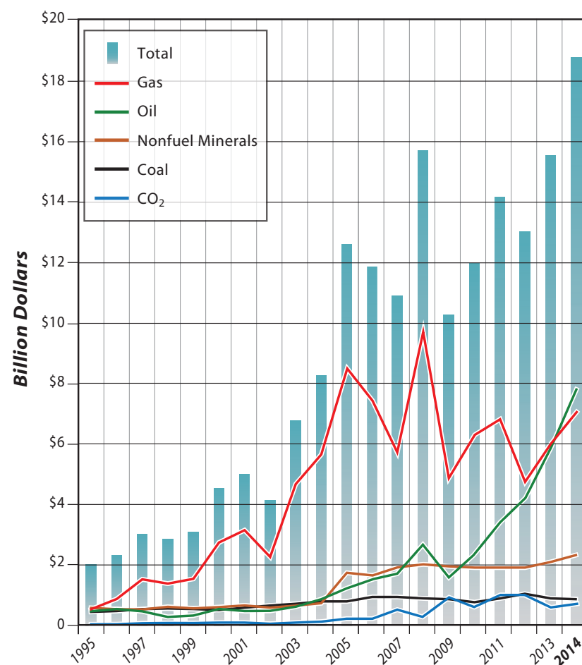
Figure ES-2. Mineral and energy fuel production value in Colorado, 1995–2014.
