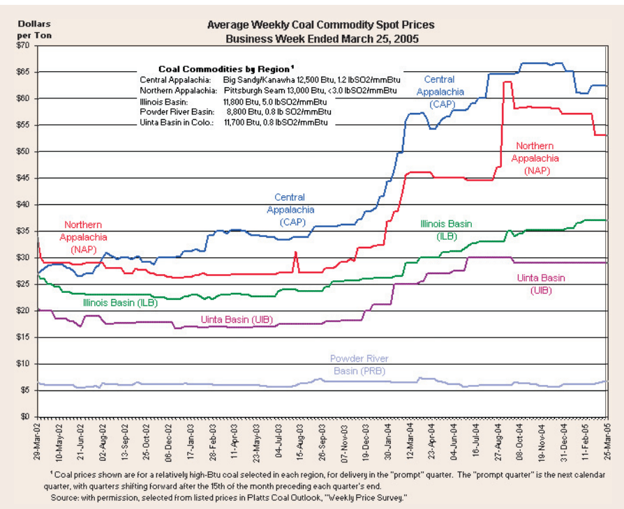
Figure 30. Spot sales price for domestic coal by region and type. Source: EIA 2005.
