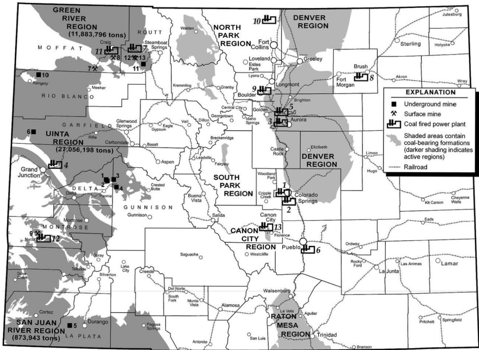
Figure 31. Locations of coal mines, power plants, railroads, and coal-bearing regions in Colorado, 2004. See table 5 for mine information, and table 8 for power plant names.
