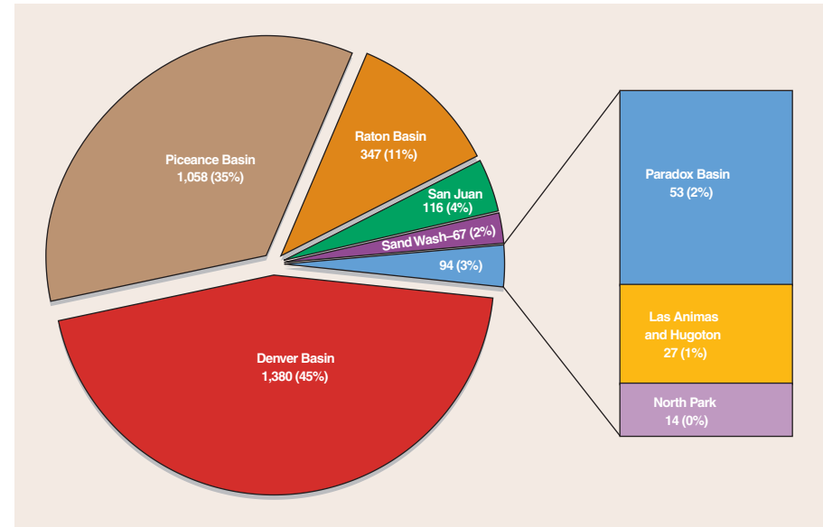
Figure 21: Basin distribution in approved applications for permit to drill in 2004, (COGCC).
