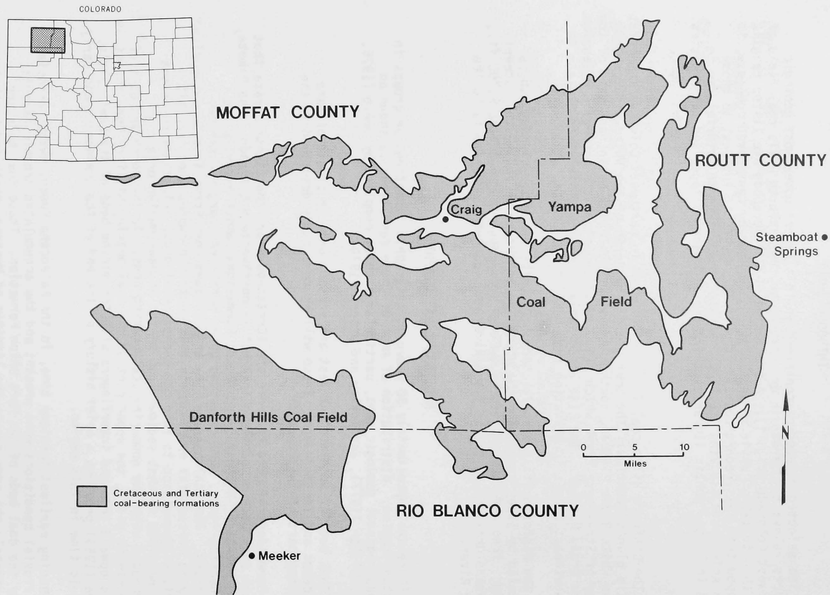
Figure 1. Location map showing the Danforth Hills Coal Field and adjacent coal field in northwestern Colorado (from Brownfield and Johnson, 1984).
