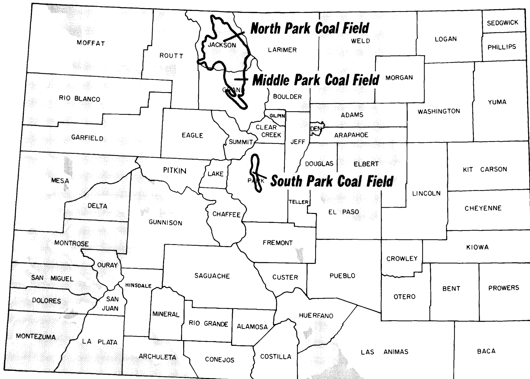
Figure 1. Index map of the North Park, Middle Park, and South Park Coal Fields, Colorado.
