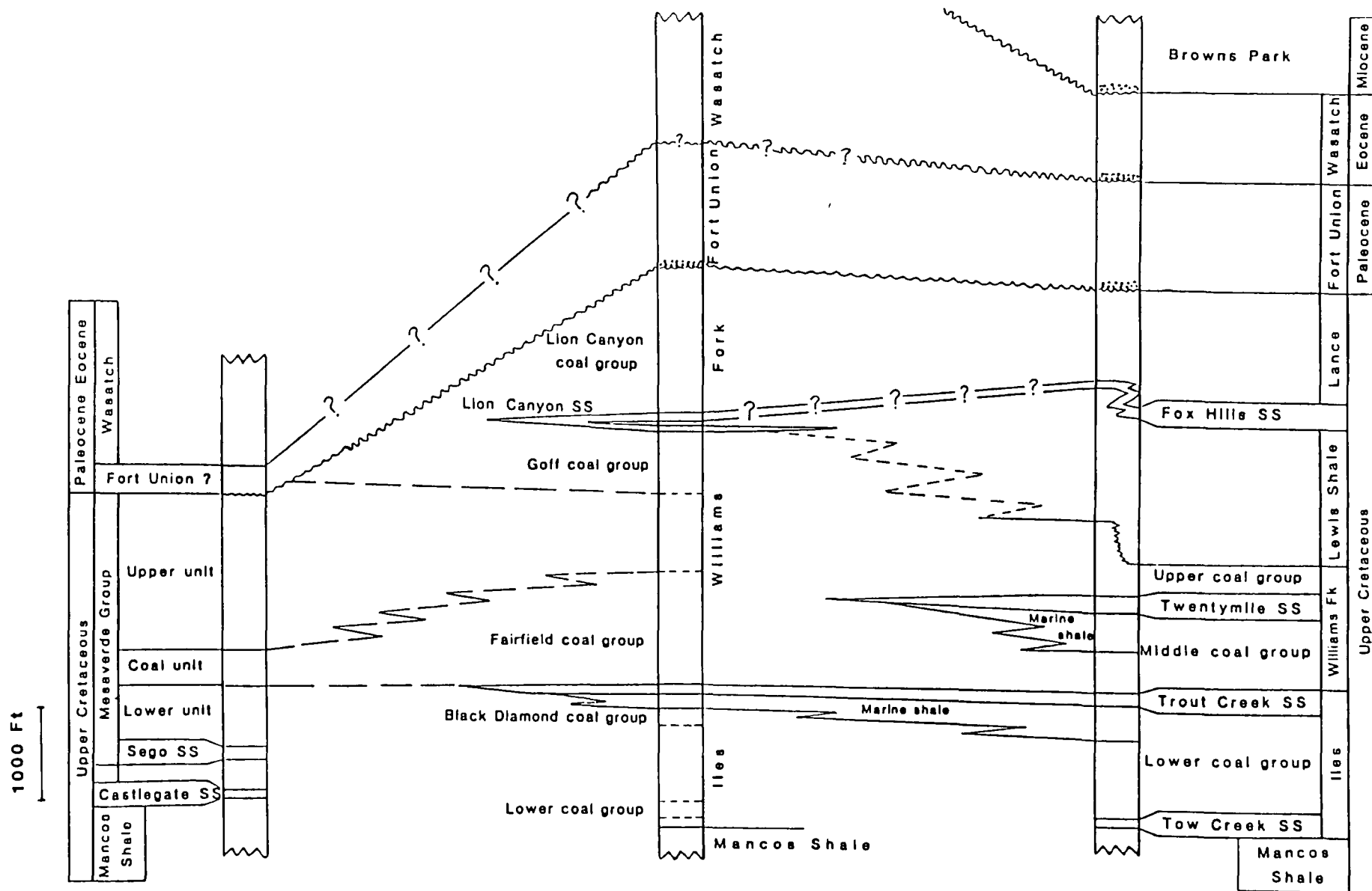
Figure 2. Generalized stratigraphic sections of the coal-bearing formations of northwestern Colorado (from Johnson and Brownfield, 1984).
