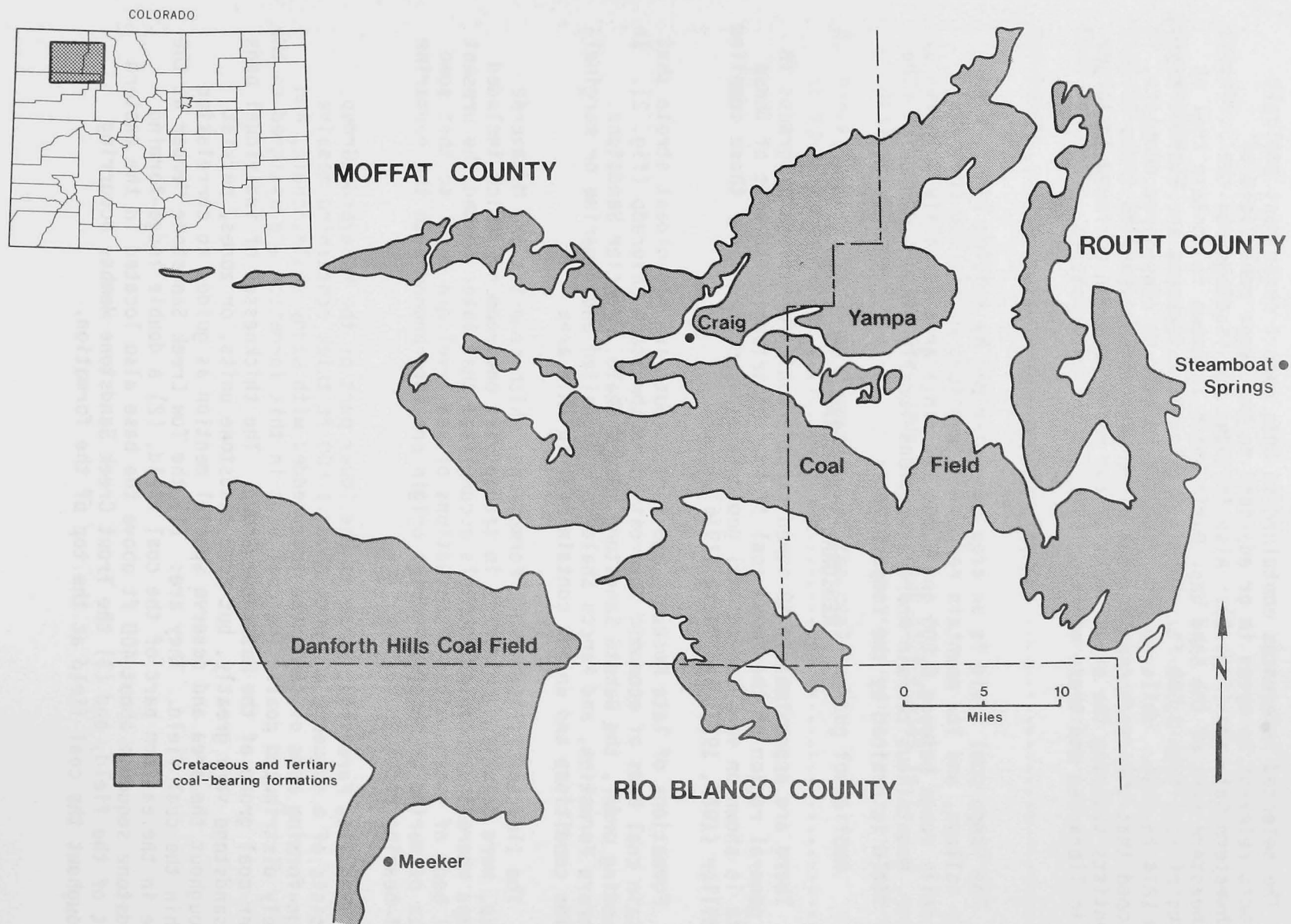
Figure 1. Location map showing the Yampa and adjacent coal field in northwestern Colorado (from Johnson and Brownfield, 1984).
