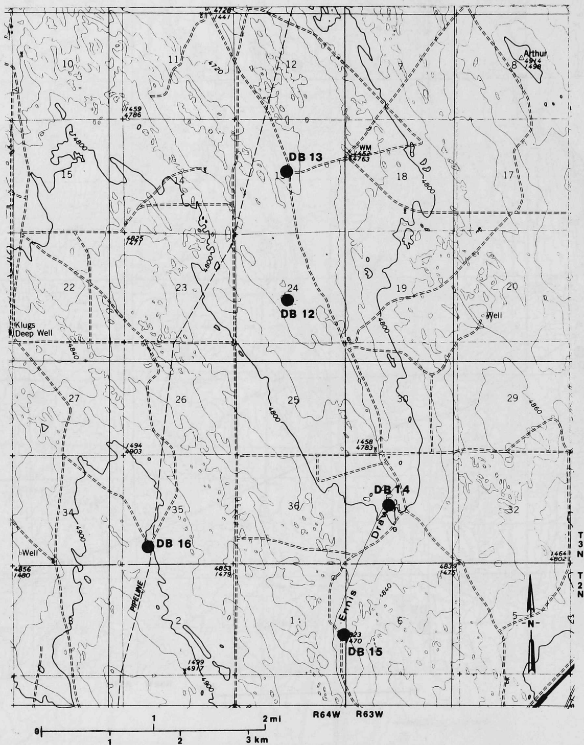
Figure 4. Location of sampled water wells in the Keenesburg area.
