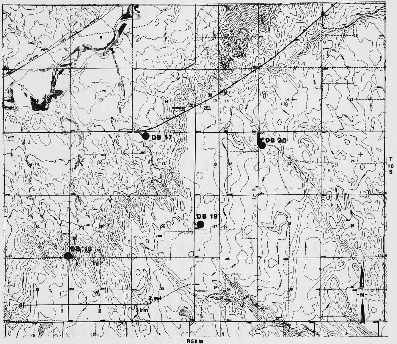
Figure 5. Location of sampled water wells in the Matheson area.
