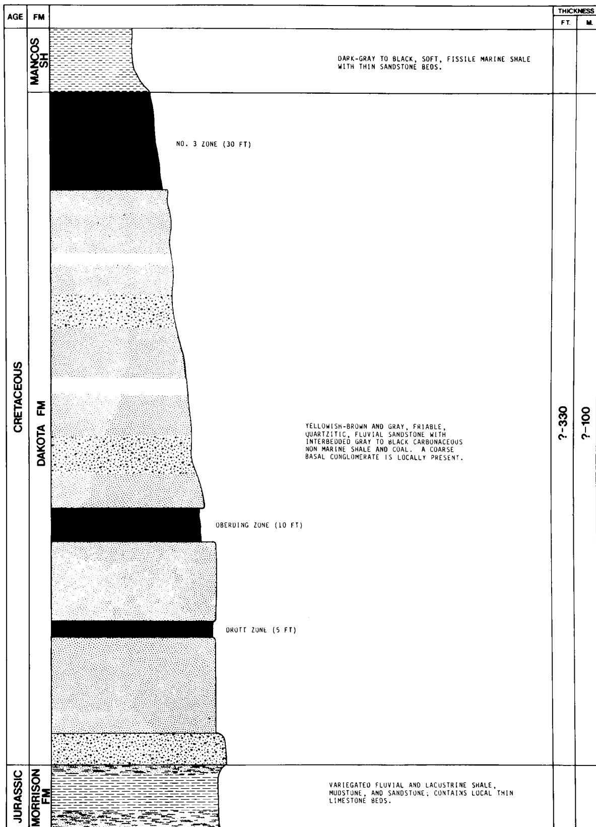
Figure E4. Generalized stratigraphic section of coal-bearing rocks in the San Juan River Region, Nucla/Naturita field. Coal zones shown in black (after Boreck and Murray, 1978; Hornbaker and others, 1976; Williams, 1964).
