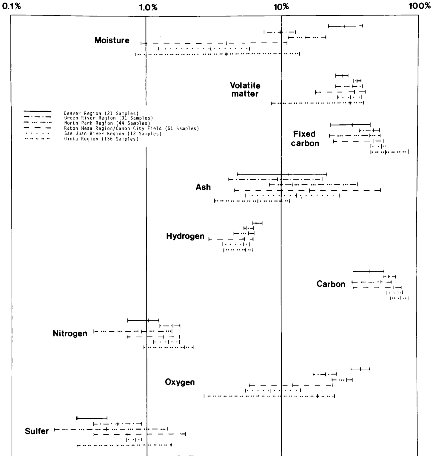
Figure 4. Arithmetic means and ranges for the proximate analyses and ultimate analyses for coal samples from the Denver, Green River, North Park, Raton Mesa (plus Canon City field), San Juan River, and Uinta Regions.
