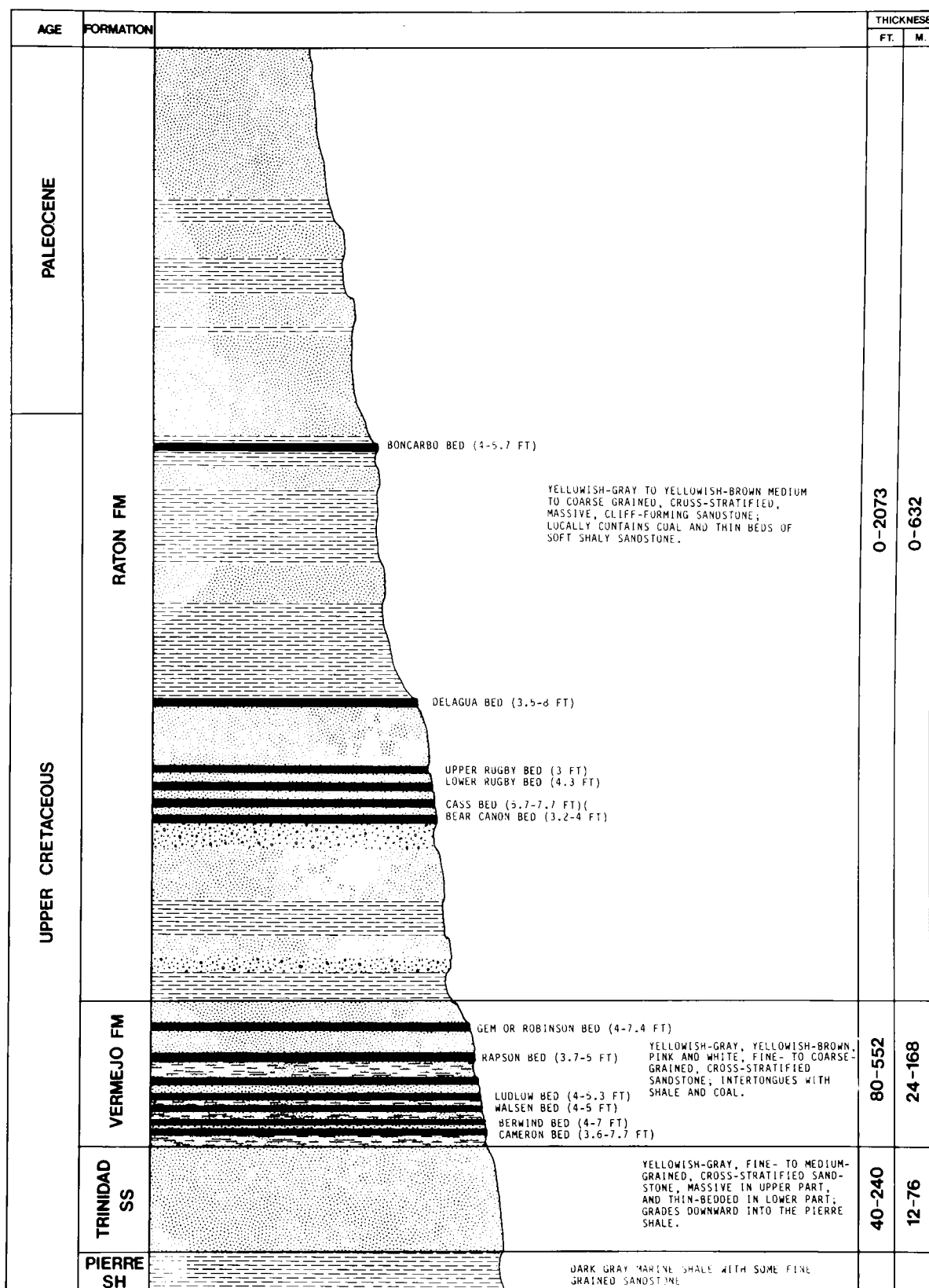
Figure D3. Generalized stratigraphic section of coal-bearing rocks in the Raton Mesa Region, Trinidad field. Coal beds shown in black (after Boreck and Murray, 1979; Harbour and Dixon, 1959; Hornbaker and others, 1976; Johnson, 1969; Wood and others, 1957).
