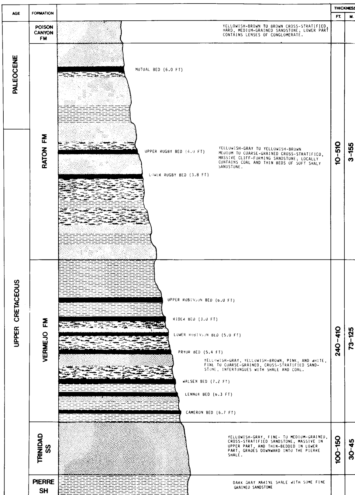
Figure D4. Generalized stratigraphic section of coal-bearing rocks in the Walsenburg field Raton Mesa Region. Coal beds shown in black (after Boreck and Murray, 1979; Hornbaker and others, 1976; Johnson, 1969; Scott and Taylor, 1974).
