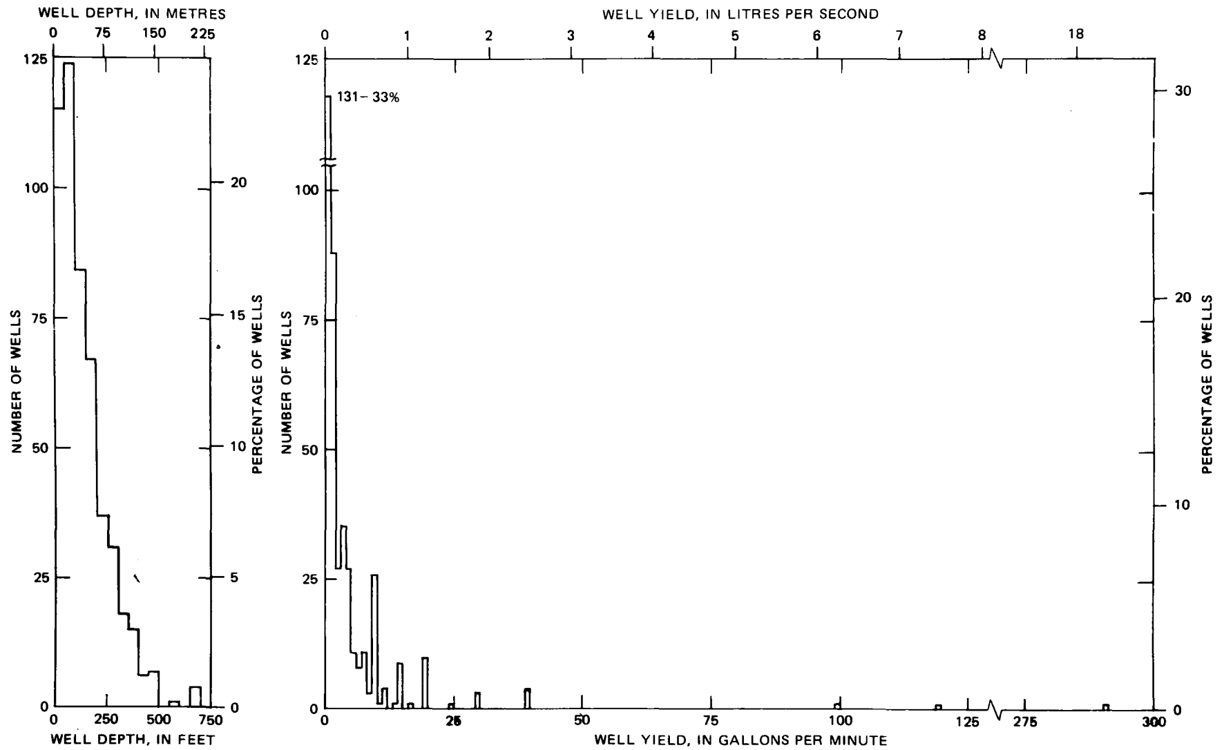
Figure 31.--Reported depths and yields for sampled wells.
