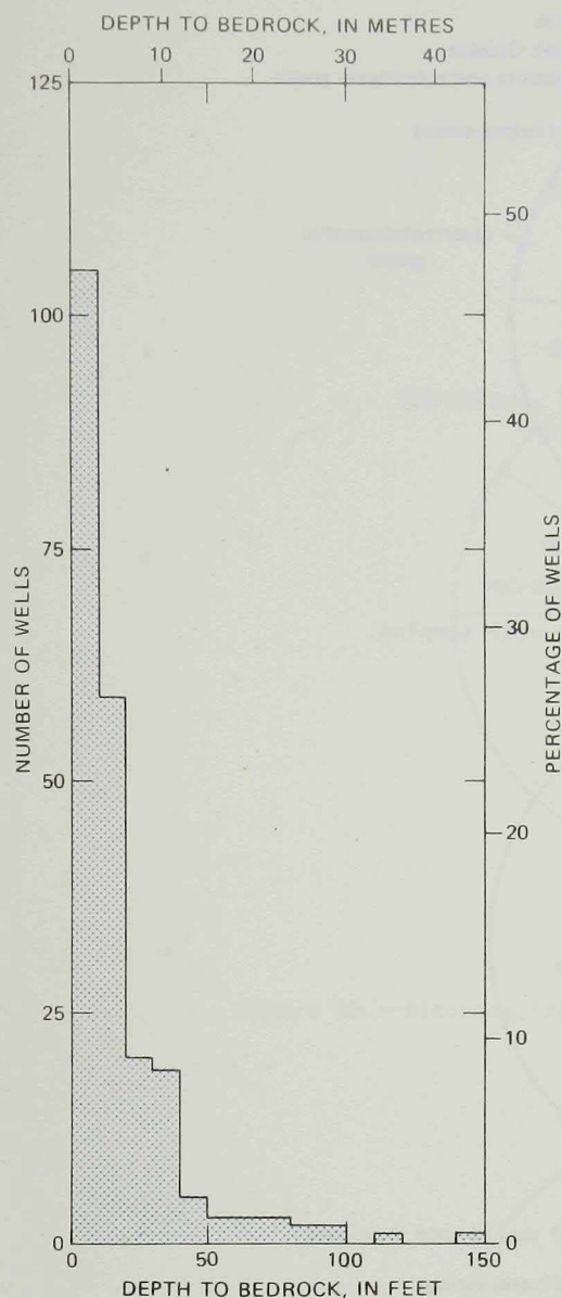
Figure 32.--Reported depths to bedrock for sampled wells.
