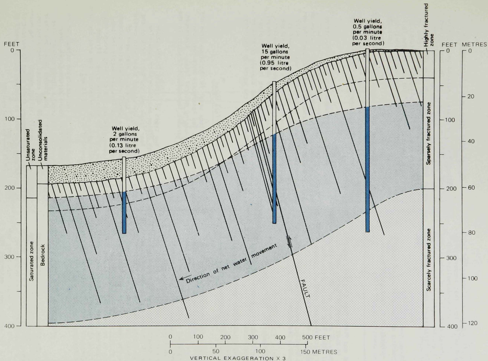
Figure 9.--Idealized one-joint fracture system and relation to ground-water yield.
