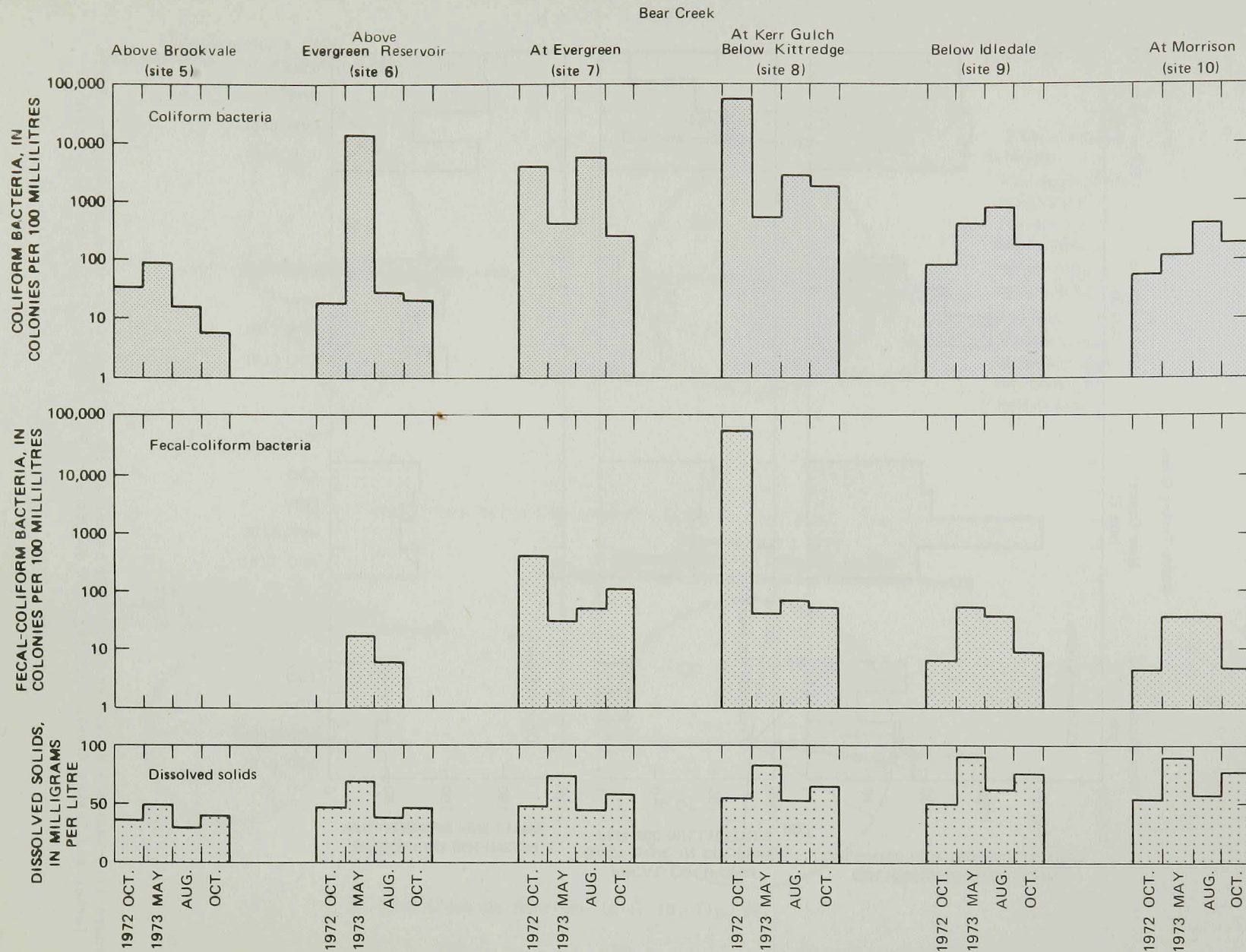
Figure 18.--Seasonal dissolved solids and bacterial concentrations for water samples from Bear Creek, October 1972 to October 1973 (see fig. 6 for location of sites).
