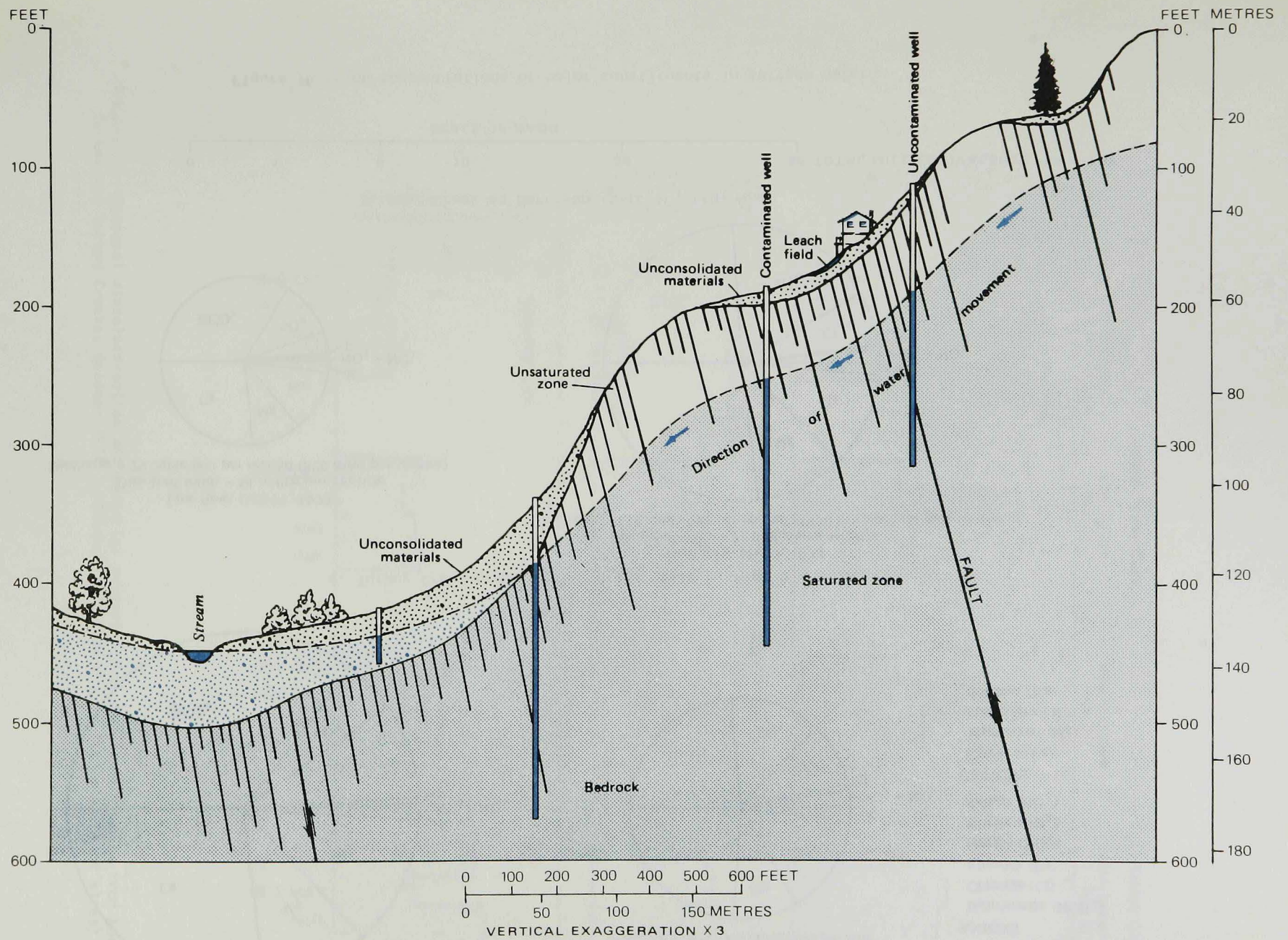
Figure 15.--Degradation of ground water resulting from leach-field effluent.
