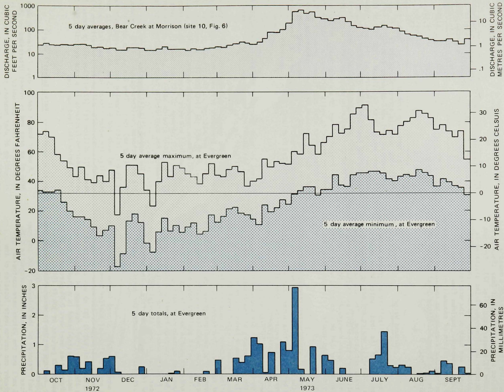
Figure 12.--Flow of Bear Creek at Morrison, and temperature and precipitation at Evergreen, for the 1973 water year. (Climatological data from the U.S. Environmental Data Service, 1972-73.)
