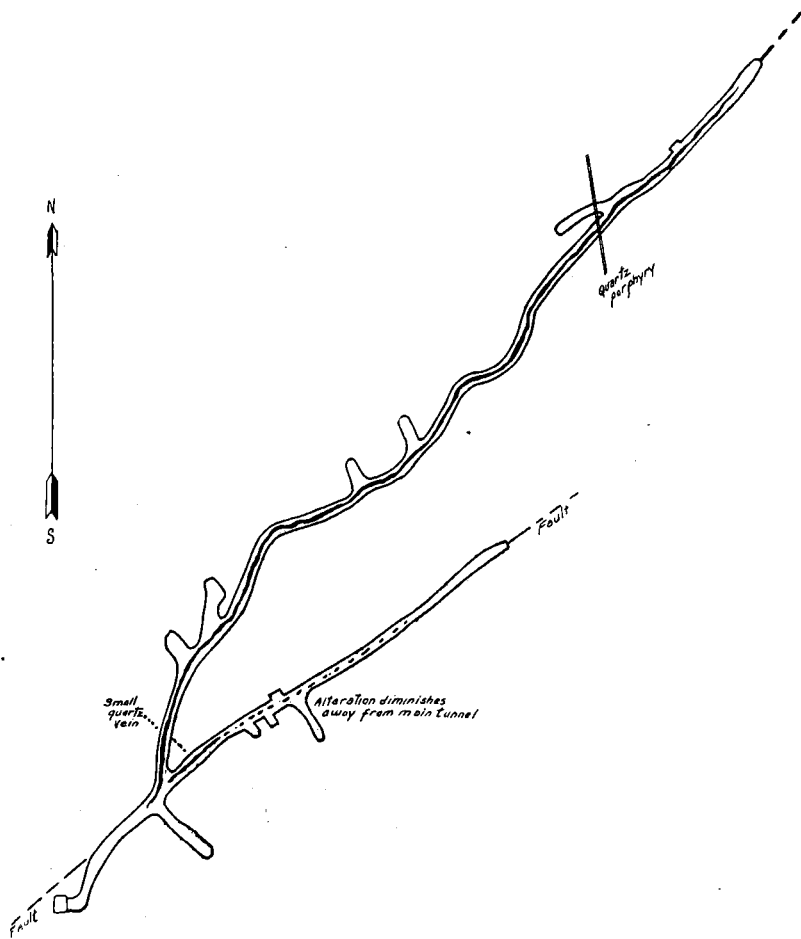
Horizontal plan of intermediate level. Mount Champion mine.
