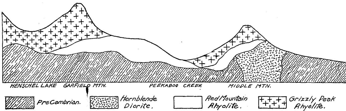
Fig. 15a. Northwest-Southeast section across Peekaboo Creek, at Henschel Lake, showing probable geologic conditions.
