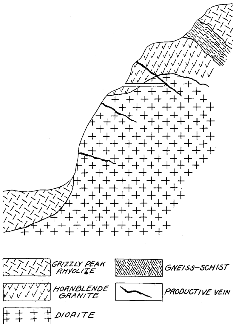
Fig. 15. Geologic cross section through Middle Mountain.
