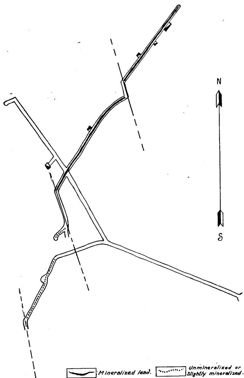
Fig. 20. Plan of workings, Eureka mine.
