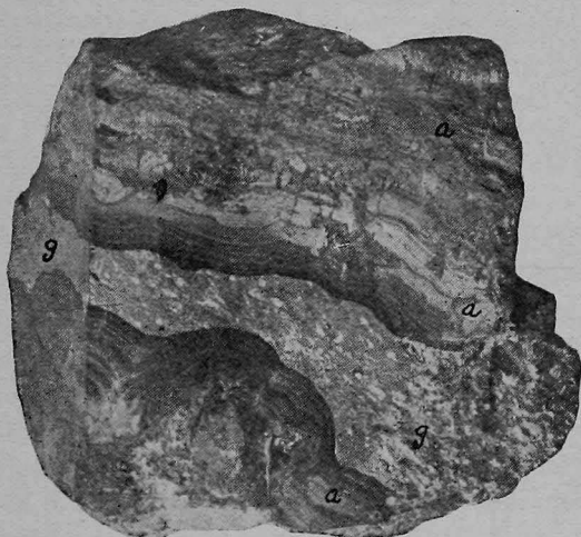
Fig. 25. Fragment of ore from one of the upper levels of the Gordon mine. Shows galena (g) altering to anglesite (a).
