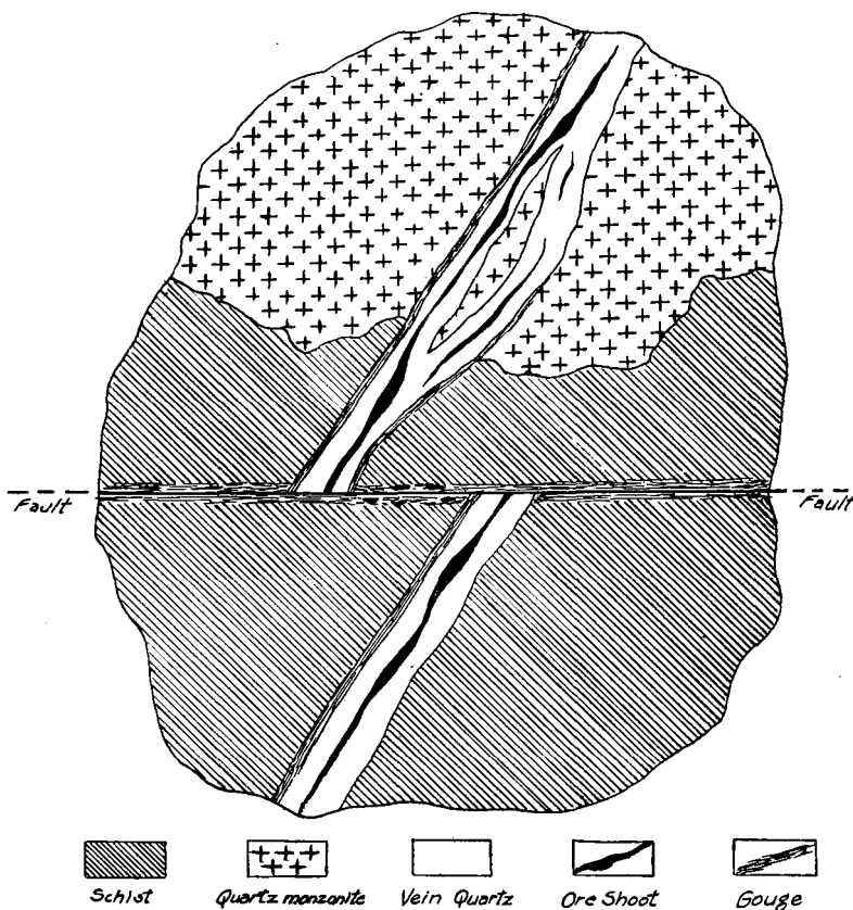
Fig. 21. Ideal cross section of Eureka vein.
