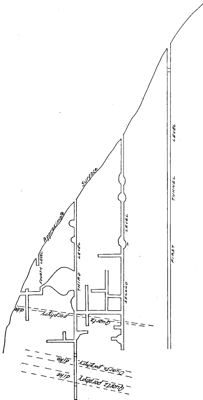
Fig. 24. Vertical section along the vein. Gordon mine.
