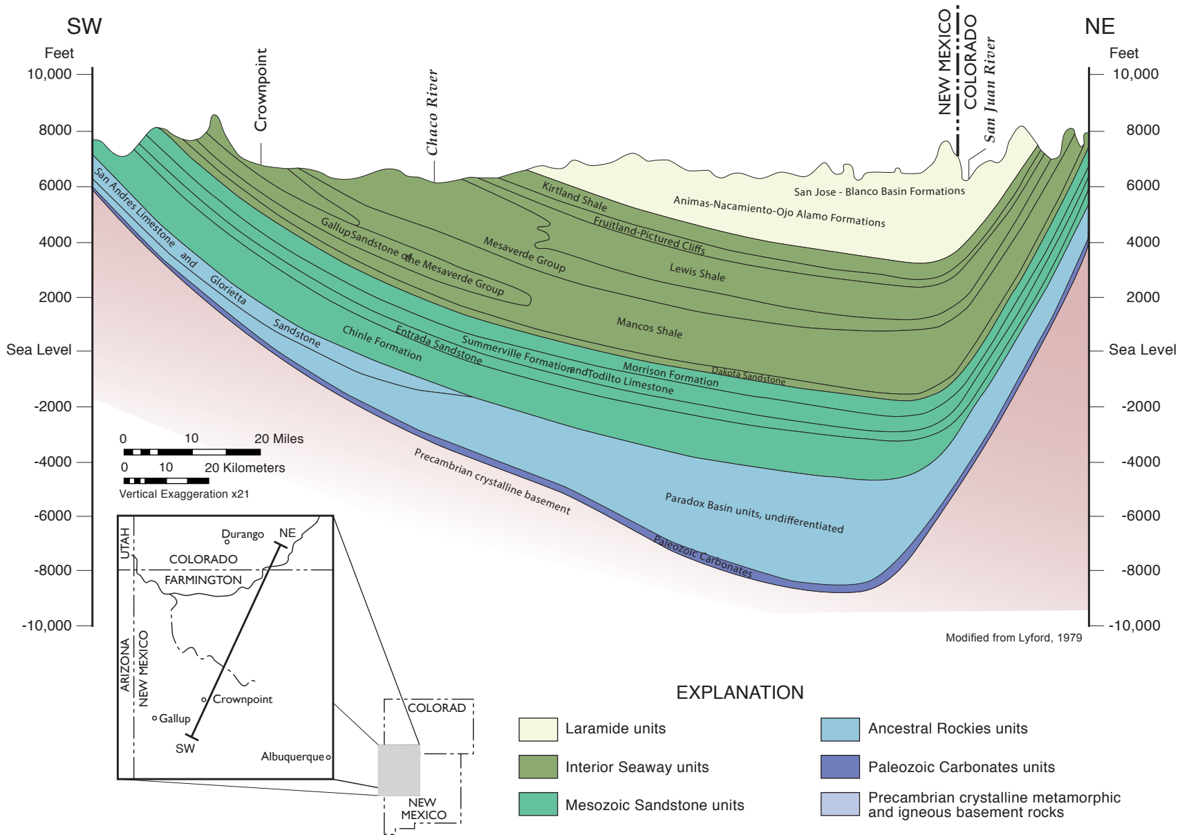
Figure 11b-02-04-02. Generalized cross section of the San Juan Basin. Modified from Lyford, 1979. Colorado Geological Survey ON-010 Colorado Groundwater Atlas.
