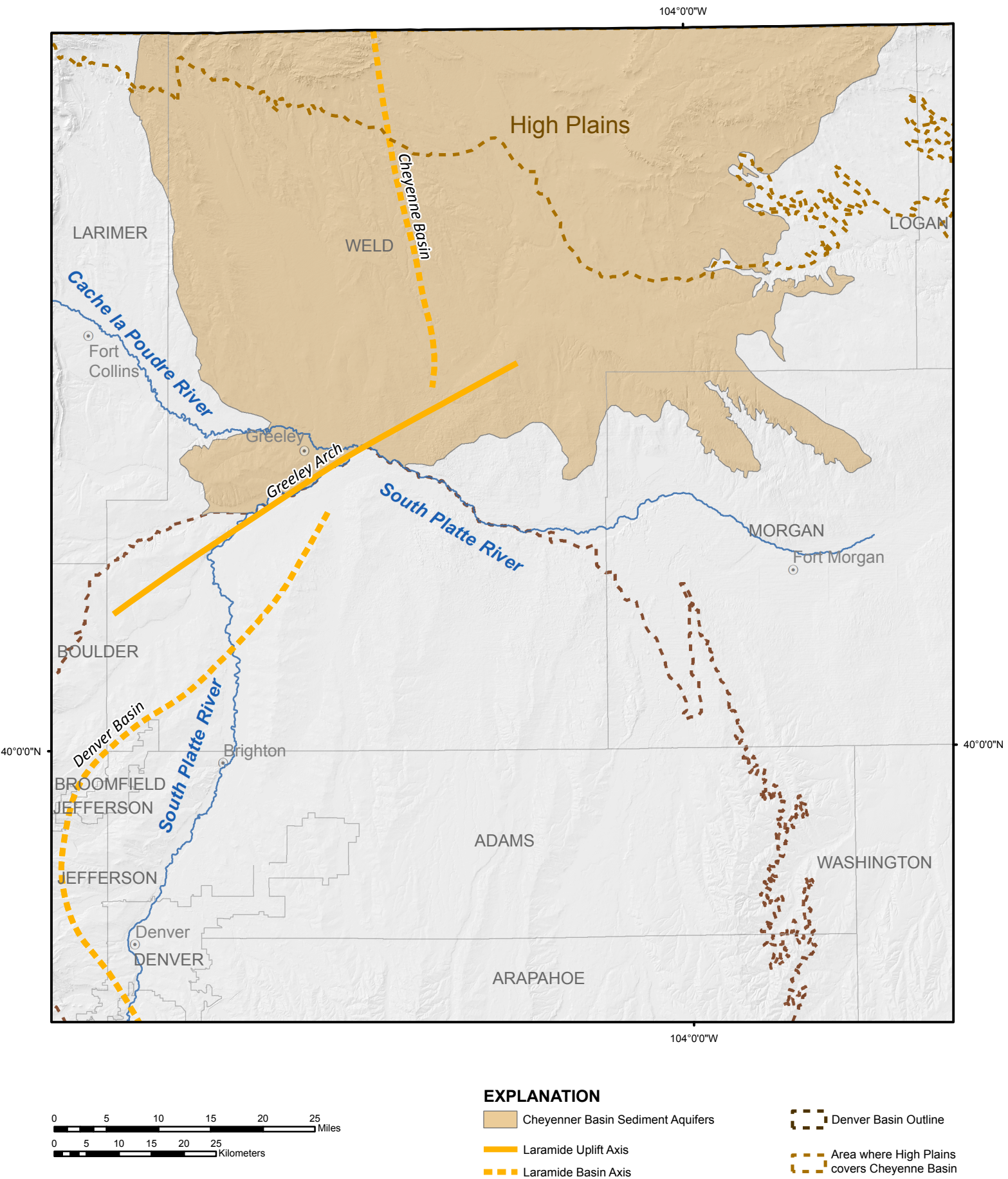
Figure 11b-02-02-01. Cheyenne Basin extent. Basin and regional boundaries modified from Tweto (1979); structural features from Hemborg (1996). Colorado Geological Survey ON-010 Colorado Groundwater Atlas.
