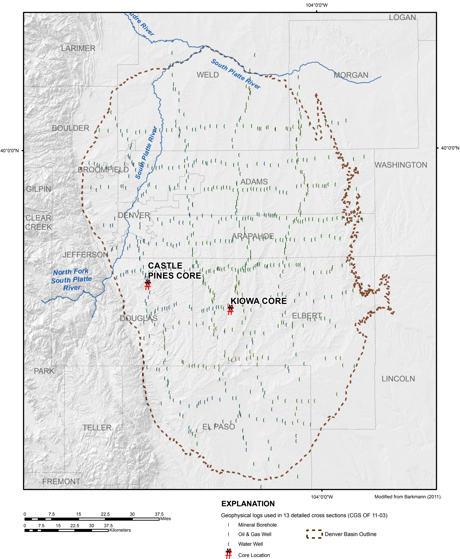
Figure 11b-02-01-02. Denver Basin core hole and cross section geophysical log locations. Modified from Barkmann (2011). Colorado Geological Survey ON-010 Colorado Groundwater Atlas.
