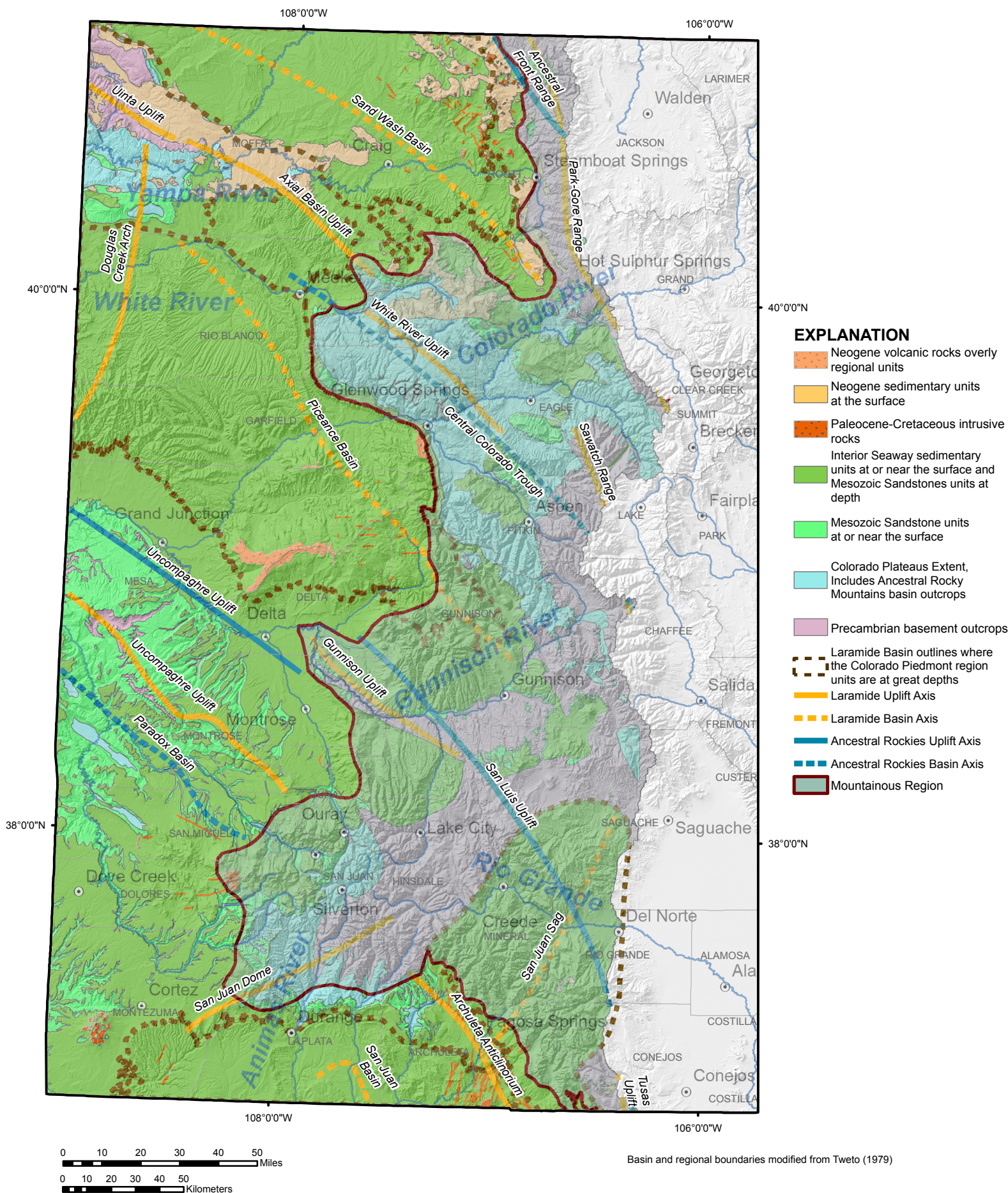
Figure 11a-03-01. Colorado Plateaus region sedimentary bedrock aquifers. Basin and regional boundaries modified from Tweto (1979). Colorado Geological Survey ON-010 Colorado Groundwater Atlas.
