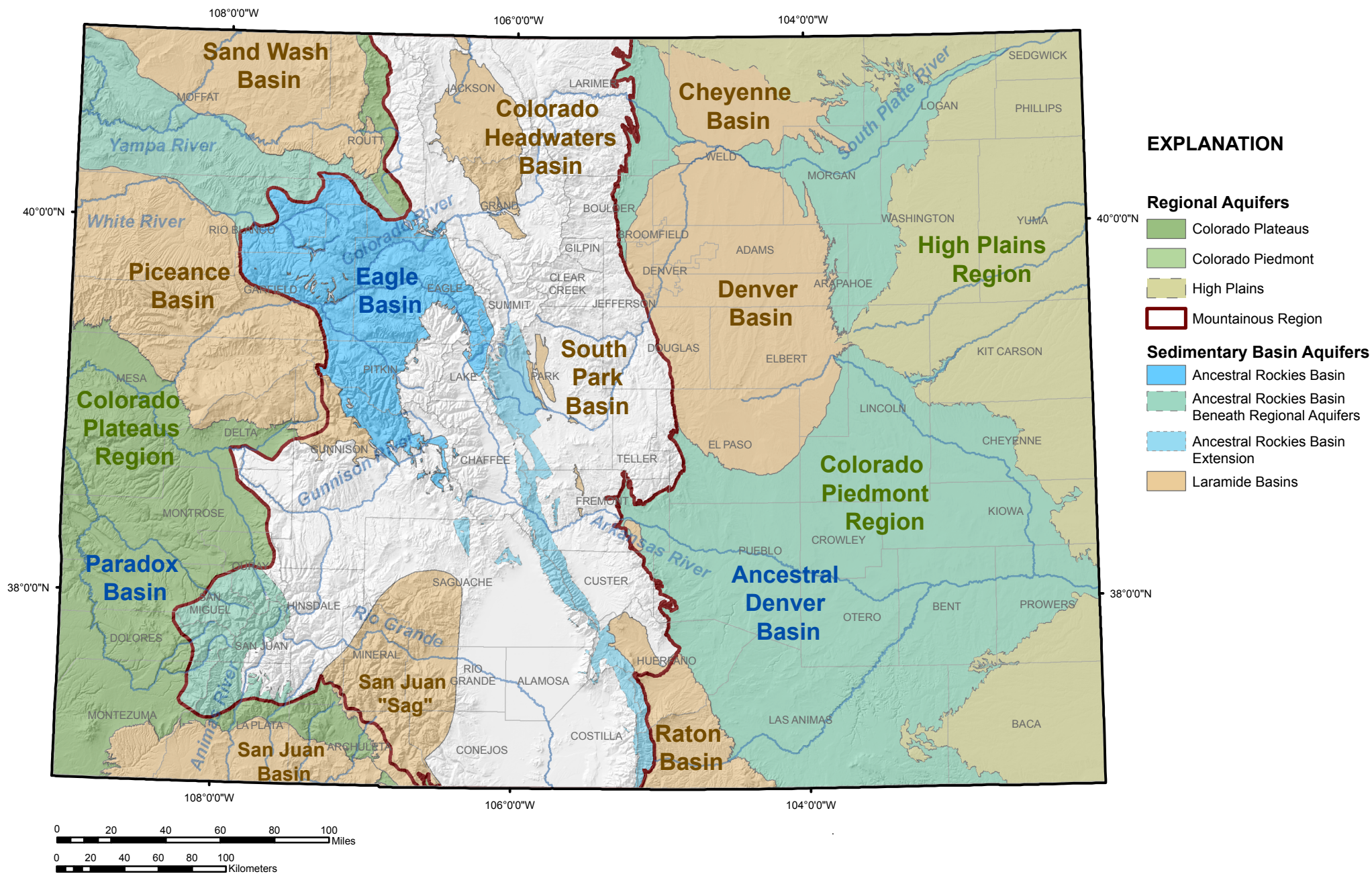
Figure 11-01. Statewide sedimentary bedrock aquifers. Basin and regional boundaries modified from Tweto (1979). Colorado Geological Survey ON-010 Colorado Groundwater Atlas.
