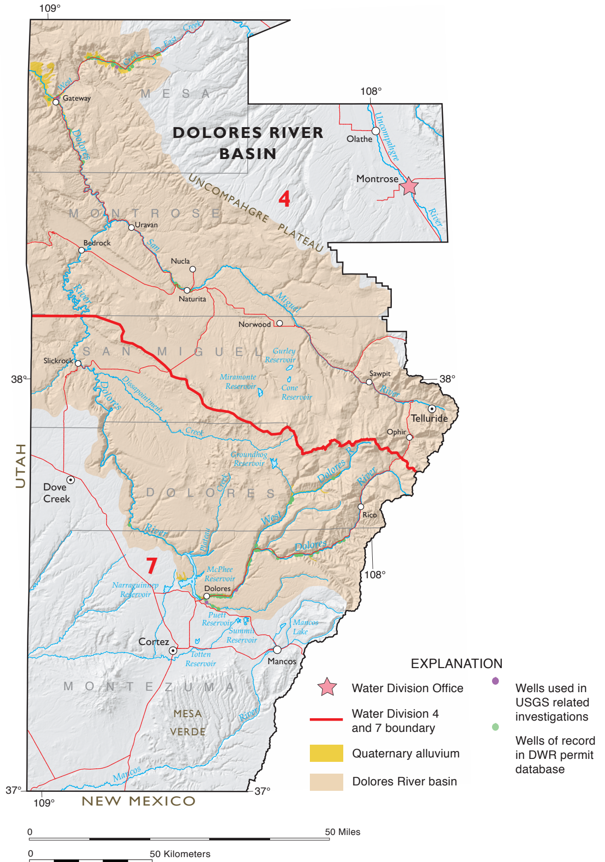
Figure 10-11-01. Dolores River Basin alluvial aquifers. Water wells from Colorado Division of Water Resources (DWR). Colorado Geological Survey ON-010 Colorado Groundwater Atlas.
