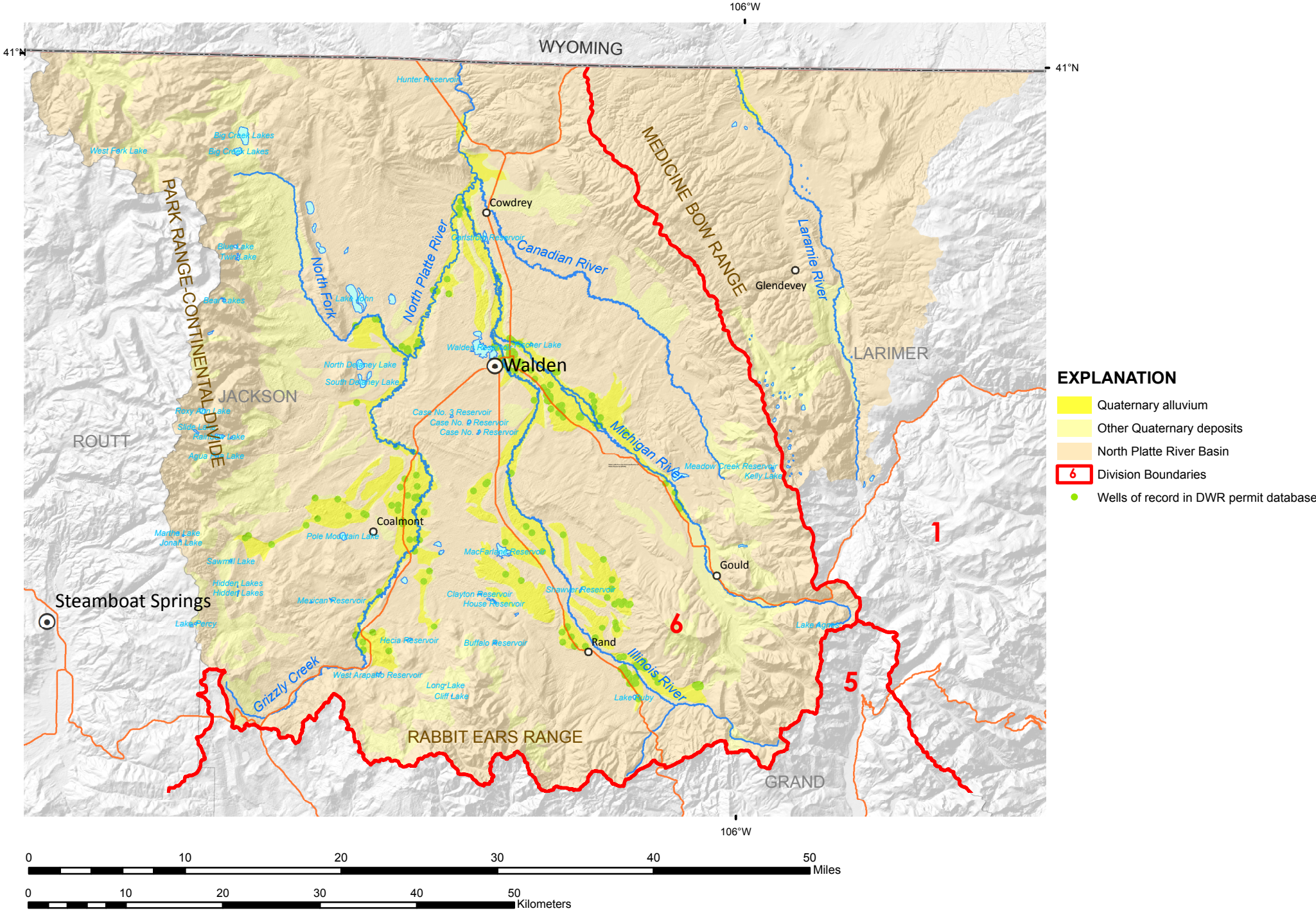
Figure 10-09-01. North Platte River Basin alluvial aquifers. Water wells from the Colorado Division of Water Resources (DWR). Colorado Geological Survey ON-010 Colorado Groundwater Atlas.
