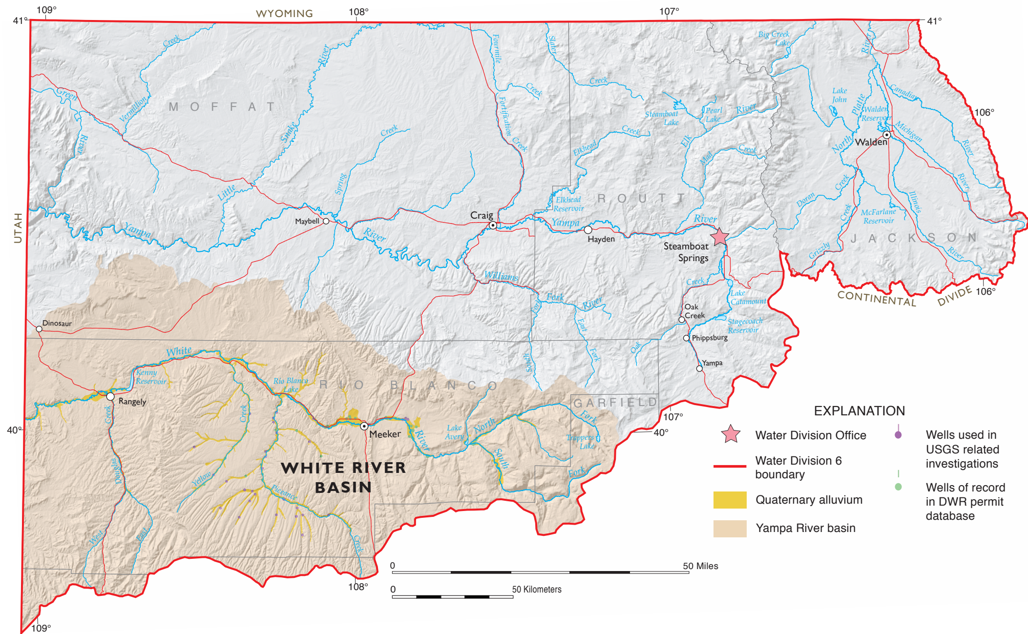
Figure 10-08-01. White River Basin alluvial aquifers. Water wells from Colorado Division of Water Resources (DWR). Colorado Geological Survey ON-010 Colorado Groundwater Atlas.
