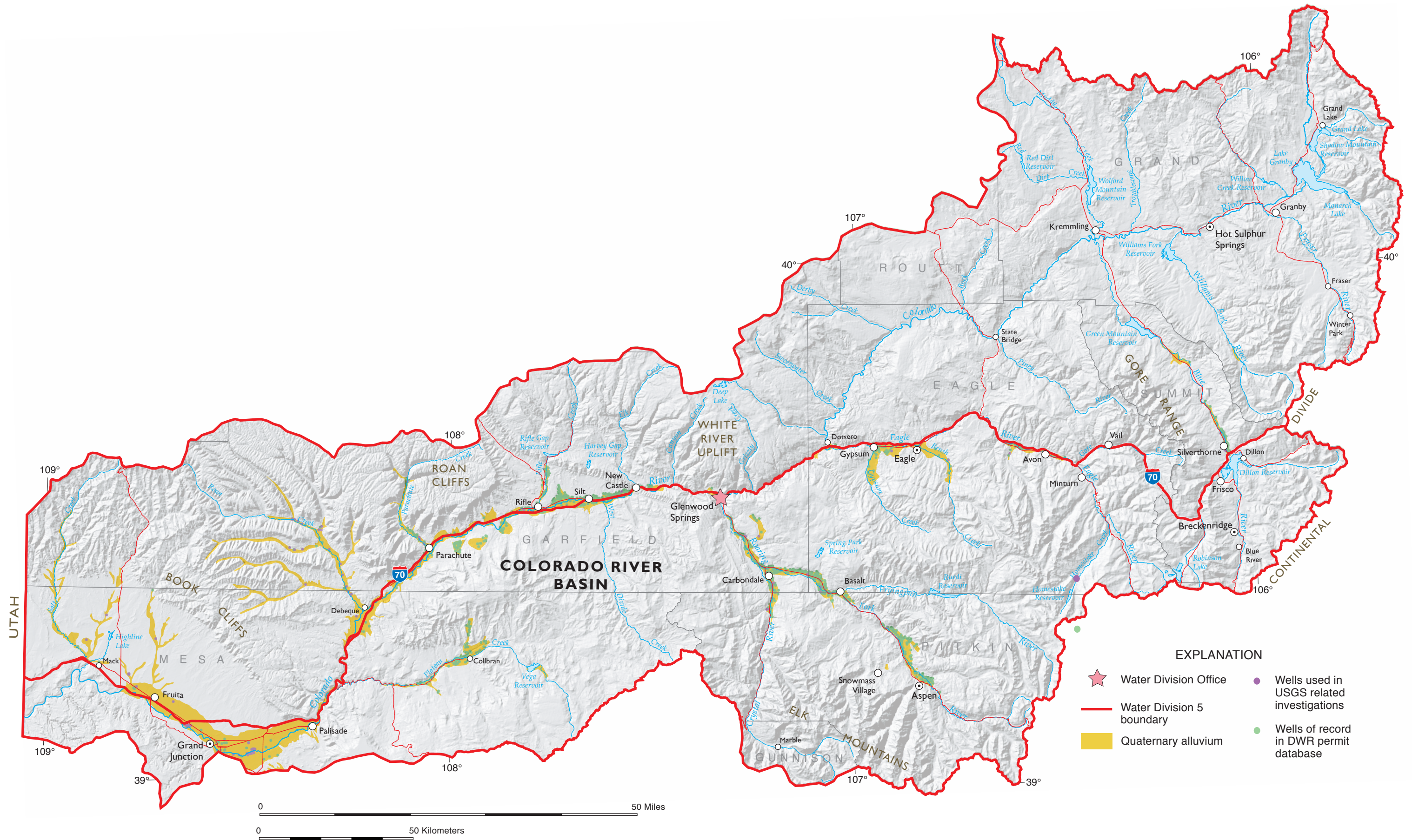
Figure 10-06-01. Colorado River Basin alluvial aquifers. Water wells from Colorado Division of Water Resources (DWR). Colorado Geological Survey ON-010 Colorado Groundwater Atlas.
