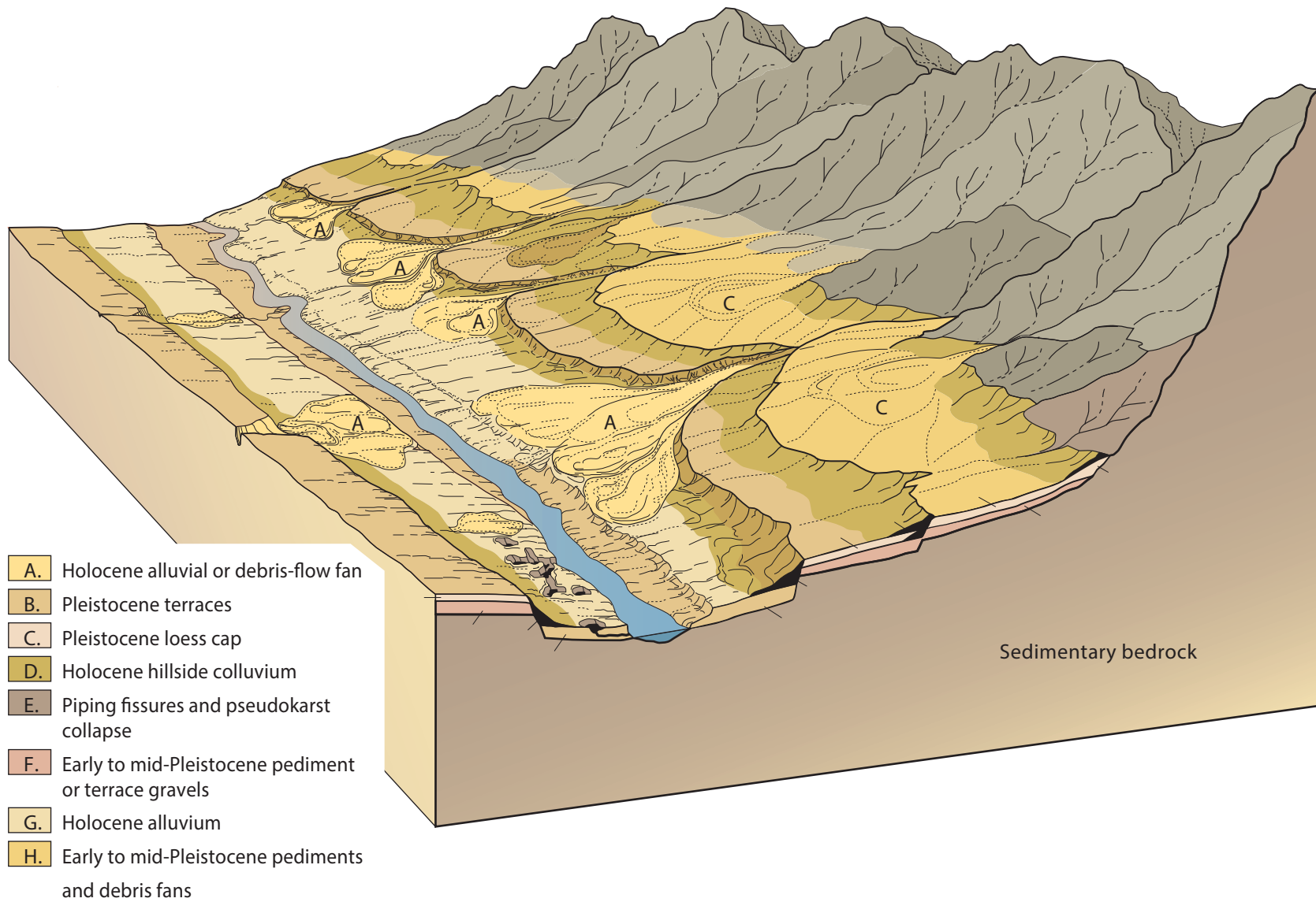
Figure 10-02. Elevations of older river terraces above modern rivers. Colorado Geological Survey ON-010 Colorado Groundwater Atlas.
