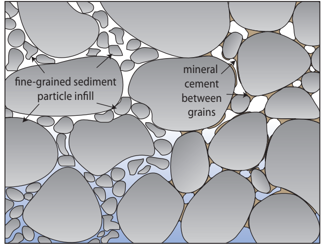
Poorly sorted, or cemented, sedimentary material (Dawson, Denver, Arapahoe aquifers)
