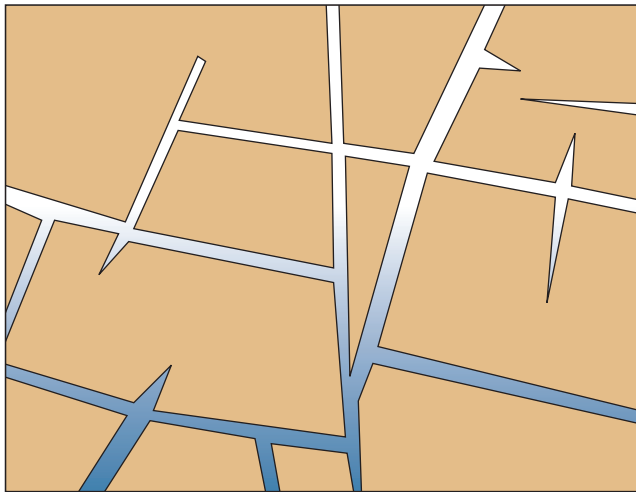
Fractured crystalline rocks (Pikes Peak Granite)
