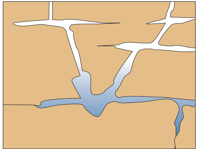
Cavernous geologic formations (Leadville Limestone)
