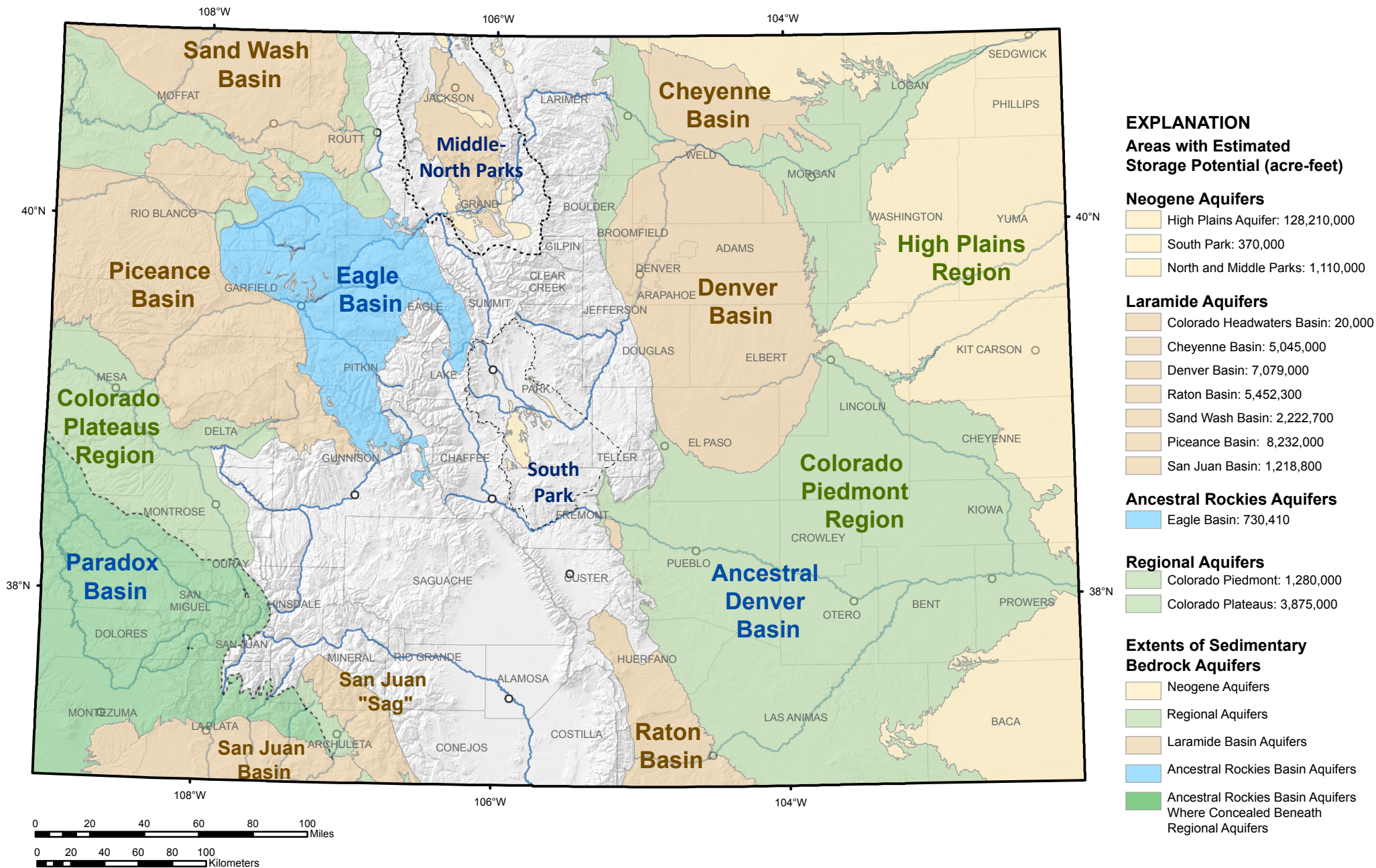
Figure 04-09. Statewide potential for underground storage in bedrock aquifers. Sites modified from Topper and others, 2004, locations approximate. Colorado Geological Survey ON-010 Colorado Groundwater Atlas.
