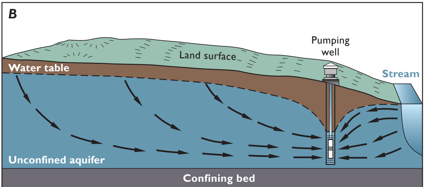
Pumping well intercepting discharge to a stream
