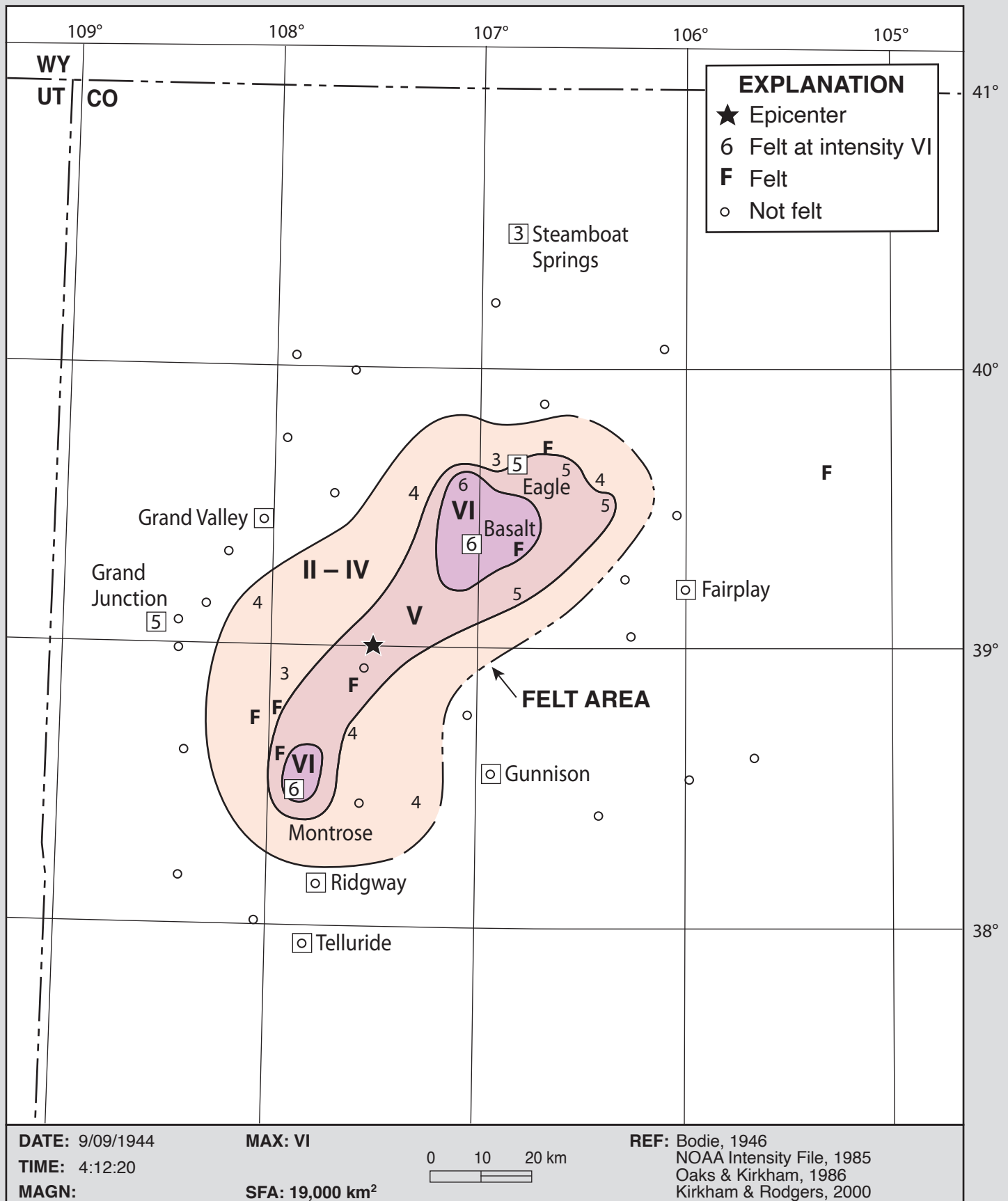
Figure 8. Isoseismal map for the Montrose-Basalt-area earthquake - 9 September 1944 - MMI VI. Kirkham, Robert M., and William P. Rogers. "Bulletin 52 - Colorado Earthquake Information, 1867-1996." Earthquake Bulletin . Denver, CO: Colorado Geological Survey, Division of Minerals and Geology, Department of Natural Resources, 2000. https://coloradogeologicalsurvey.org/publications/colorado-earthquake-information-1867-1996 .
