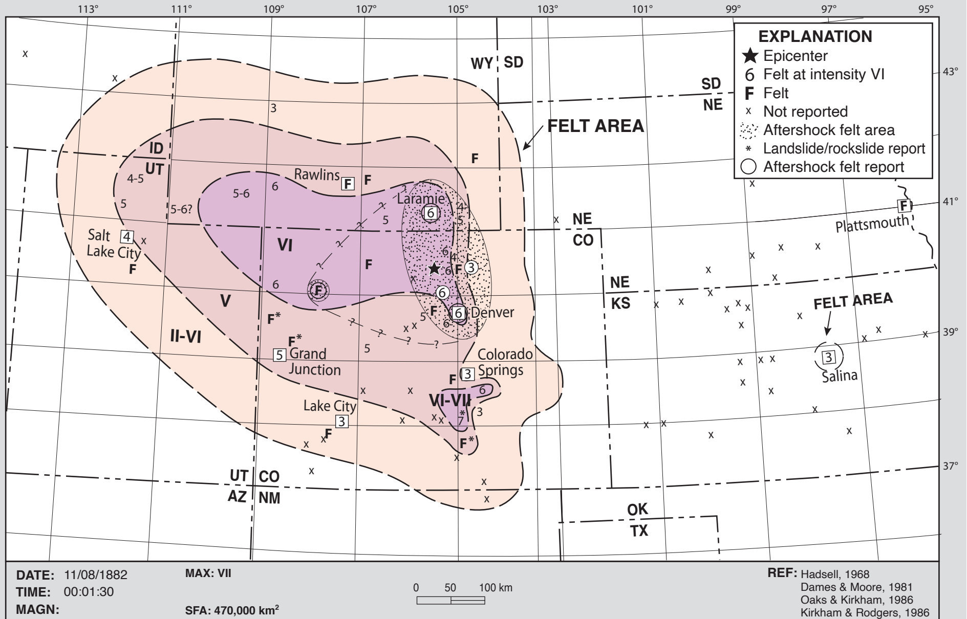
Figure 1. Isoseismal map for the north-central Colorado earthquake - 8 November 1882 - MMI VII. Kirkham, Robert M., and William P. Rogers. "Bulletin 52 - Colorado Earthquake Information, 1867-1996." Earthquake Bulletin . Denver, CO: Colorado Geological Survey, Division of Minerals and Geology, Department of Natural Resources, 2000. https://coloradogeologicalsurvey.org/publications/colorado-earthquake-information-1867-1996 .
