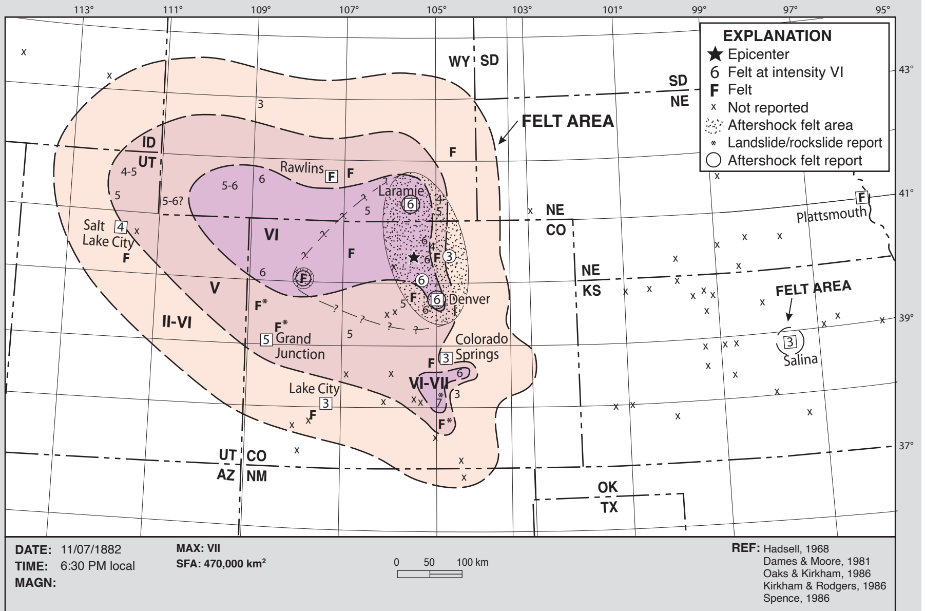
Figure I. Isoseismal map for the north-central Colorado earthquake - 7 November 1882 - MMI VII. Kirkham, Robert M., and William P. Rogers. "Bulletin 52 - Colorado Earthquake Information, 1867-1996." Earthquake Bulletin . Denver, CO: Colorado Geological Survey, Division of Minerals and Geology, Department of Natural Resources, 2000. https://coloradogeologicalsurvey.org/publications/colorado-earthquake-information-1867-1996 .
