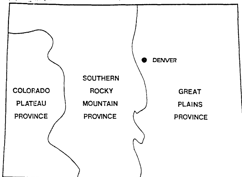
Figure 1. Heat Flow Provinces
