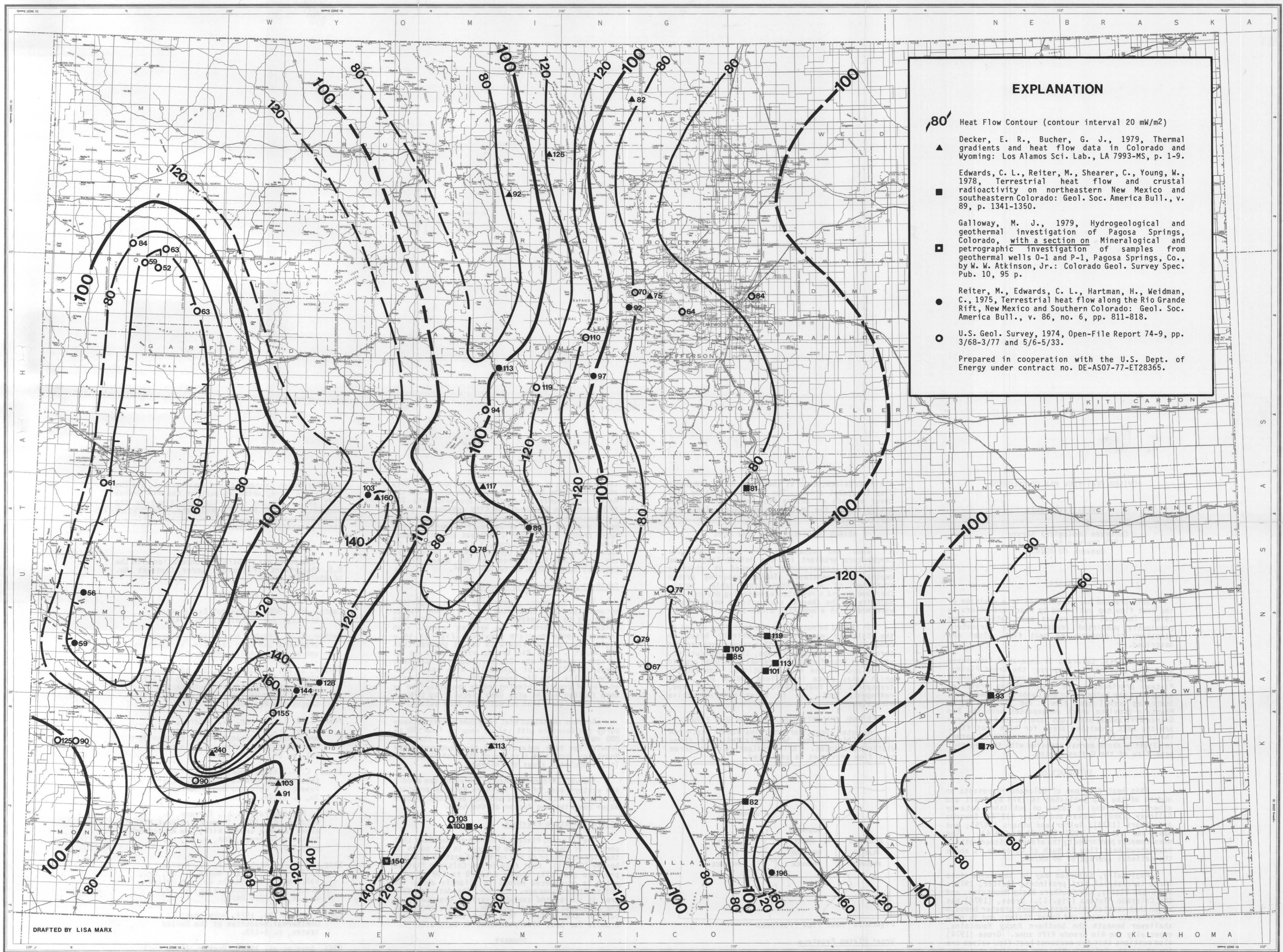
Revised Heat Flow Map of Colorado by Ted G. Zacharakis
