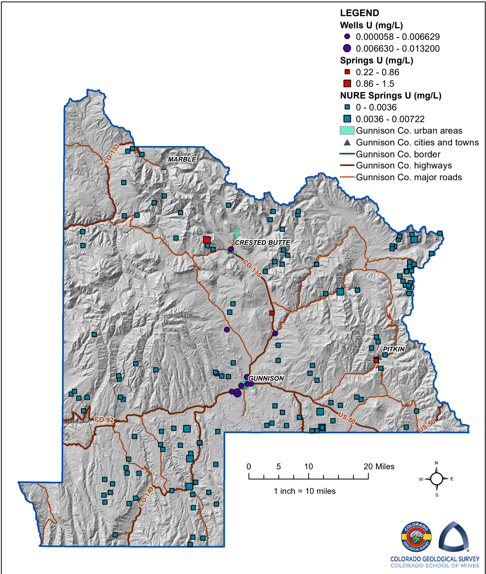
Figure 2. Historic groundwater uranium detected in wells and springs in Gunnison County, Colorado. Exceedances of the uranium 0.030 mg/L drinking water standard are shown in red. Data sources are the Water Quality Portal (WQP), the ECMC (COGCC), and NURE.
