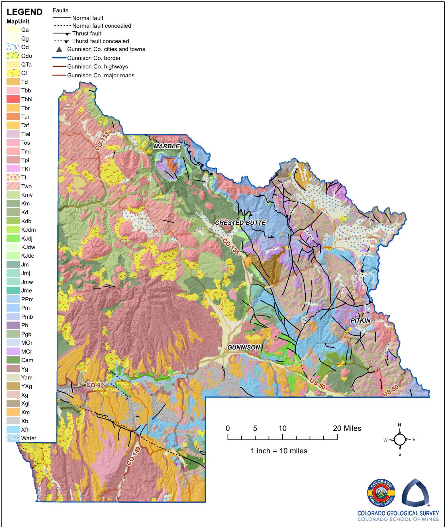
Figure 3. Compiled geologic map of Gunnison County, Colorado. From CGS Resource Series RS-37.
