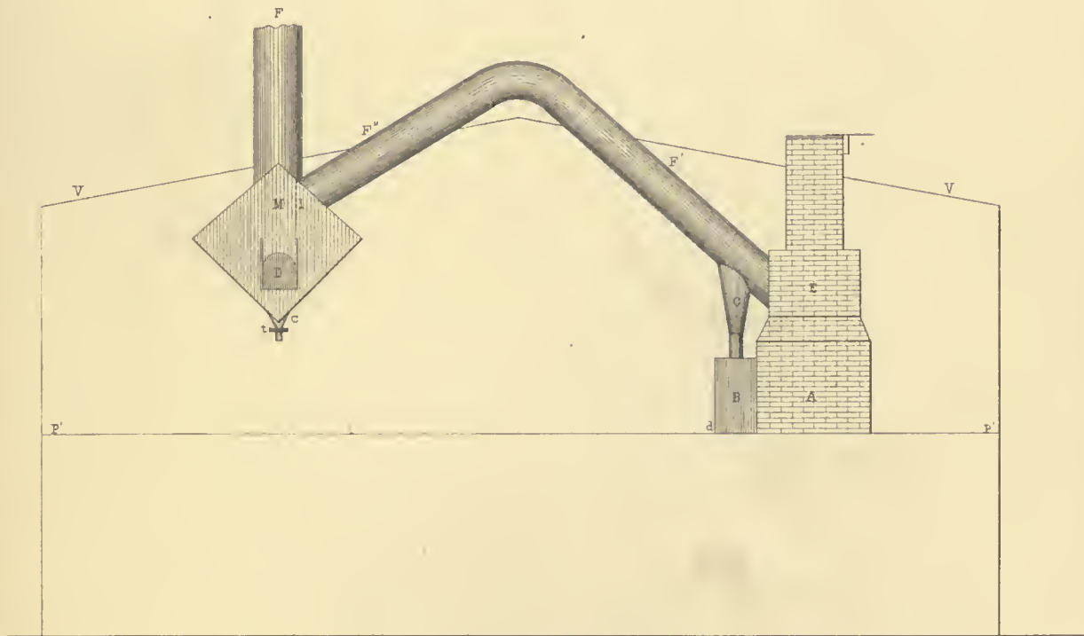
Fig. 2, FRONT ELEVATION.
