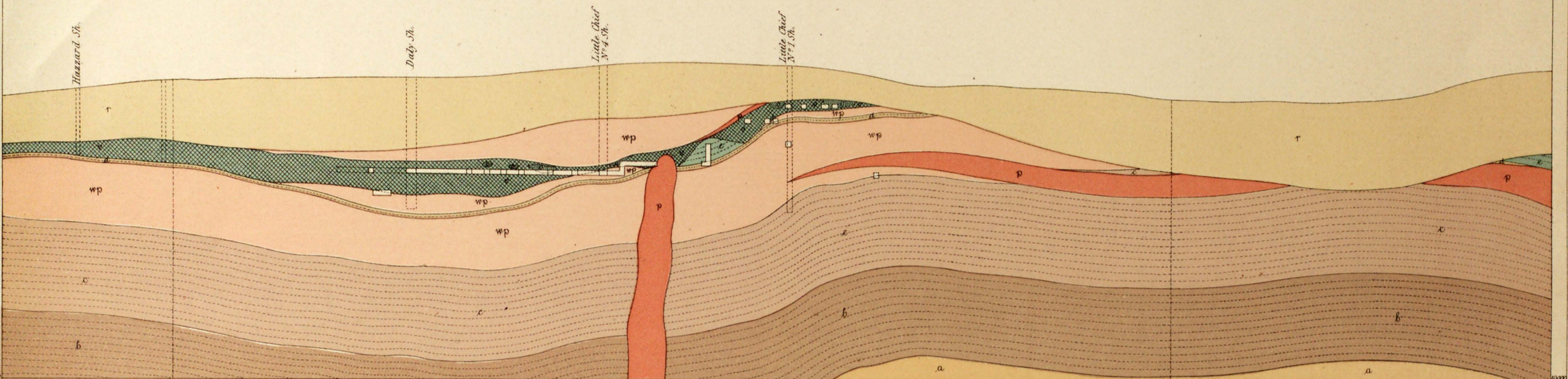
SECTION K K Through Chrysolite and New Discovery mines
