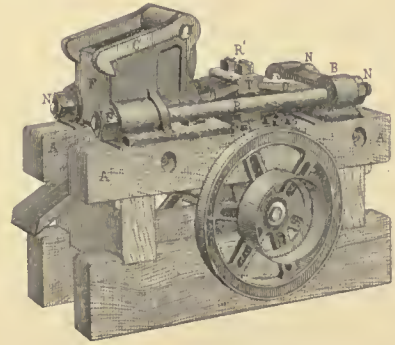
Fig. 3, PERSPECTIVE VIEW.
