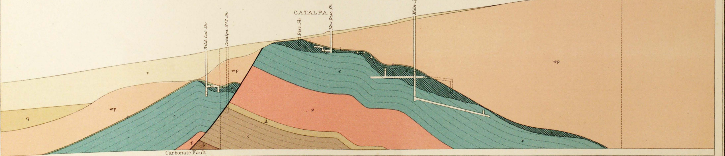
Section EE Through Catalpa Mine
