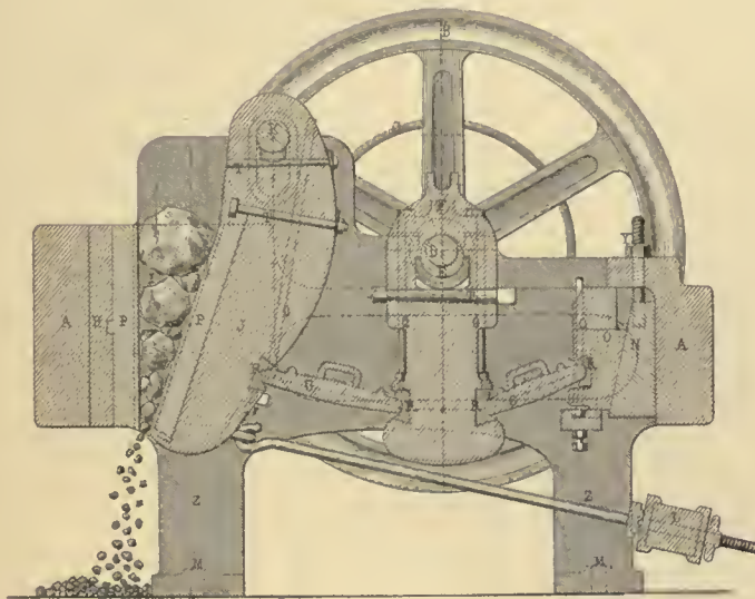
Fig. 2. SECTION ON a b.
