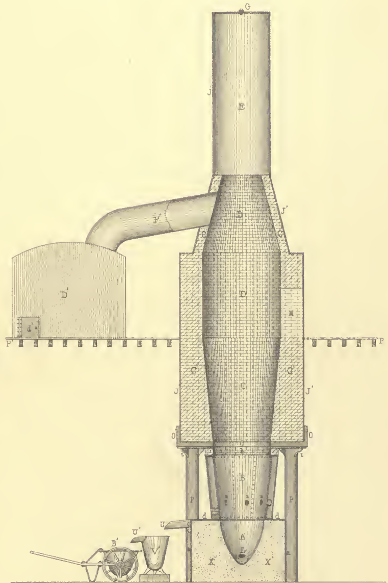
Fig. 2 SECTION ON alpha beta
