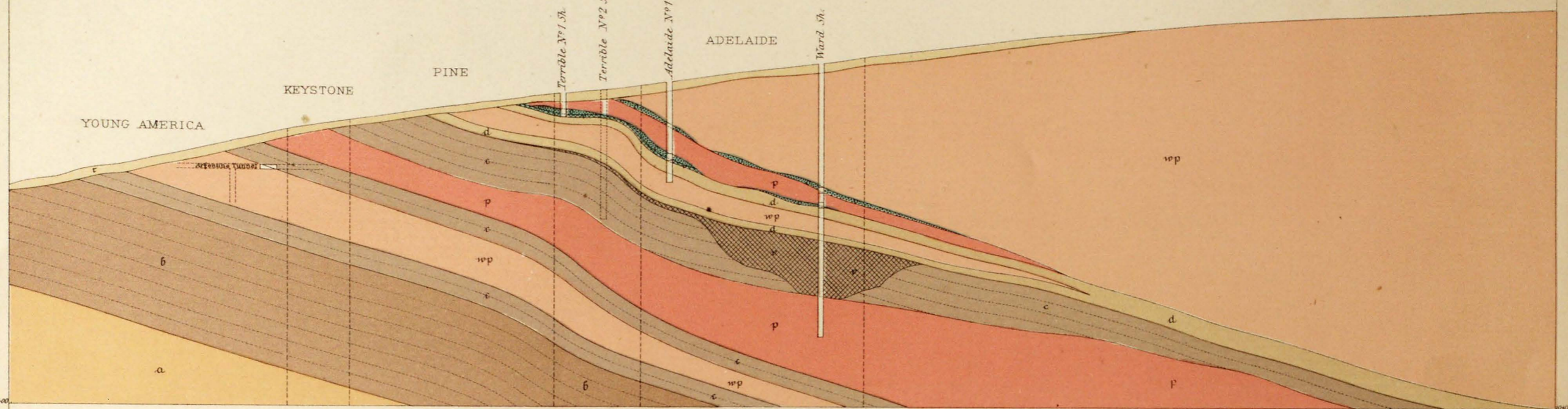
Section BB On Pine-Campbird Line
