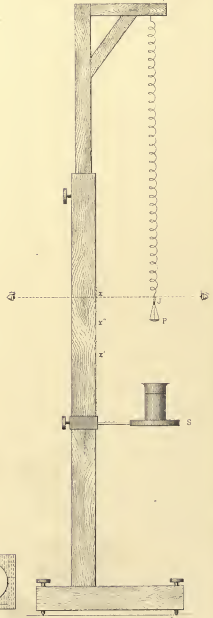
Fig 2 JOLLY'S SPECIFIC GRAVITY SPRING BALANCE Scale: 1 1/2 ft - 1in
