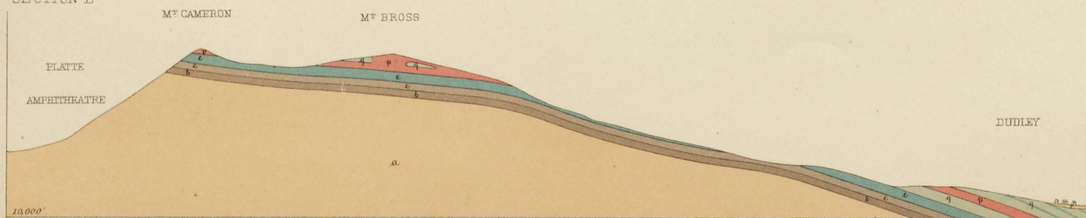
SECTION L
