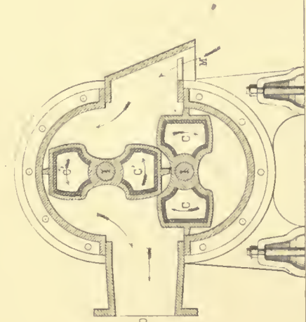
Fig. 4 SECTION Scale \frac{1}{2} in.
