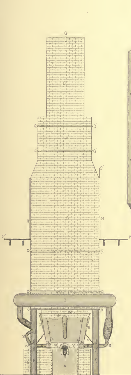
Fig. 1 ELEVATION FURNACE SMELTER F
