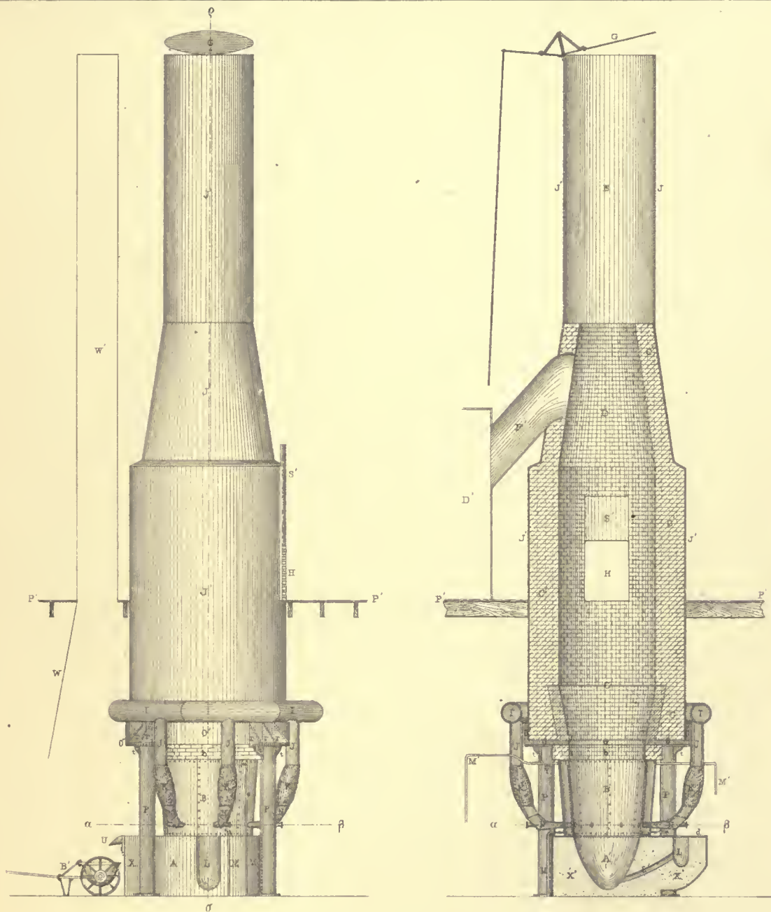
Fig 1 ELEVATION
