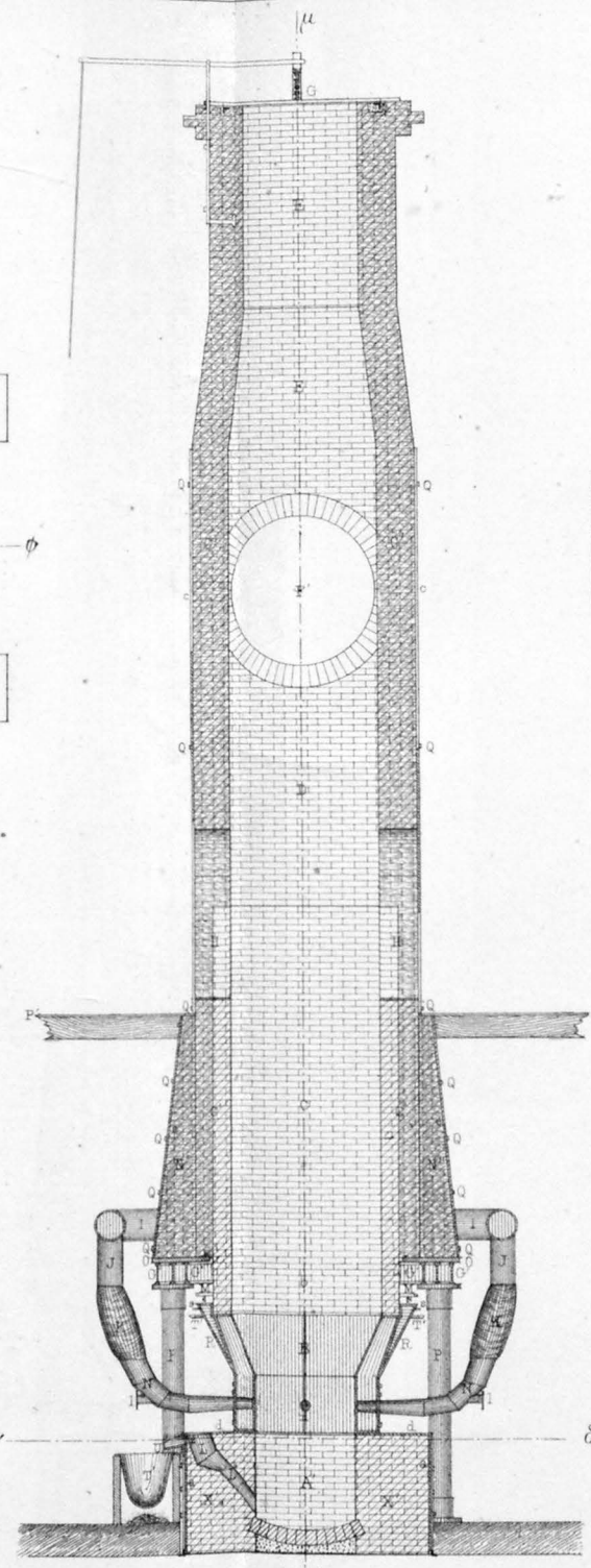
Fig. 3 SECTION ON \gamma\delta
