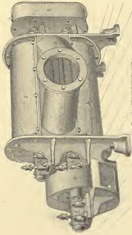
Fig. 3 PERSPECTIVE VIEW
