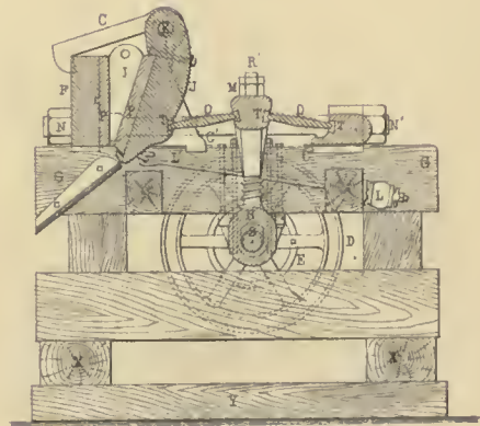
Fig. 4, VERTICAL SECTION
