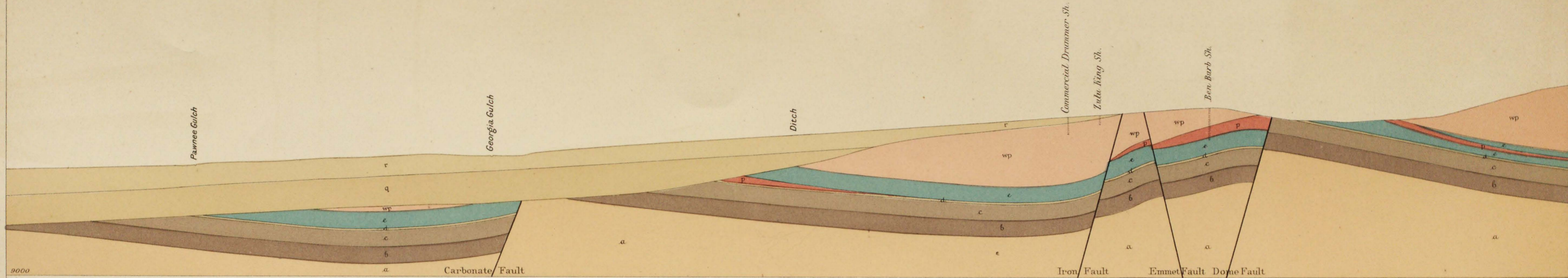
SECTION H H
