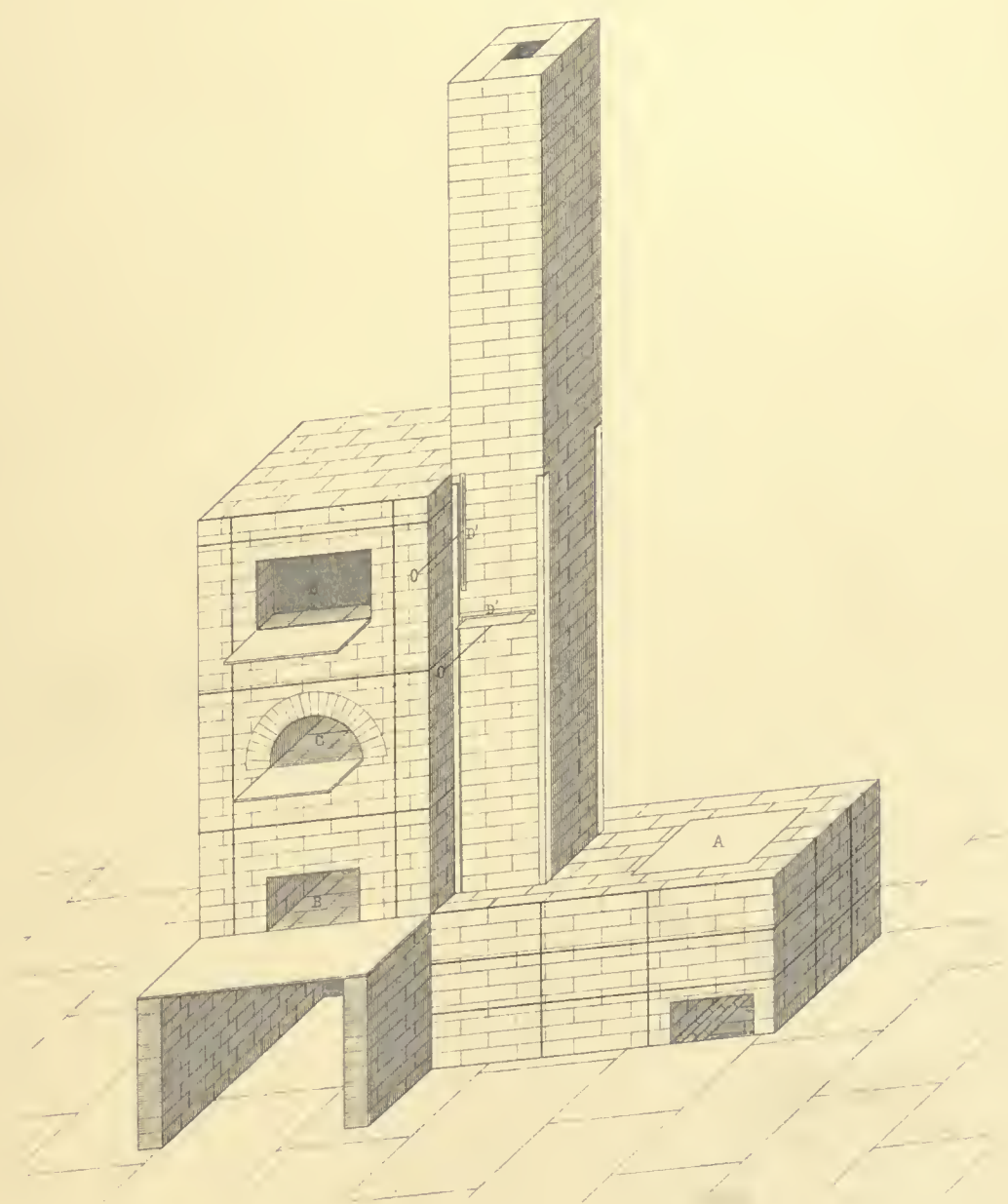
ISOMETRIC PROJECTION
