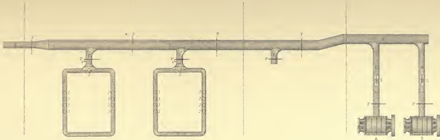
Fig. 1, BLAST ARRANGEMENT
