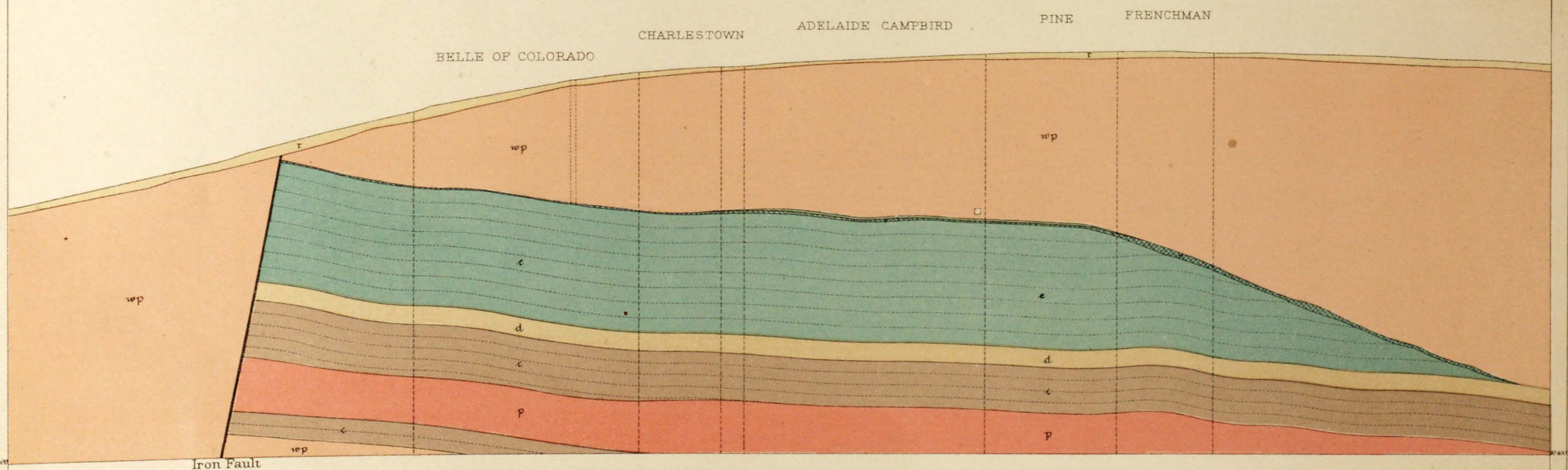
Section CC Across North Iron Hill
