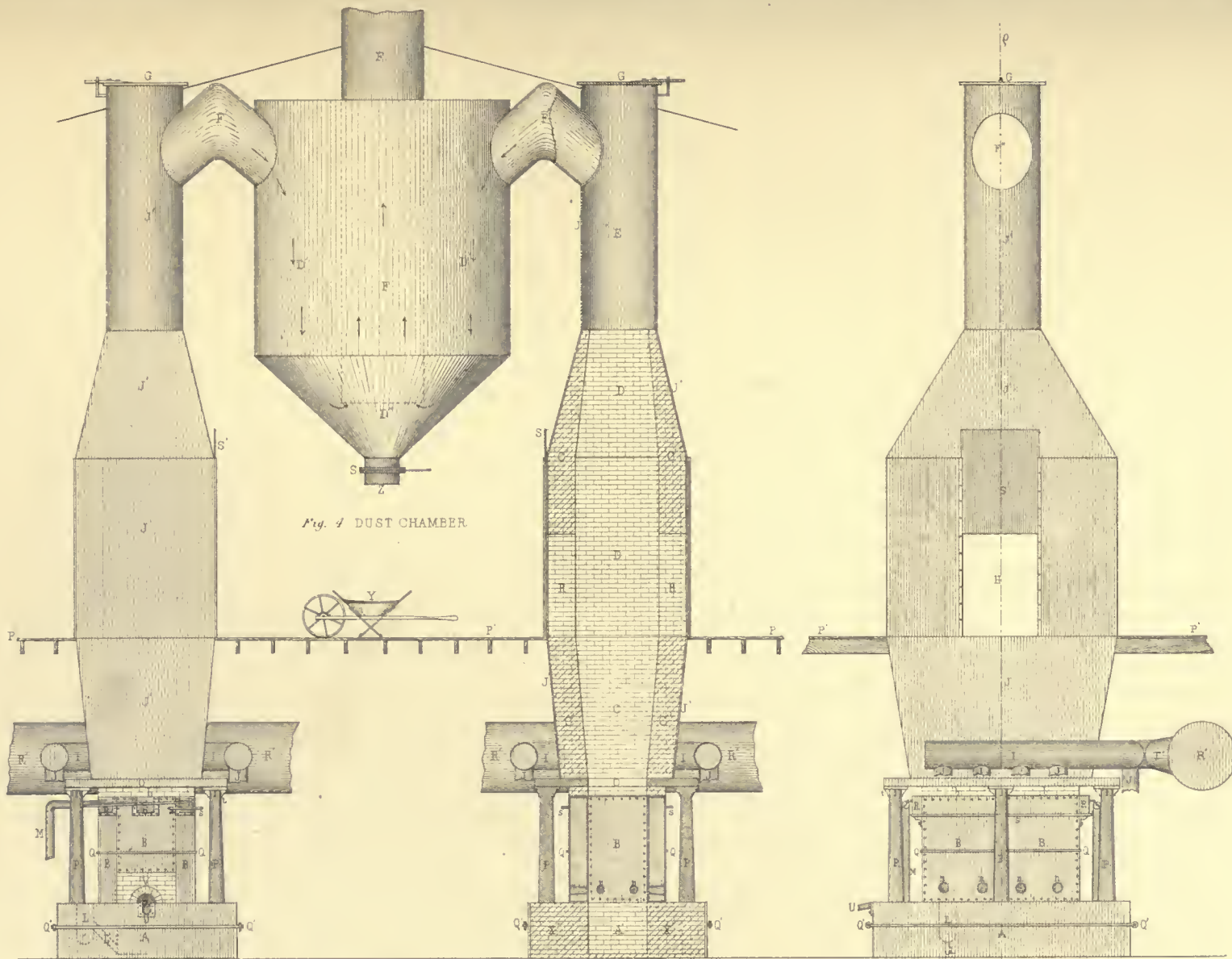
Fig 1 FRONT ELEVATION
