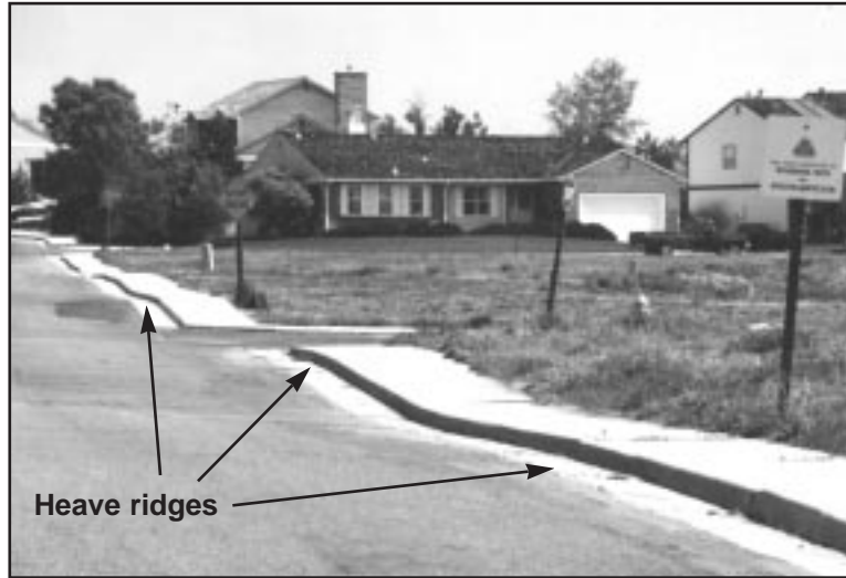
Road damage from heaving bedrock in Morrison
