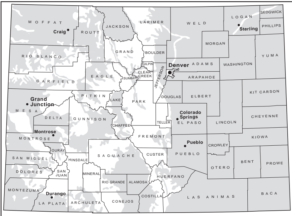
Distribution of swelling soils and bedrock (shaded areas) in Colorado
