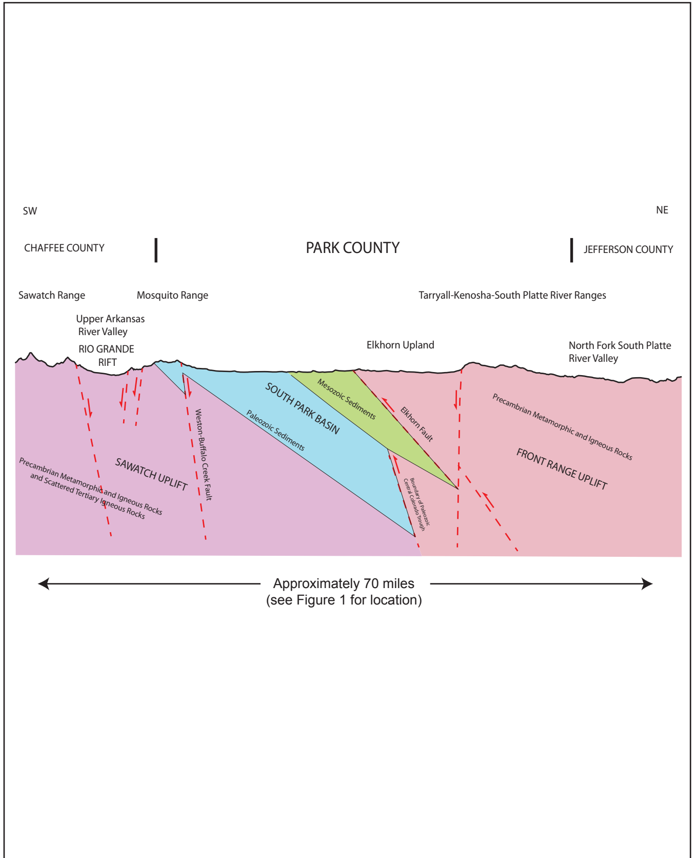
Figure 3. Structural Setting of Park County. Park County straddles three major structural blocks. Laramide uplifts that expose cores of Precambrian crystalline bedrock bound a basin that preserves Cambrian through Paleocene sedimentary strata. The younger Rio Grande rift system cuts through the Sawatch uplift west of the county, forming the Upper Arkansas Valley in Chaffee and Lake Counties.
